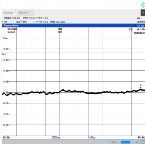
NTNV_N77-3450- 3550_PC2_30_20_H_TID3_NS_01_26000_40000_#1
