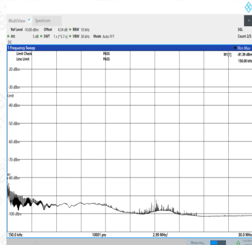
NTNV_N77-3450- 3550_PC2_30_60_M_TID3_NS_01_0.15_30_#1
