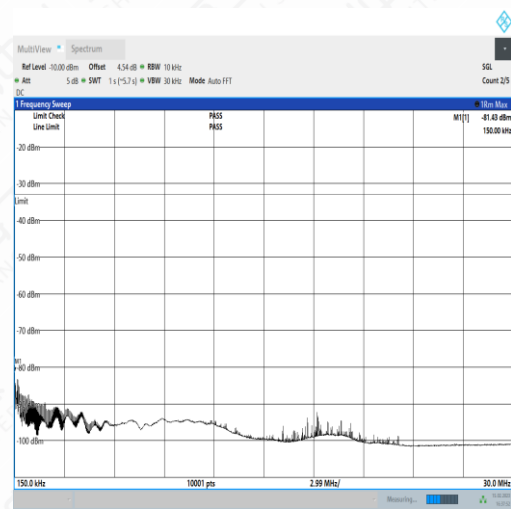
NTNV_N77-3450- 3550_PC2_30_60_L_TID1_NS_01_0.15_30_#1
