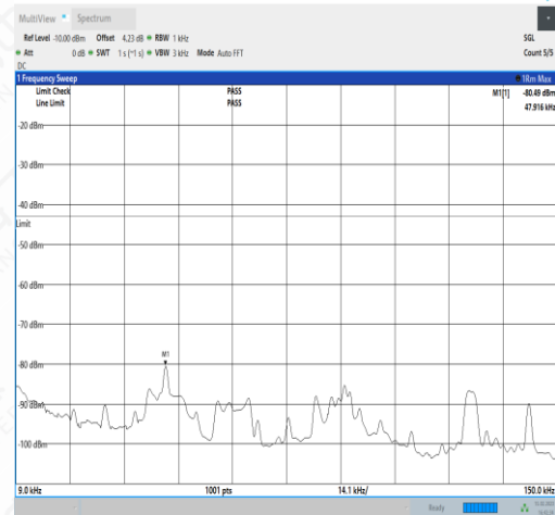
NTNV_N77-3450- 3550_PC2_30_60_L_TID4_NS_01_0.009_0.15_#1
