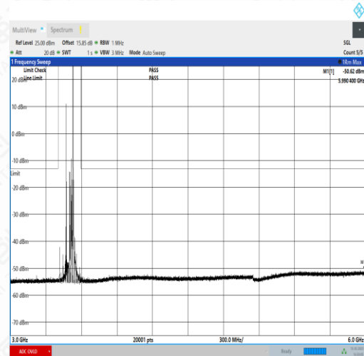
NTNV_N77-3450- 3550_PC2_30_60_M_TID4_NS_01_3000_6000_#1
