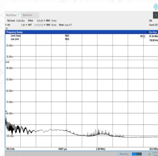
NTNV_N77-3450- 3550_PC2_30_60_H_TID3_NS_01_0.15_30_#1
