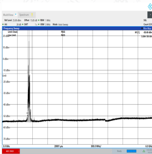
NTNV_N77-3450- 3550_PC2_30_20_H_TID3_NS_01_3000_6000_#1
