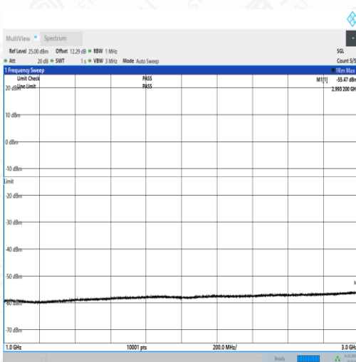
NTNV_N77-3450- 3550_PC2_30_20_M_TID2_NS_01_0.15_30_#1
