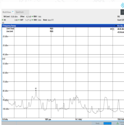
NTNV_N77-3450- 3550_PC2_30_60_H_TID3_NS_01_0.009_0.15_#1
