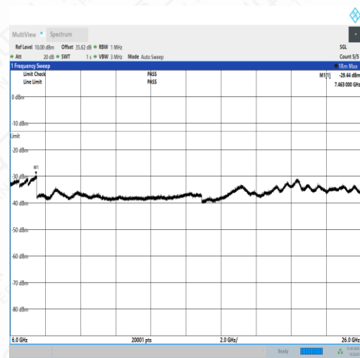
NTNV_N77-3450- 3550_PC2_30_60_H_TID1_NS_01_6000_26000_#1
