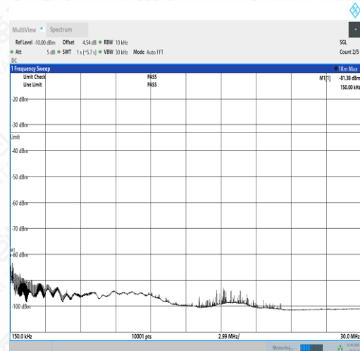
NTNV_N77-3450- 3550_PC2_30_20_H_TID1_NS_01_0.15_30_#1
