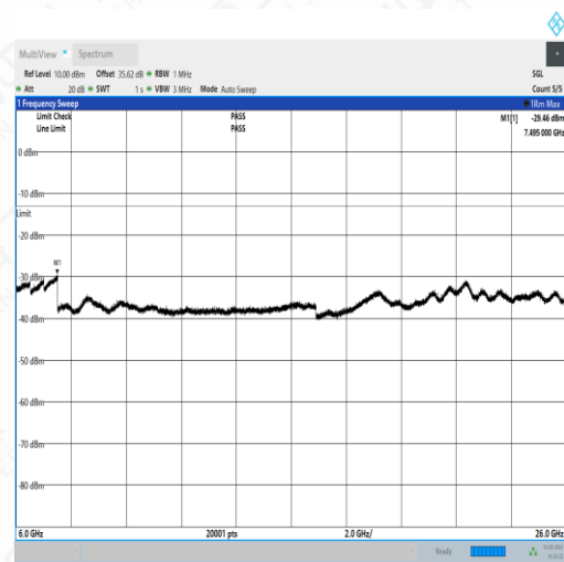
NTNV_N77-3450- 3550_PC2_30_20_H_TID3_NS_01_6000_26000_#1
