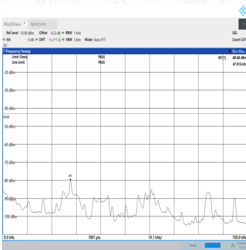
NTNV_N77-3450- 3550_PC2_30_60_L_TID1_NS_01_0.009_0.15_#1
