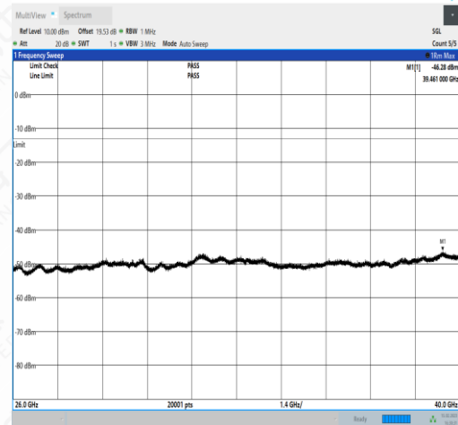
NTNV_N77-3450- 3550_PC2_30_20_M_TID4_NS_01_26000_40000_#1
