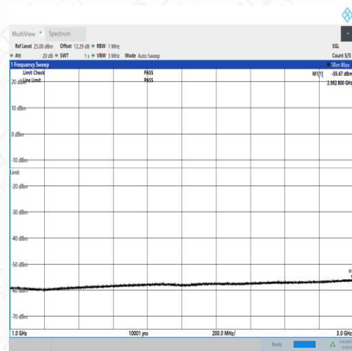
NTNV_N77-3450- 3550_PC2_30_20_M_TID3_NS_01_1000_3000_#1
