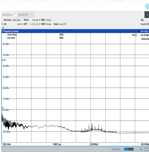
NTNV_N77-3450- 3550_PC2_30_20_H_TID2_NS_01_0.15_30_#1
