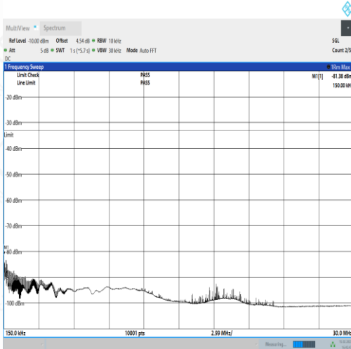
NTNV_N77-3450- 3550_PC2_30_60_L_TID4_NS_01_0.15_30_#1
