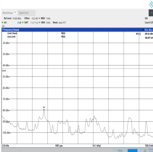
NTNV_N77-3450- 3550_PC2_30_20_H_TID1_NS_01_0.009_0.15_#1
