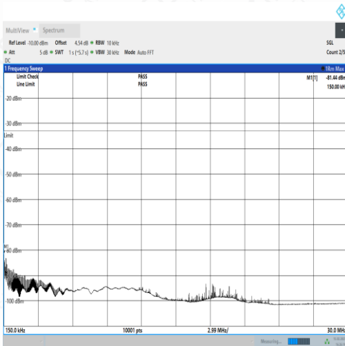
NTNV_N77-3450- 3550_PC2_30_20_M_TID2_NS_01_0.15_30_#1
