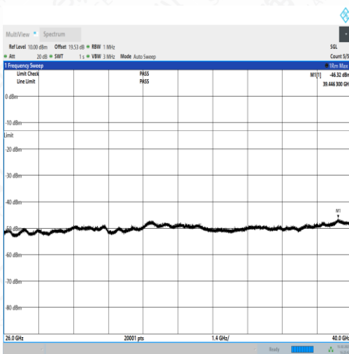
NTNV_N77-3450- 3550_PC2_30_20_M_TID1_NS_01_26000_40000_#1
