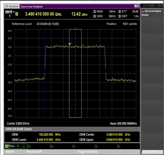
NTNV_N78-3450-3550_PC2_30_100_M_TID3_Ant1#1
