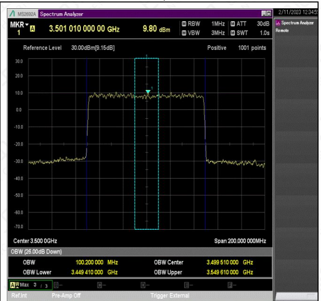
NTNV_N78-3450-3550_PC2_30_100_M_TID5_Ant1#1
