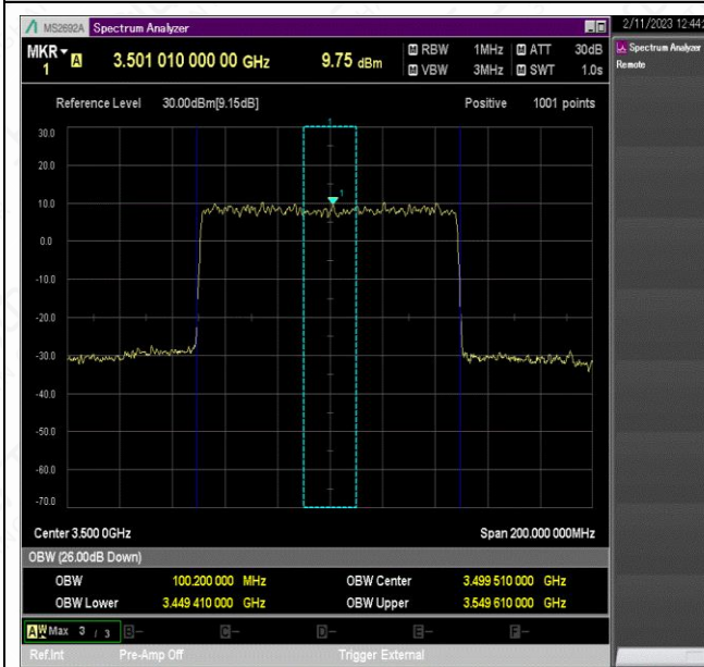
NTNV_N78-3450-3550_PC2_30_100_H_TID5_Ant1#1
