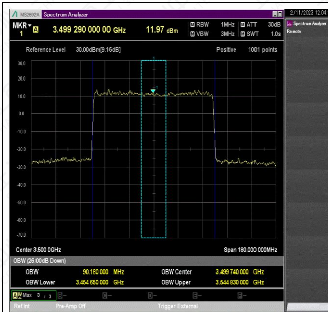
NTNV_N78-3450-3550_PC2_30_90_M_TID3_Ant1#1
