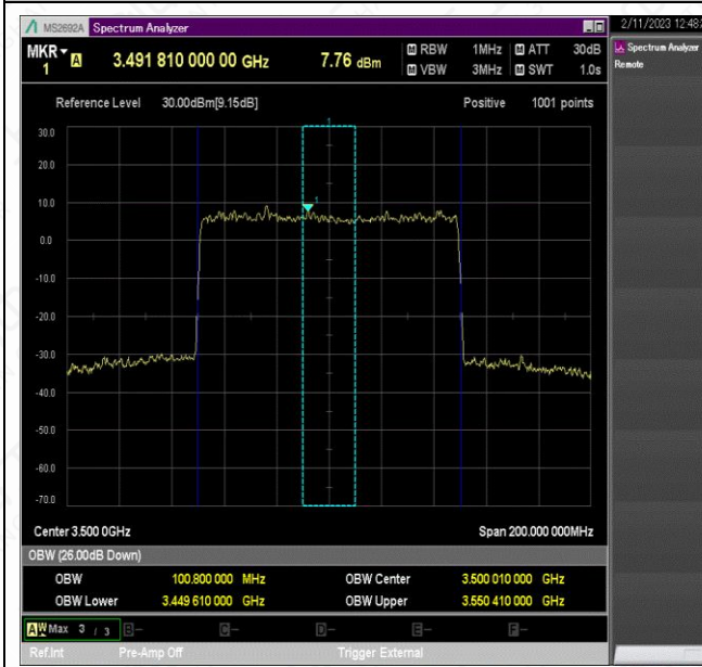
NTNV_N78-3450-3550_PC2_30_100_H_TID9_Ant1#1
