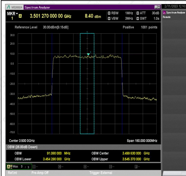
NTNV_N78-3450-3550_PC2_30_90_M_TID9_Ant1#1
