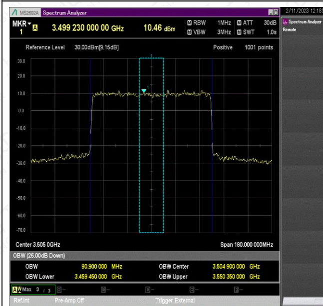
NTNV_N78-3450-3550_PC2_30_90_H_TID8_Ant1#1
