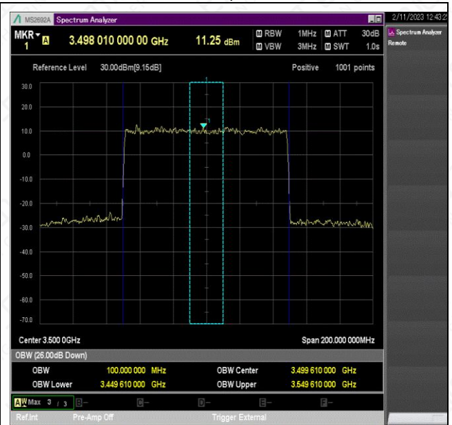
NTNV_N78-3450-3550_PC2_30_100_H_TID4_Ant1#1
