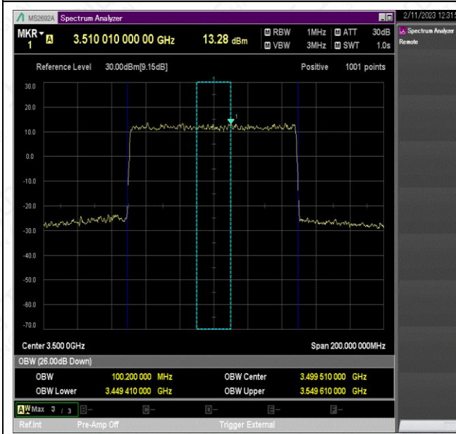
NTNV_N78-3450-3550_PC2_30_100_M_TID2_Ant1#1
