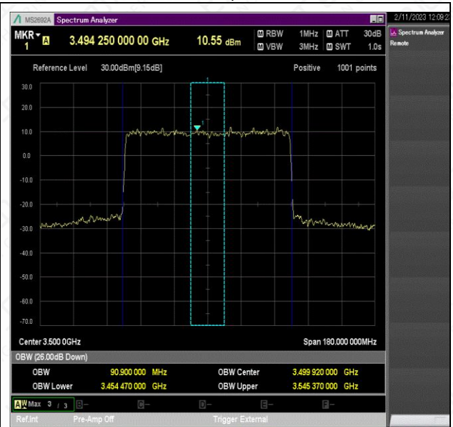
NTNV_N78-3450-3550_PC2_30_90_M_TID8_Ant1#1
