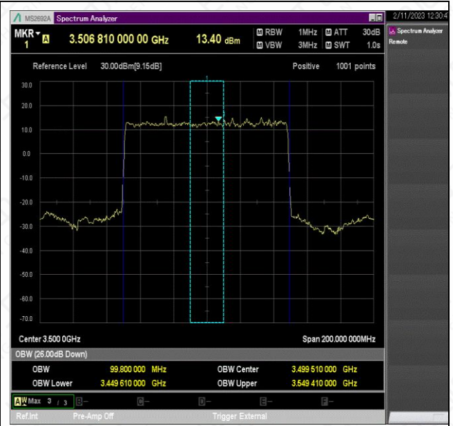
NTNV_N78-3450-3550_PC2_30_100_M_TID1_Ant1#1
