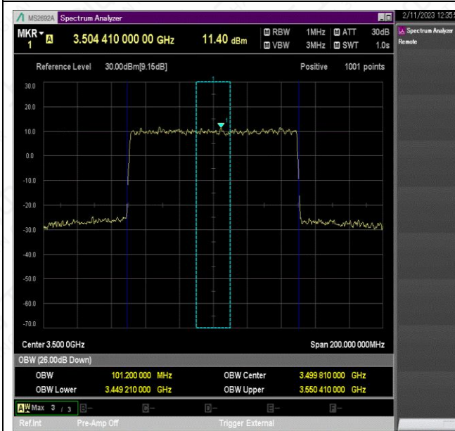
NTNV_N78-3450-3550_PC2_30_100_M_TID6_Ant1#1
