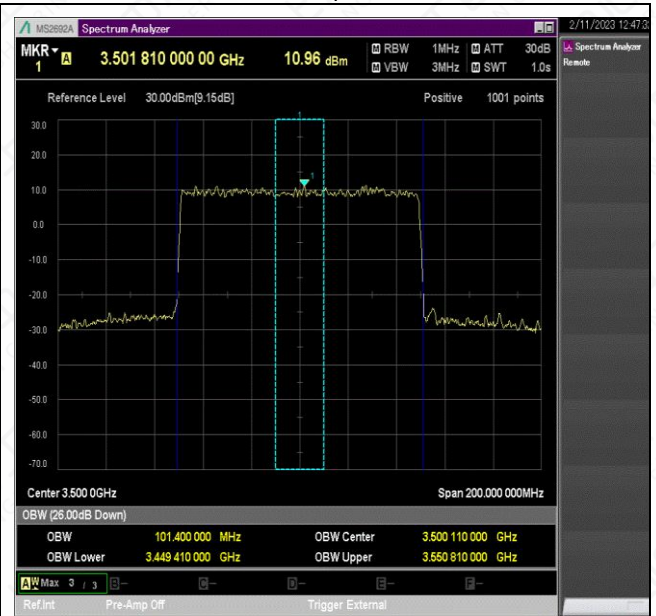
NTNV_N78-3450-3550_PC2_30_100_H_TID8_Ant1#1
