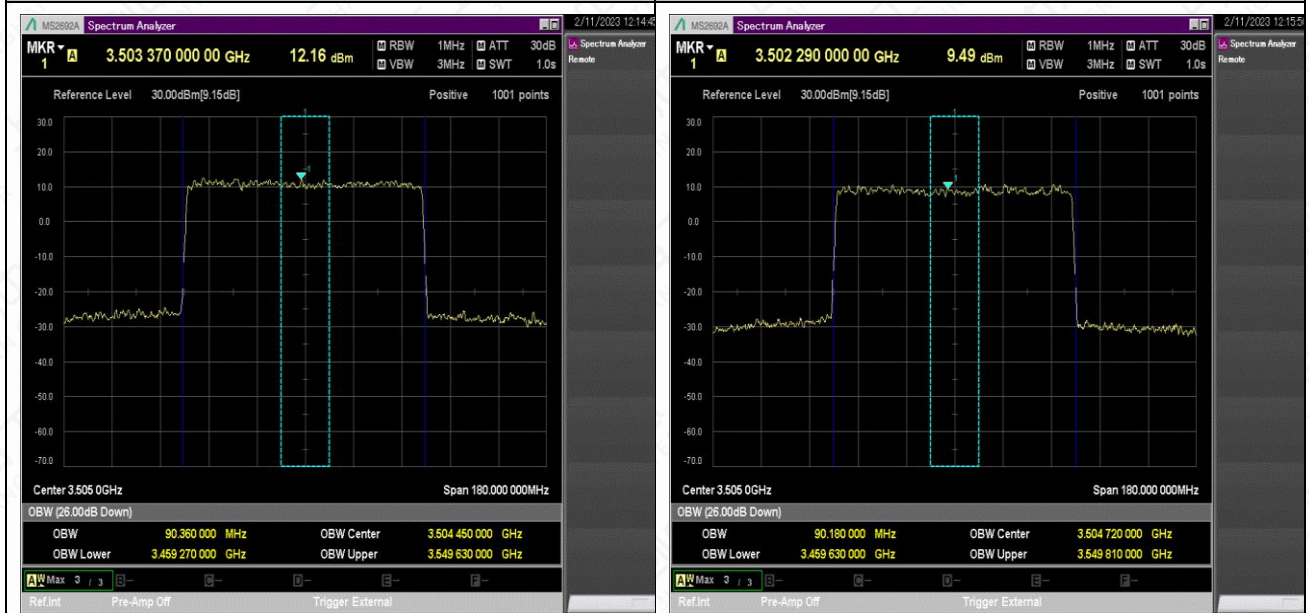
NTNV_N78-3450-3550_PC2_30_90_H_TID4_Ant1#1
