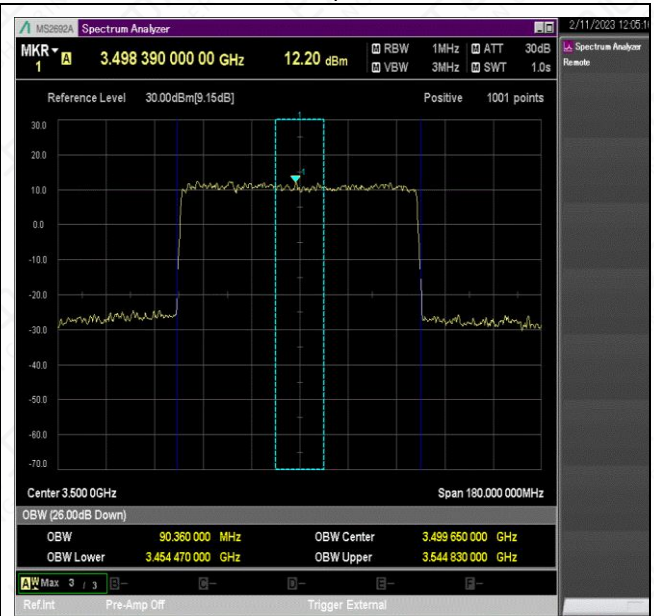
NTNV_N78-3450-3550_PC2_30_90_M_TID4_Ant1#1
