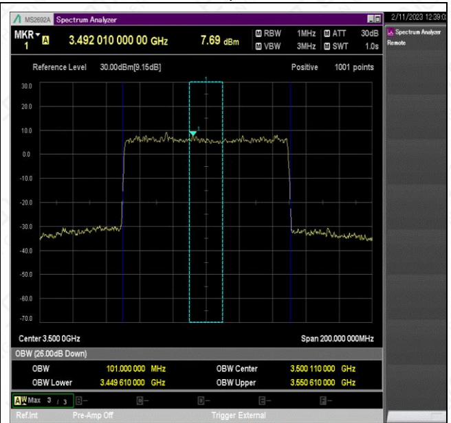
NTNV_N78-3450-3550_PC2_30_100_M_TID9_Ant1#1
