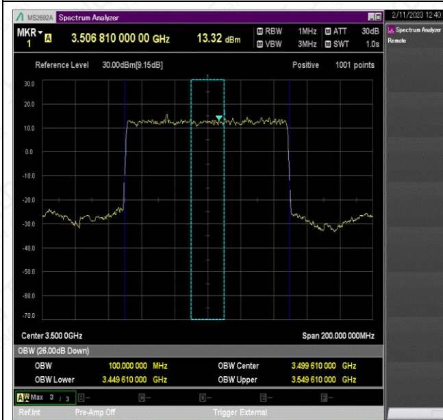
NTNV_N78-3450-3550_PC2_30_100_H_TID1_Ant1#1
