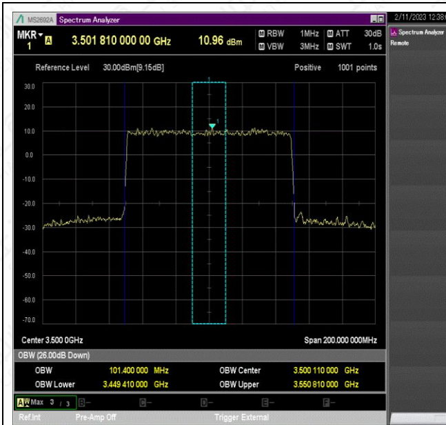
NTNV_N78-3450-3550_PC2_30_100_M_TID8_Ant1#1
