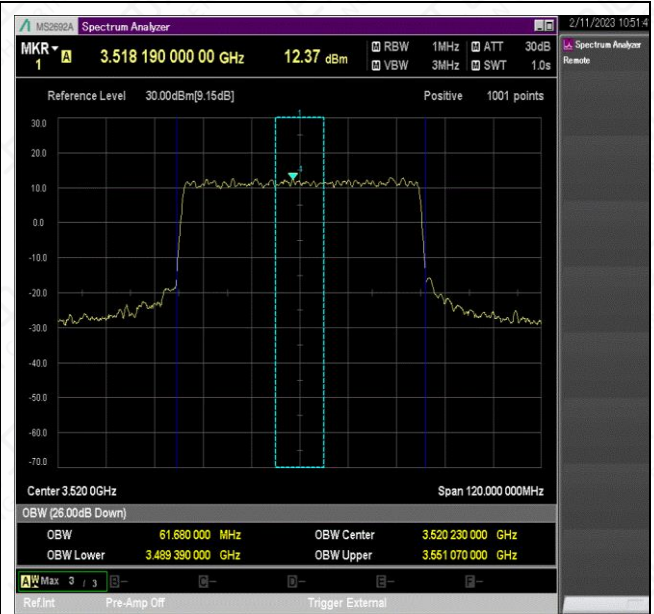
NTNV_N78-3450-3550_PC2_30_60_H_TID8_Ant1#1
