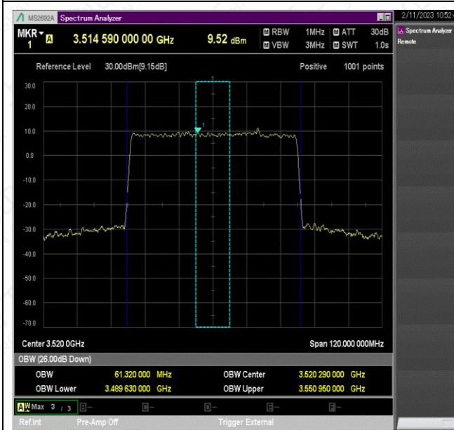
NTNV_N78-3450-3550_PC2_30_60_H_TID9_Ant1#1
