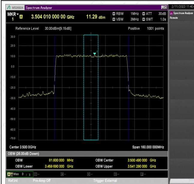
NTV_N78-3450-3550_PC2_30_80_M_TID8_Ant1#1
