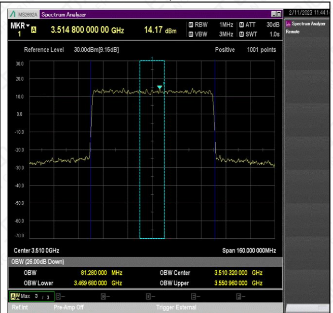
NTV_N78-3450-3550_PC2_30_80_H_TID2_Ant1#1
