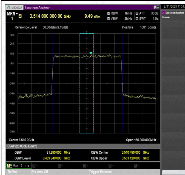
NTNV_N78-3450-3550_PC2_30_80_H_TID9_Ant1#1
