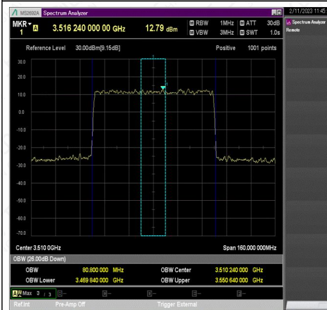
NTV_N78-3450-3550_PC2_30_80_H_TID3_Ant1#1
