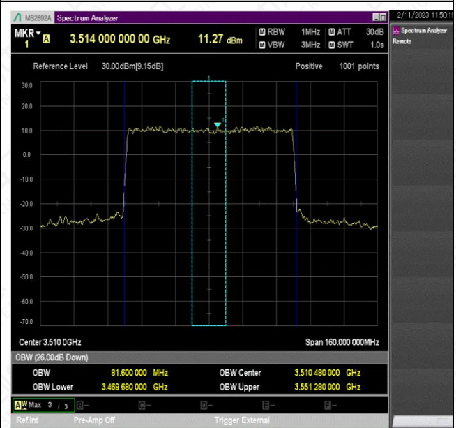
NTNV_N78-3450-3550_PC2_30_80_H_TID8_Ant1#1
