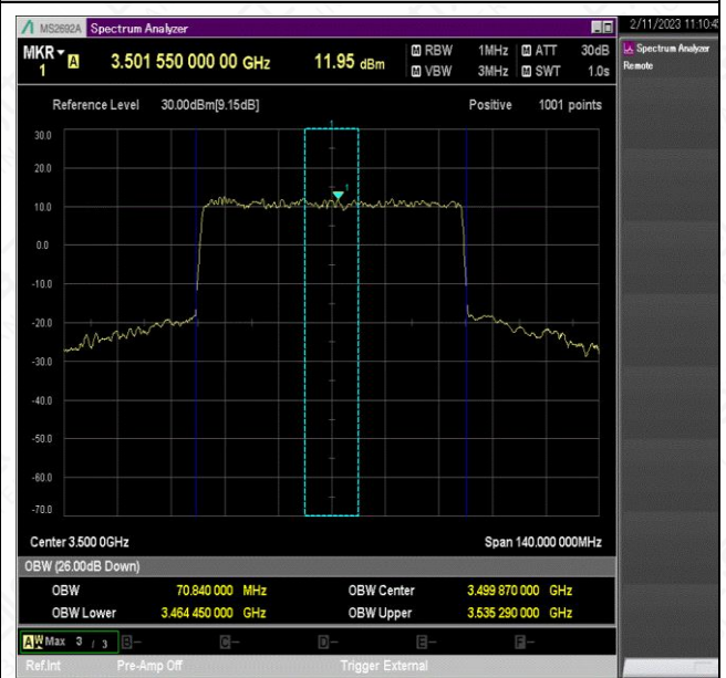
NTV_N78-3450-3550_PC2_30_70_M_TID8_Ant1#1
