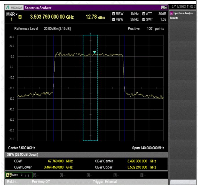
NTNV_N78-3450-3550_PC2_30_70_M_TID4_Ant1#1
