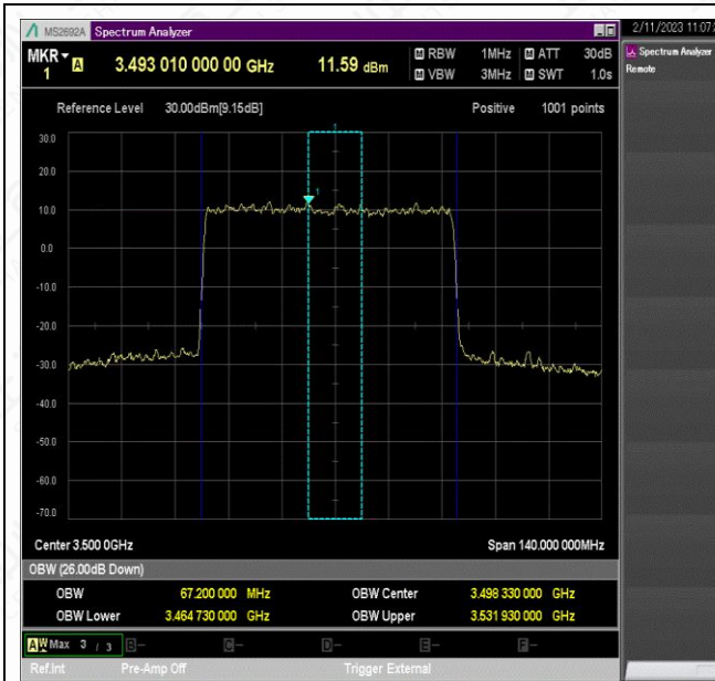
NTV_N78-3450-3550_PC2_30_70_M_TID5_Ant1#1
