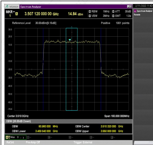
NTV_N78-3450-3550_PC2_30_80_H_TID1_Ant1#1
