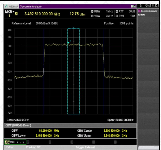
NTV_N78-3450-3550_PC2_30_80_M_TID3_Ant1#1
