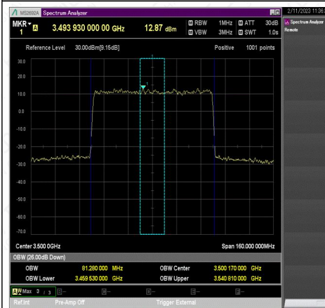
NTV_N78-3450-3550_PC2_30_80_M_TID4_Ant1#1
