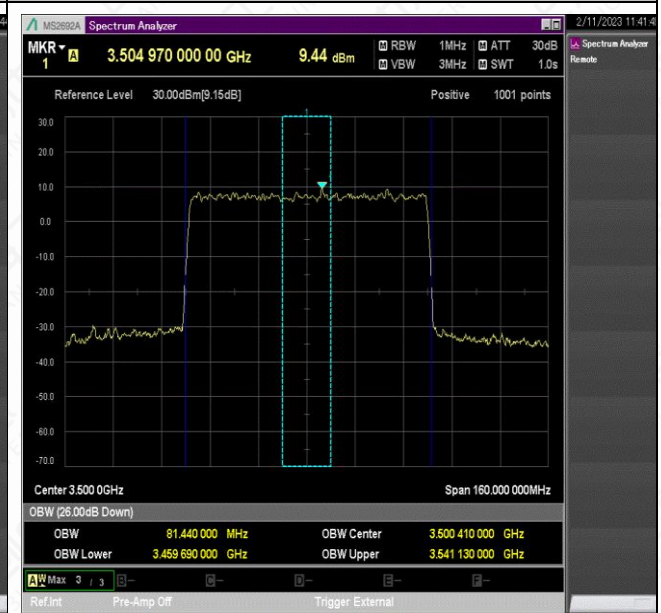
NTV_N78-3450-3550_PC2_30_80_M_TID9_Ant1#1
