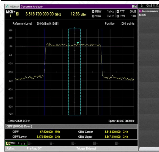
NTNV_N78-3450-3550_PC2_30_70_H_TID4_Ant1#1
