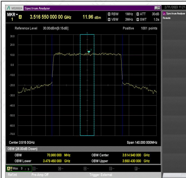
NTNV_N78-3450-3550_PC2_30_70_H_TID8_Ant1#1
