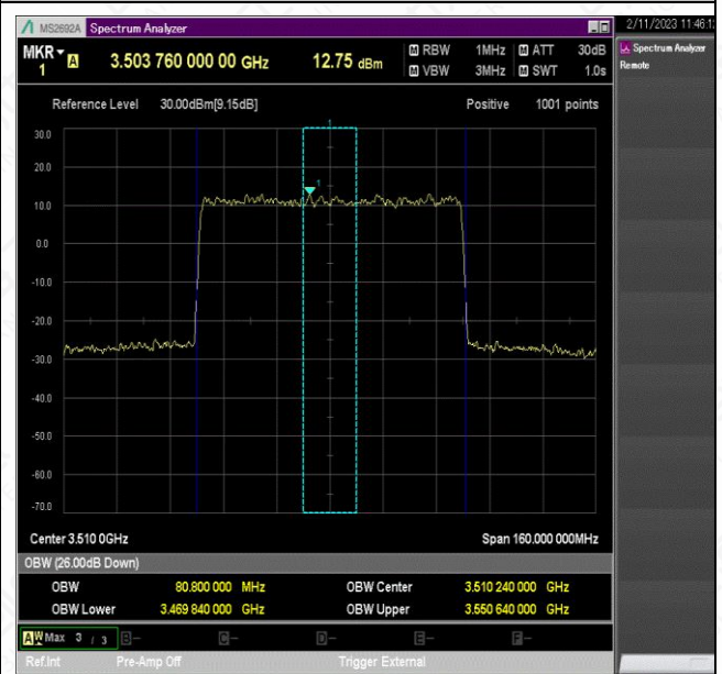
NTV_N78-3450-3550_PC2_30_80_H_TID4_Ant1#1
