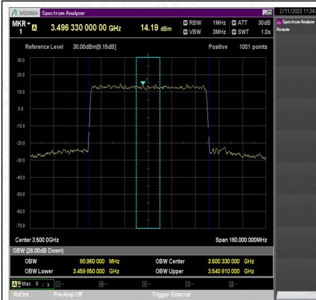
NTV_N78-3450-3550_PC2_30_80_M_TID2_Ant1#1
