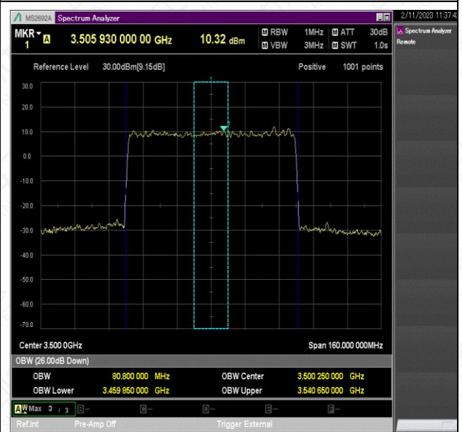
NTV_N78-3450-3550_PC2_30_80_M_TID5_Ant1#1
