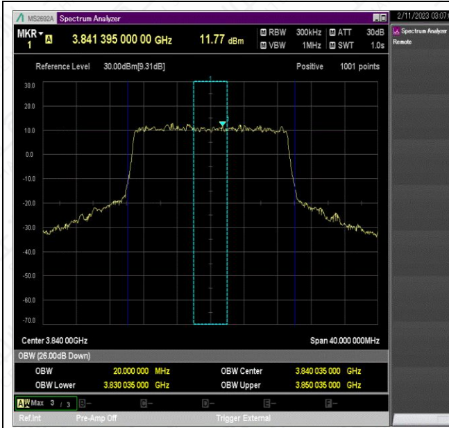
NTNV_N77-3700-3980_PC2_30_20_M_TID8_Ant1#1
