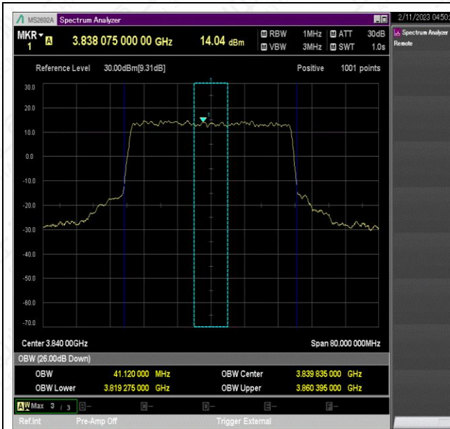
NTNV_N77-3700-3980_PC2_30_40_M_TID8_Ant1#1
