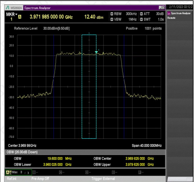
NTNV_N77-3700-3980_PC2_30_20_H_TID4_Ant1#1
