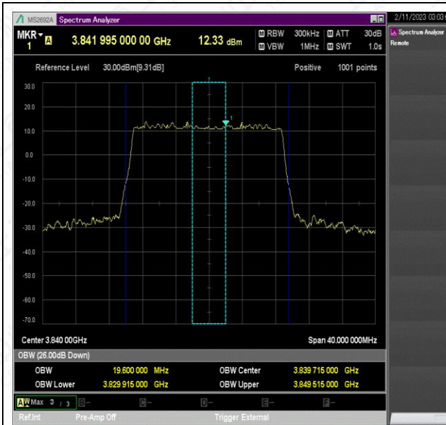
NTNV_N77-3700-3980_PC2_30_20_M_TID4_Ant1#1
