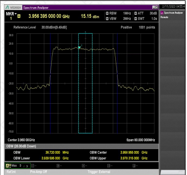
NTNV_N77-3700-3980_PC2_30_40_H_TID4_Ant1#1
