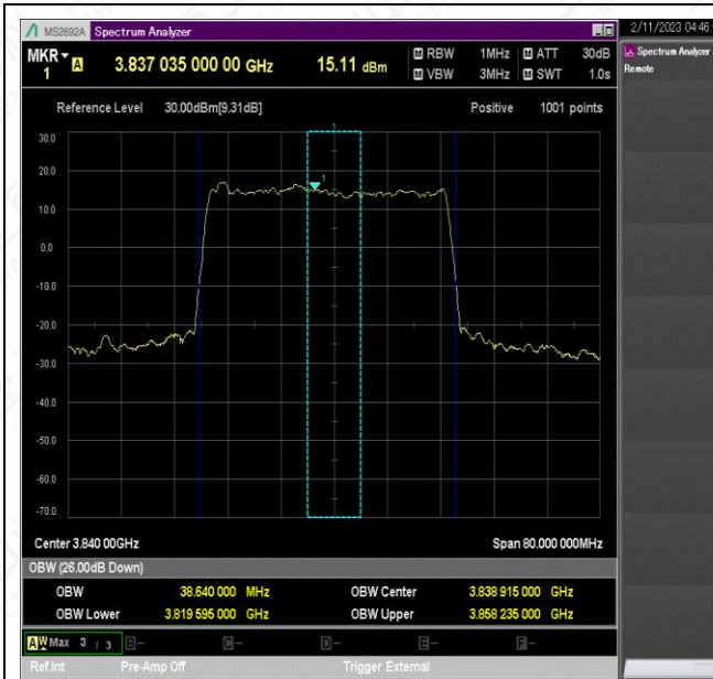
NTNV_N77-3700-3980_PC2_30_40_M_TID4_Ant1#1
