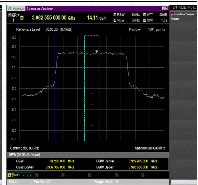
NTNV_N77-3700-3980_PC2_30_40_H_TID8_Ant1#1
