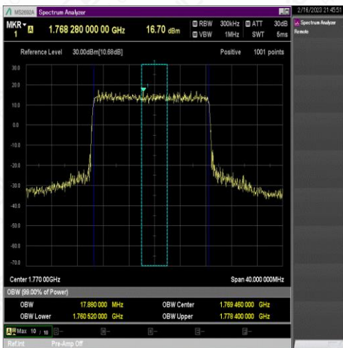
NTNV_N66_PC3_15_20_M_TID9_Ant1#1
