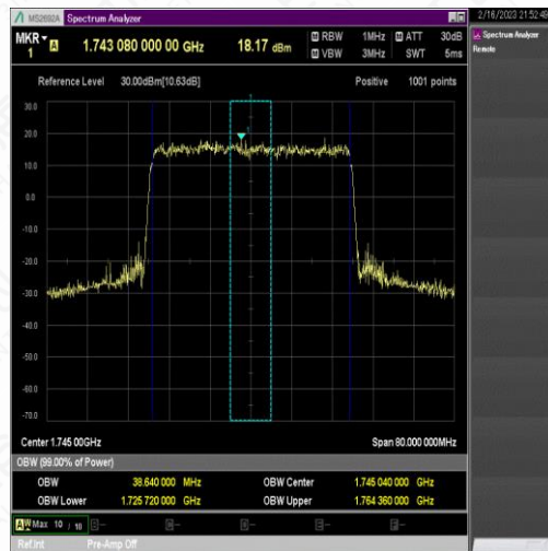
NTNV_N66_PC3_15_40_M_TID4_Ant1#1
