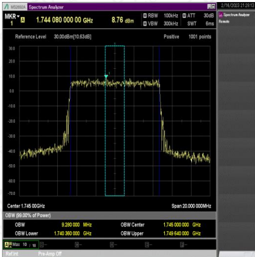
NTNV_N66_PC3_15_10_M_TID9_Ant1#1
