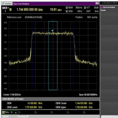
NTNV_N66_PC3_15_15_M_TID6_Ant1#1
