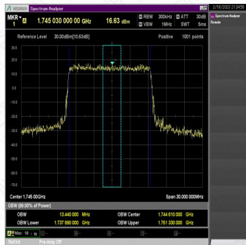
NTNV_N66_PC3_15_15_M_TID1_Ant1#1
