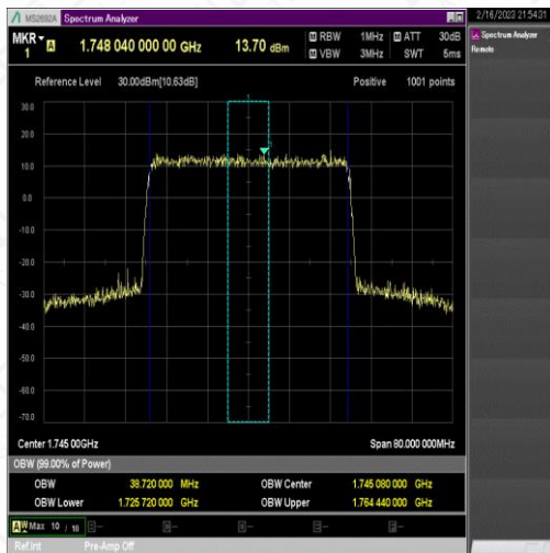
NTNV_N66_PC3_15_40_M_TID9_Ant1#1
