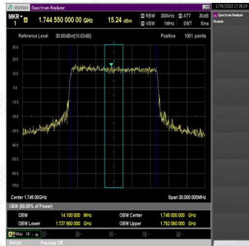
NTNV_N66_PC3_15_15_M_TID7_Ant1#1
