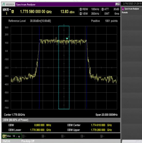
NTNV_N66_PC3_15_10_M_TID9_Ant1#1
