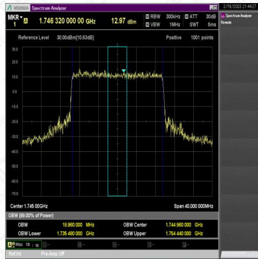
NTNV_N66_PC3_15_20_M_TID8_Ant1#1
