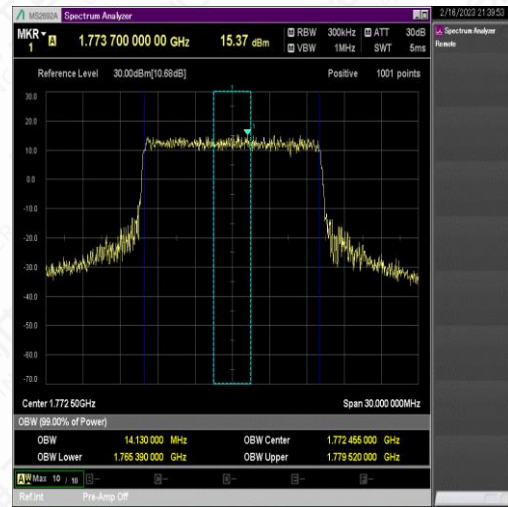
NTNV_N66_PC3_15_15_H_TID8_Ant1#1
