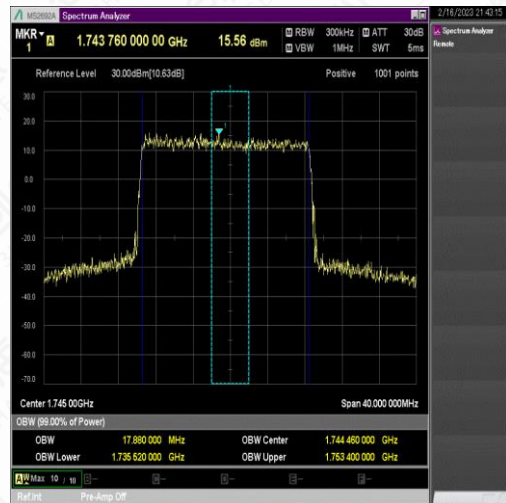
NTNV_N66_PC3_15_20_M_TID4_Ant1#1
