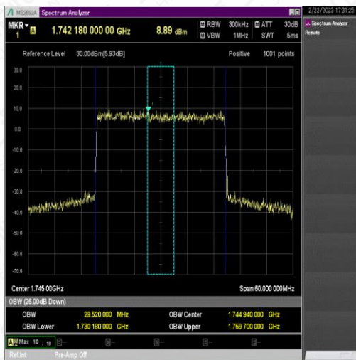
NTNV_N66_PC3_15_30_M_TID4_Ant1#1
