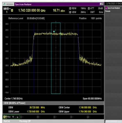
NTNV_N66_PC3_15_40_M_TID8_Ant1#1
