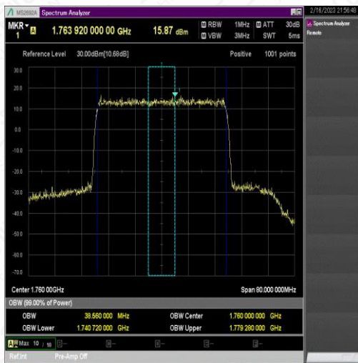
NTNV_N66_PC3_15_40_H_TID5_Ant#1
