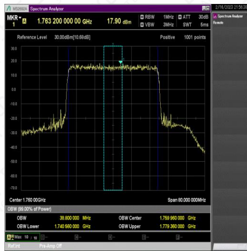
NTNV_N66_PC3_15_40_H_TID4_Ant#1
