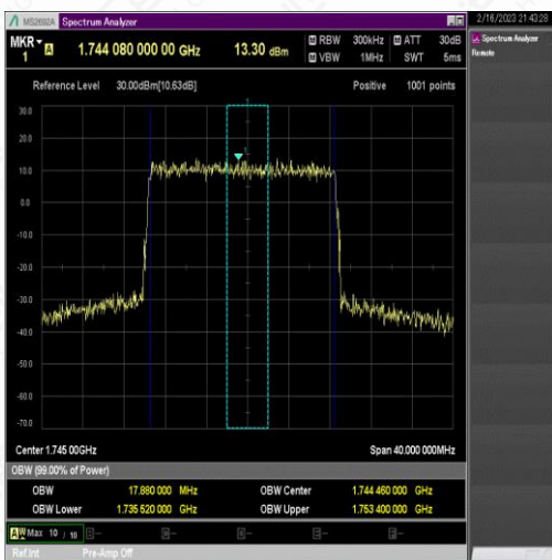
NTNV_N66_PC3_15_20_M_TID3_Ant1#1
