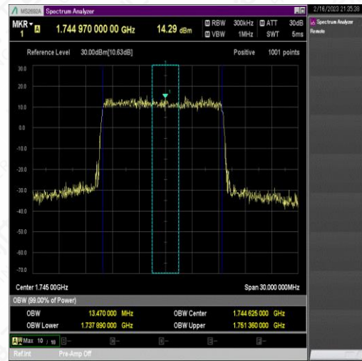
NTNV_N66_PC3_15_15_M_TID5_Ant1#1
