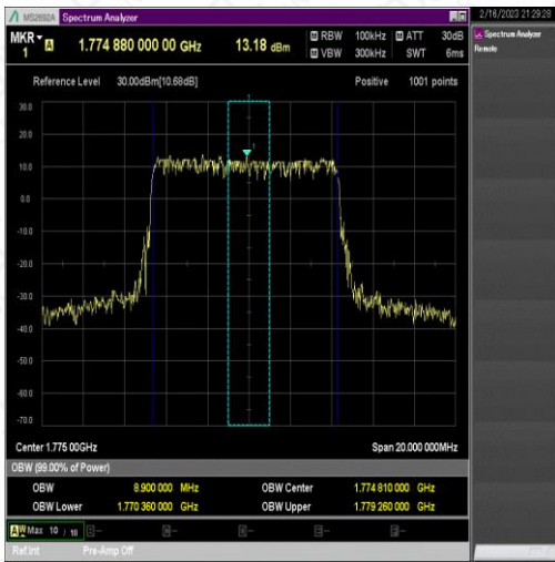
NTNV_N66_PC3_15_10_H_TID4_Ant1#1
