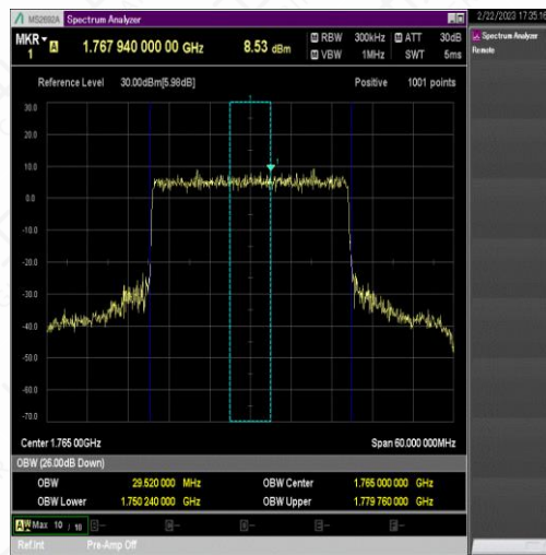
NTNV_N66_PC3_15_30_H_TID8_Ant1#1
