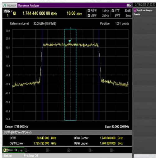
NTNV_N66_PC3_15_40_M_TID5_Ant1#1
