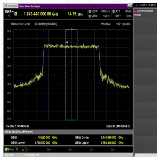
NTNV_N66_PC3_15_20_M_TID4_Ant1#1
