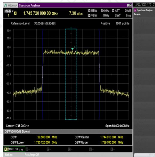
NTNV_N66_PC3_15_30_M_TID5_Ant1#1
