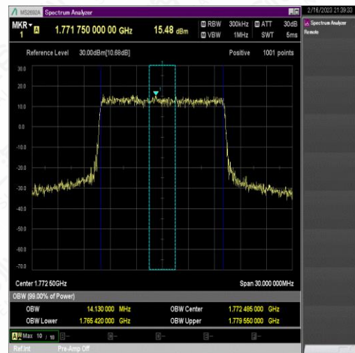
NTNV_N66_PC3_15_15_H_TID4_Ant1#1
