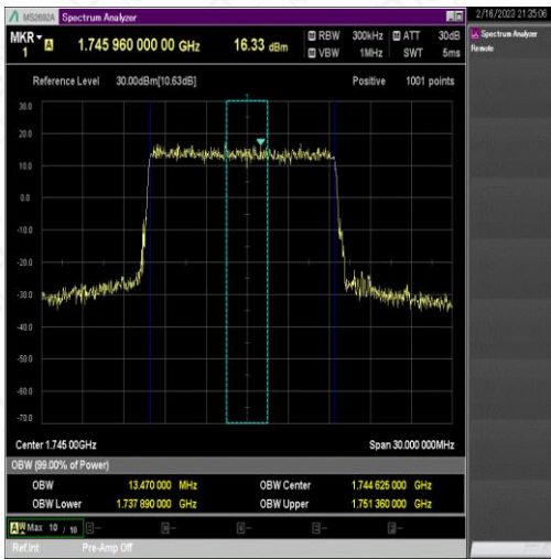
NTNV_N66_PC3_15_15_M_TID4_Ant1#1
