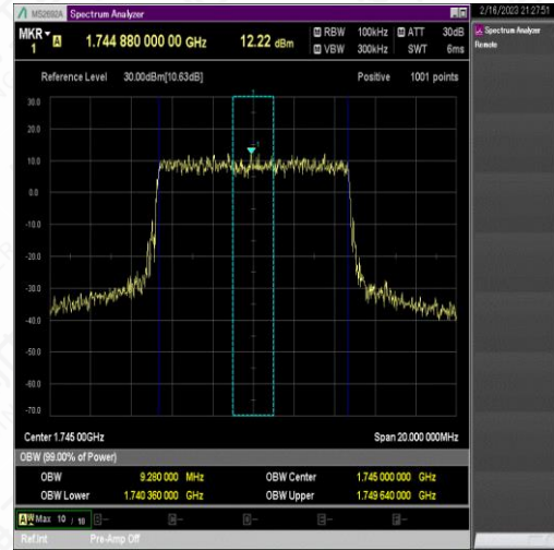
NTNV_N66_PC3_15_10_M_TID8_Ant1#1
