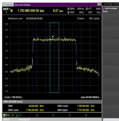
NTNV_N66_PC3_15_30_H_TID4_Ant1#1
