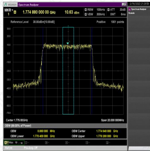
NTNV_N66_PC3_15_10_H_TID5_Ant1#1
