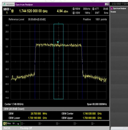
NTNV_N66_PC3_15_30_M_TID9_Ant1#1
