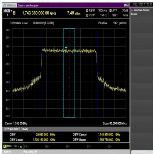
NTNV_N66_PC3_15_30_M_TID8_Ant1#1
