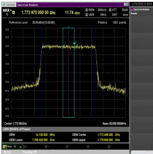
NTNV_N66_PC3_15_15_H_TID9_Ant1#1
