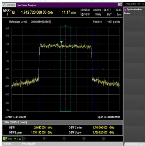
NTNV_N66_PC3_15_30_M_TID2_Ant1#1
