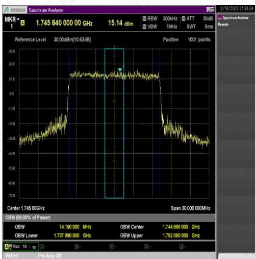
NTNV_N66_PC3_15_15_M_TID6_Ant1#1
