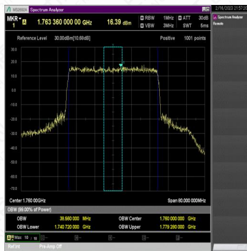
NTNV_N66_PC3_15_40_H_TID8_Ant#1
