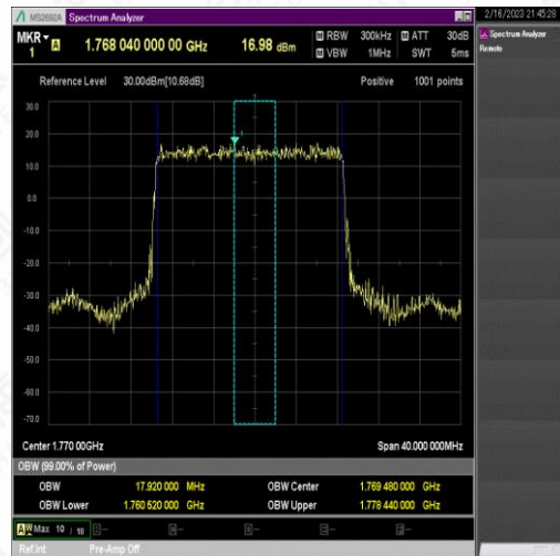
NTNV_N66_PC3_15_20_H_TID1_Ant1#1
