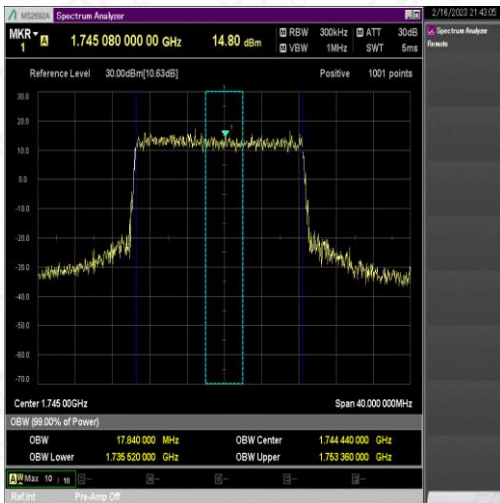
NTNV_N66_PC3_15_20_M_TID3_Ant1#1
