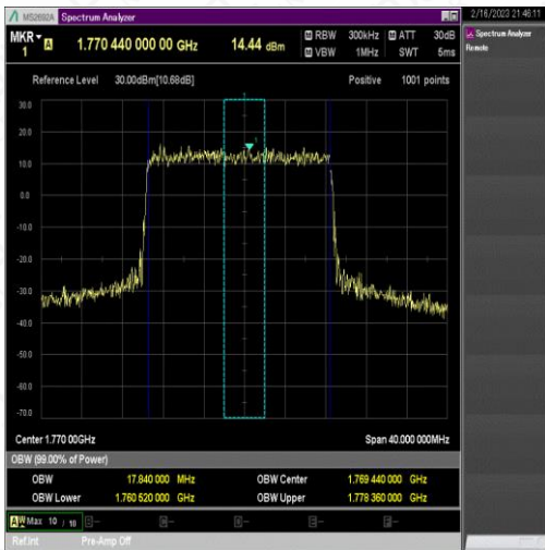
NTNV_N66_PC3_15_20_H_TID4_Ant1#1
