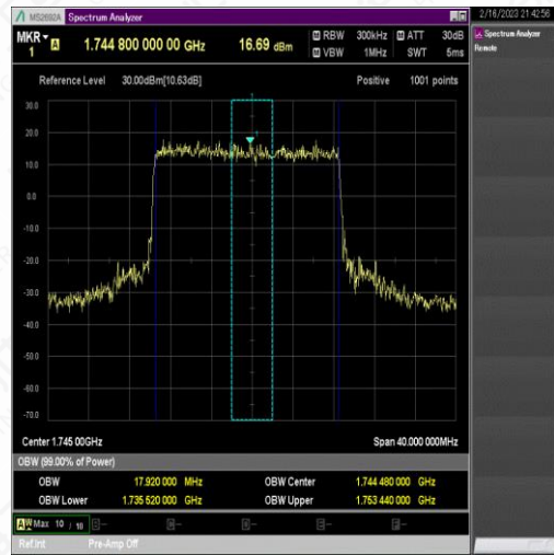
NTNV_N66_PC3_15_20_M_TID2_Ant1#1
