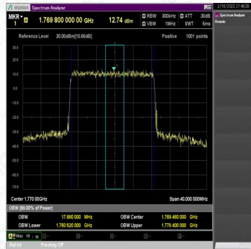
NTNV_N66_PC3_15_20_H_TID5_Ant1#1
