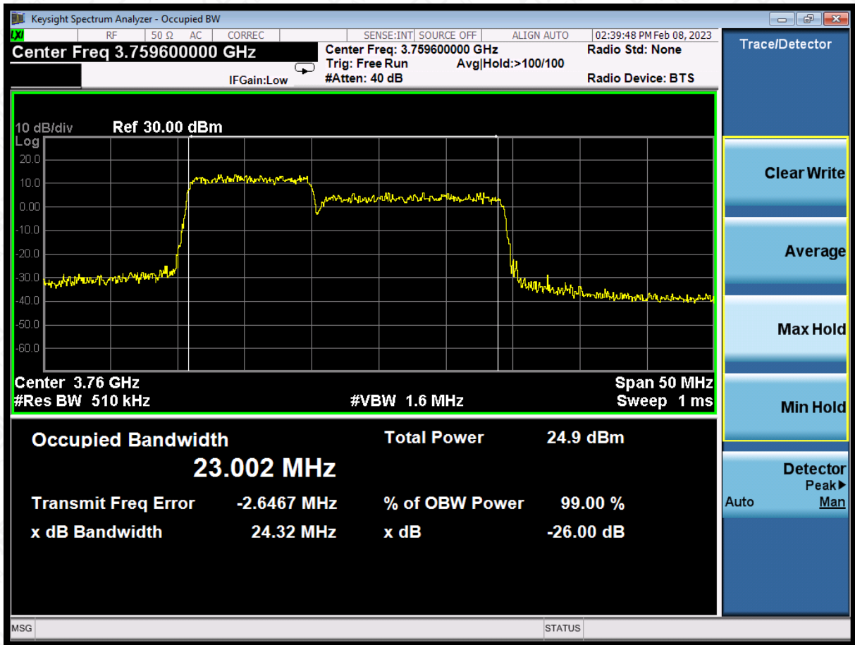
LTE CA band 43Part27 , 10MHz+15MHz Bandwidth,64QAM (-26dBc BW)
