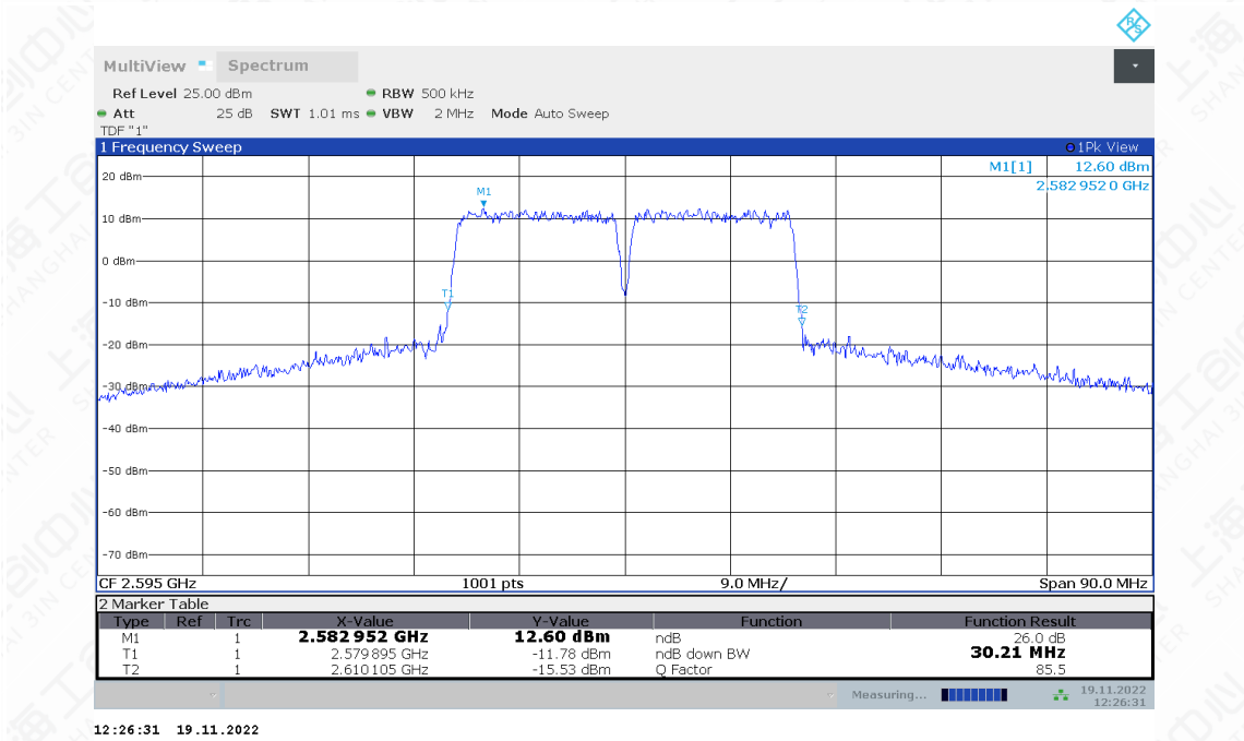
LTE CA band 38 , 15MHz+15MHz Bandwidth,QPSK (-26dBc BW)
