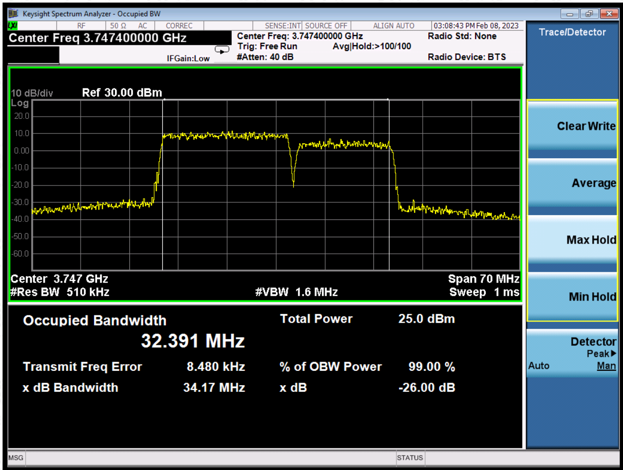
LTE CA band 43Part27 , 20MHz+15MHz Bandwidth,64QAM (-26dBc BW)
