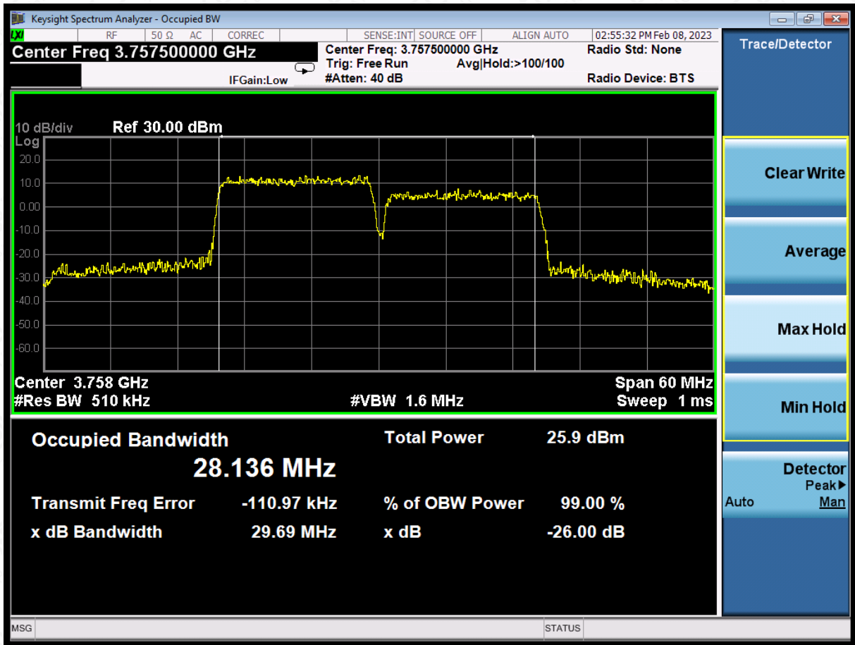
LTE CA band 43Part27 ,15MHz+15MHz Bandwidth,16QAM (-26dBc BW)
