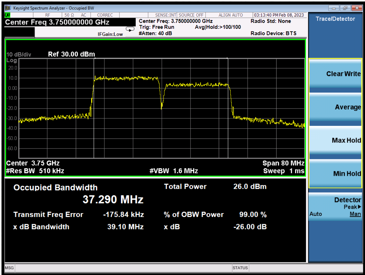
LTE CA band 43Part27 , 20MHz+20MHz Bandwidth,16QAM (-26dBc BW)
