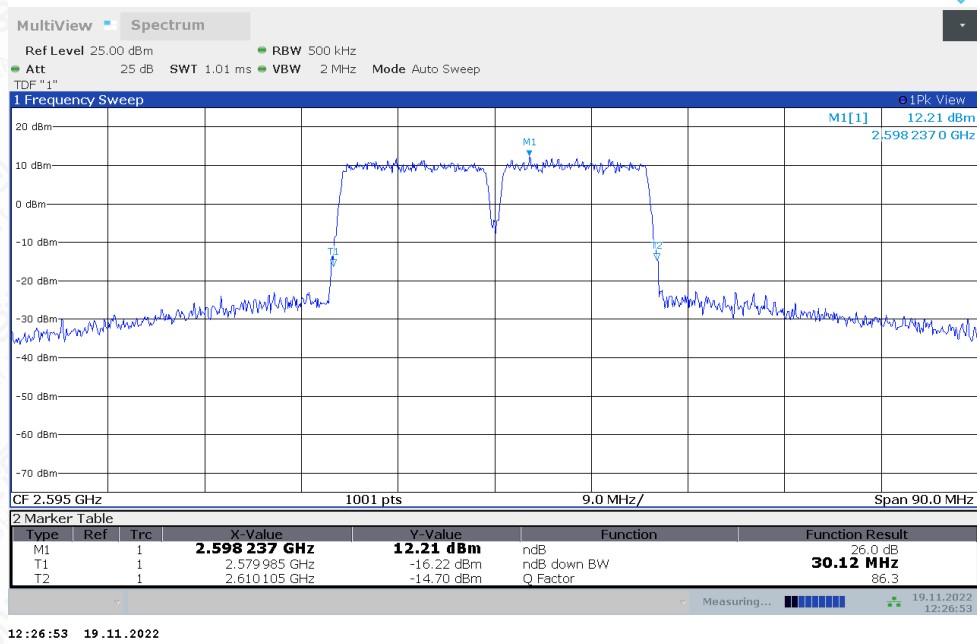
LTE CA band 38 , 15MHz+15MHz Bandwidth,64QAM (-26dBc BW)
