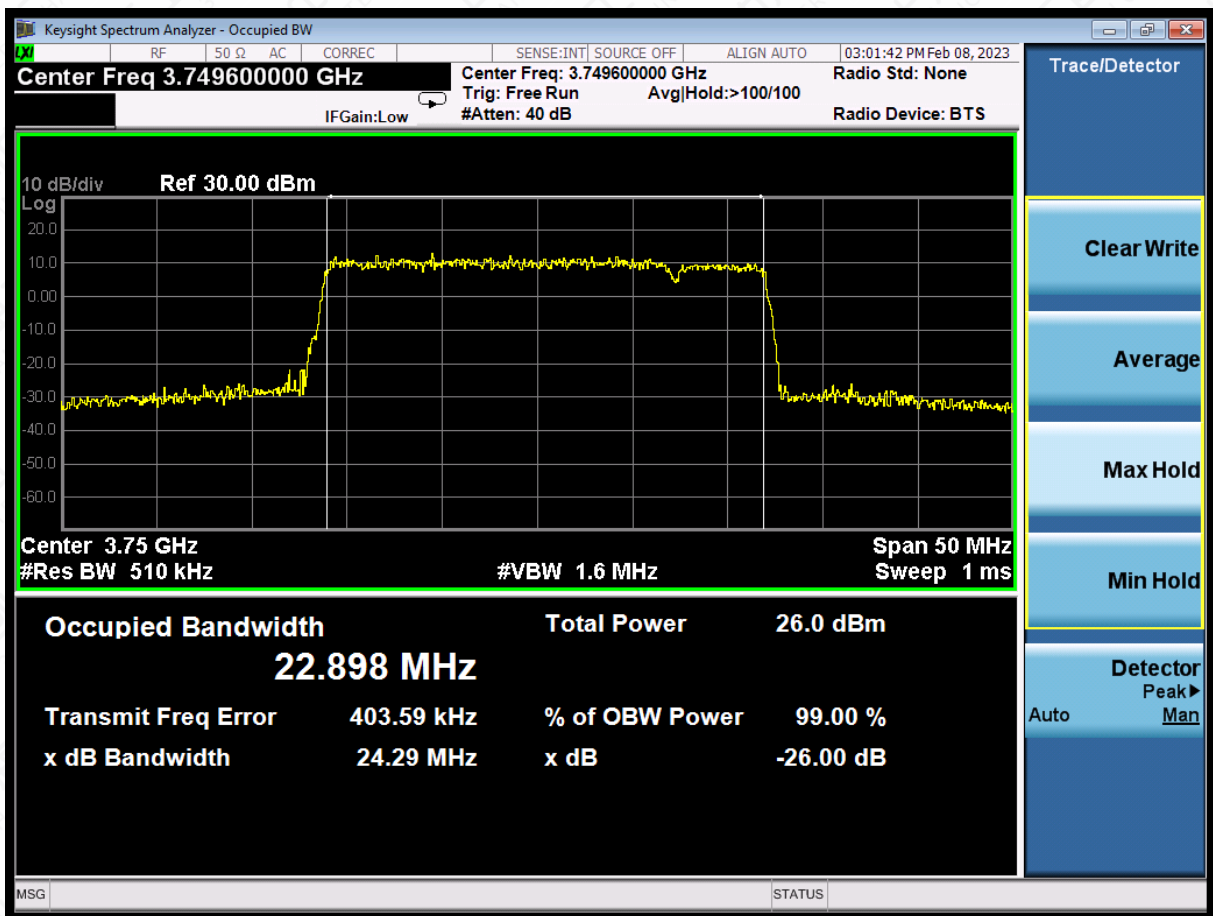
LTE CA band 43Part27 , 20MHz+5MHz Bandwidth,16QAM (-26dBc BW)
