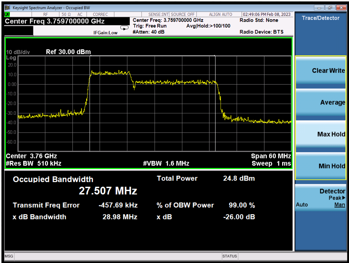
LTE CA band 43Part27 , 10MHz+20MHz Bandwidth,64QAM (-26dBc BW)
