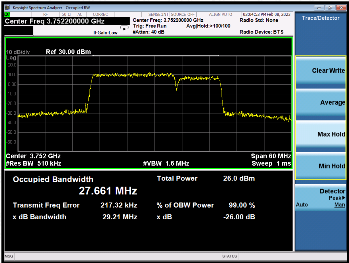
LTE CA band 43Part27 , 20MHz+10MHz Bandwidth,16QAM (-26dBc BW)
