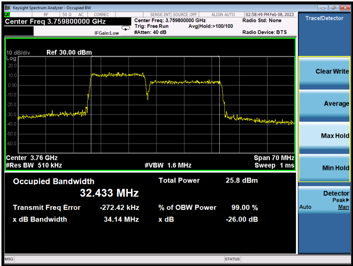
LTE CA band 43Part27 , 15MHz+20MHz Bandwidth,16QAM (-26dBc BW)
