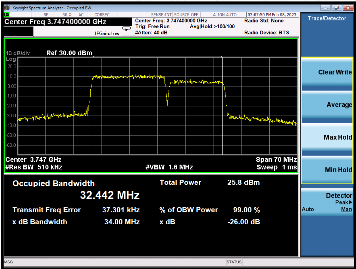
LTE CA band 43Part27 , 20MHz+15MHz Bandwidth,16QAM (-26dBc BW)
