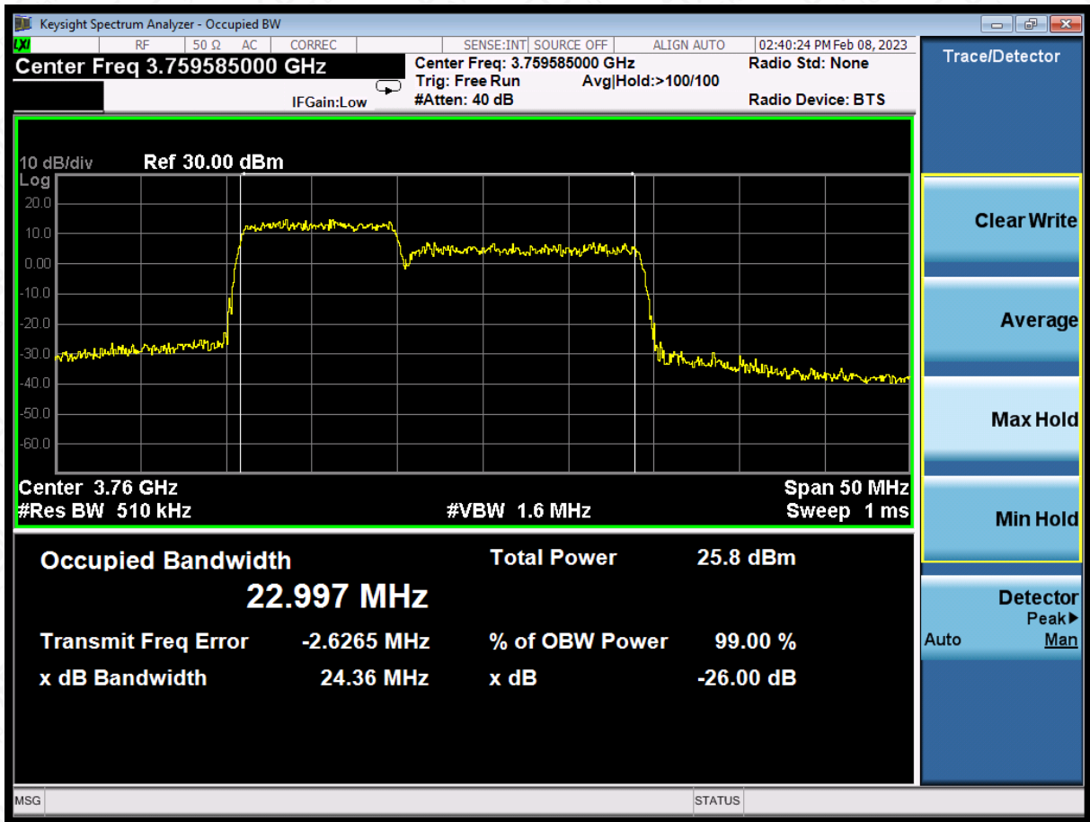
LTE CA band 43Part27 , 10MHz+15MHz Bandwidth,16QAM (-26dBc BW)
