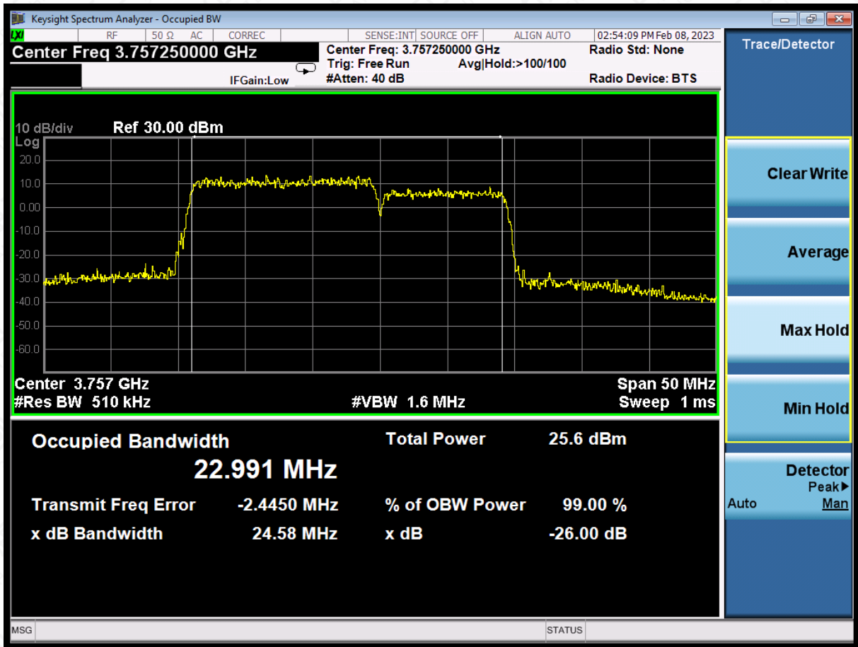
LTE CA band 43Part27 ,15MHz+10MHz Bandwidth,16QAM (-26dBc BW)
