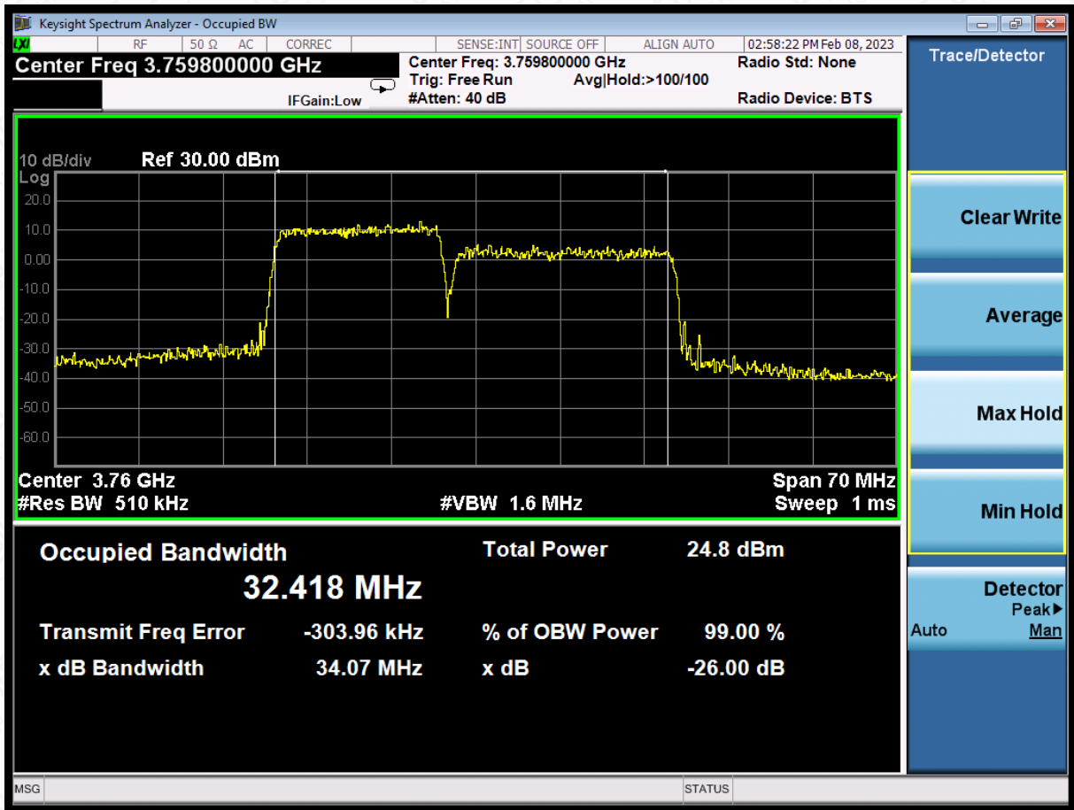
LTE CA band 43Part27 , 15MHz+20MHz Bandwidth,64QAM (-26dBc BW)
