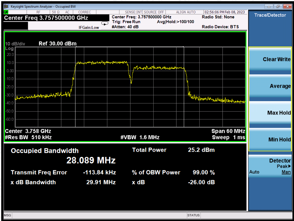
LTE CA band 43Part27 , 15MHz+15MHz Bandwidth,64QAM (-26dBc BW)
