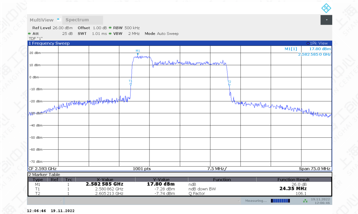
LTE CA band 41 , 5MHz+20MHz Bandwidth,QPSK (-26dBc BW)
