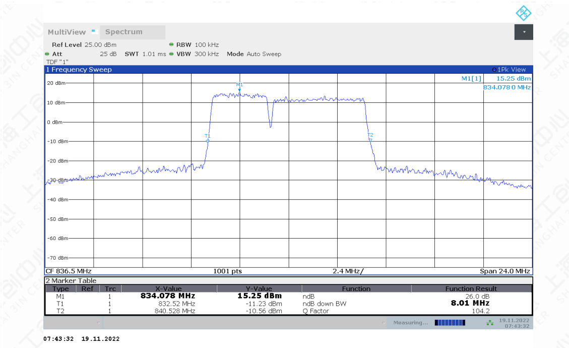
LTE CA band 5 , 3MHz+5MHz Bandwidth,QPSK (-26dBc BW)
