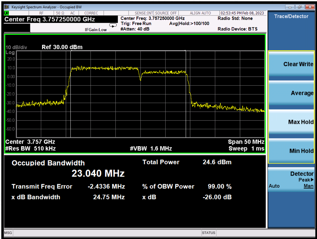
LTE CA band 43Part27 , 15MHz+10MHz Bandwidth,64QAM (-26dBc BW)
