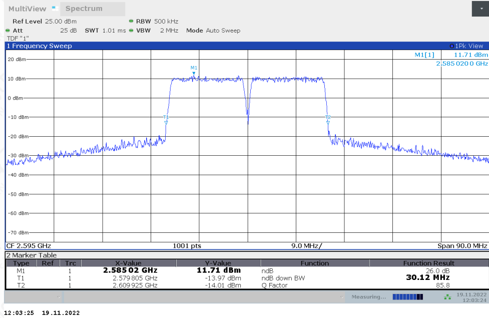
LTE CA band 38 , 15MHz+15MHz Bandwidth,64QAM (-26dBc BW)
