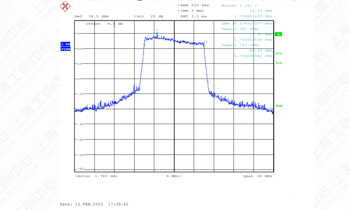
LTE band 66@CA_2+66, 20MHz Bandwidth, 64QAM (99% BW)
