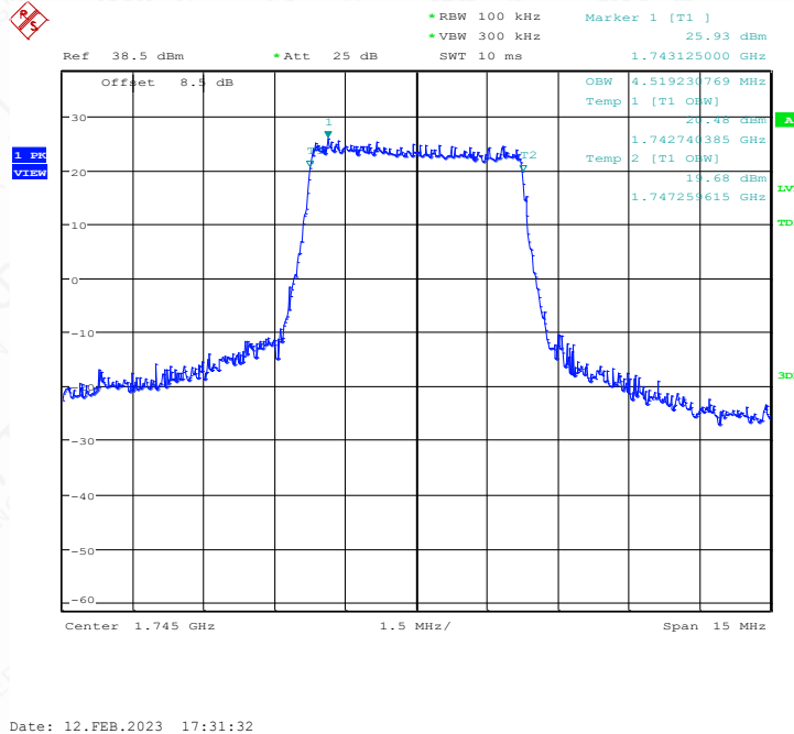
LTE band 66@CA_2+66, 5MHz Bandwidth, 64QAM (99% BW)
