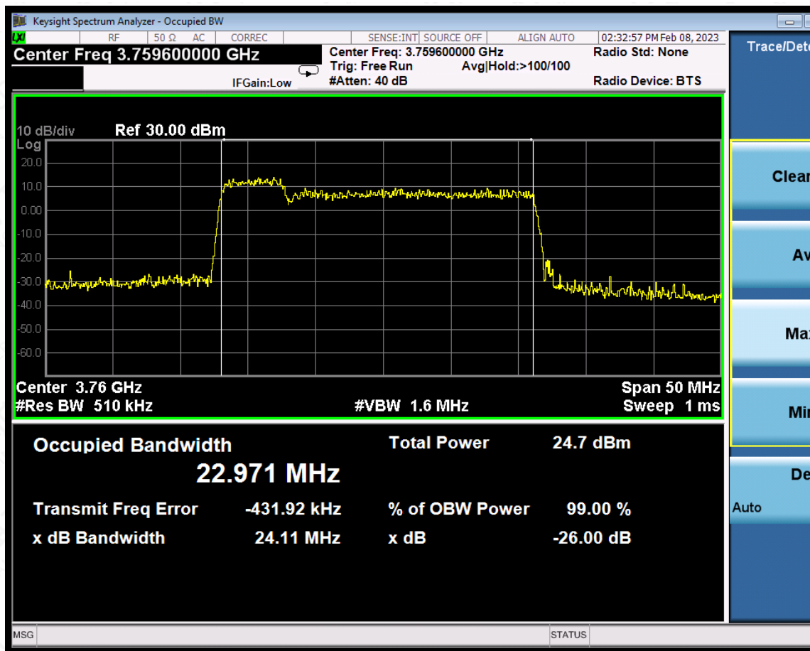
LTE CA band 43Part27 , 5MHz+20MHz Bandwidth,64QAM (99% BW)
