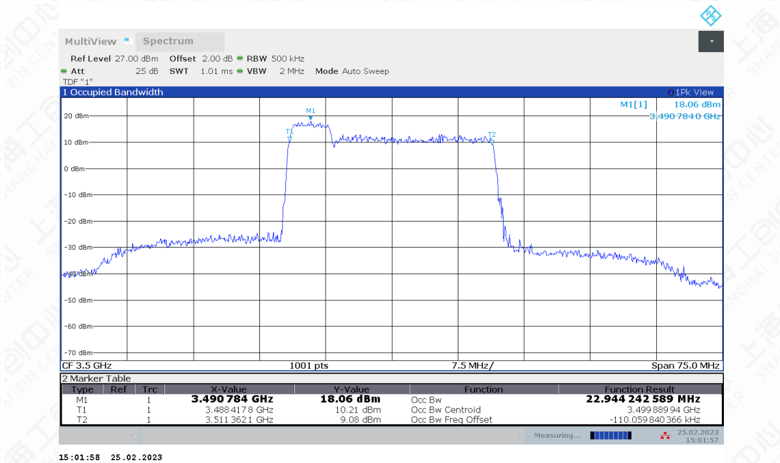
LTE CA band 42Part27, 5MHz+20MHz Bandwidth,QPSK (99% BW)
