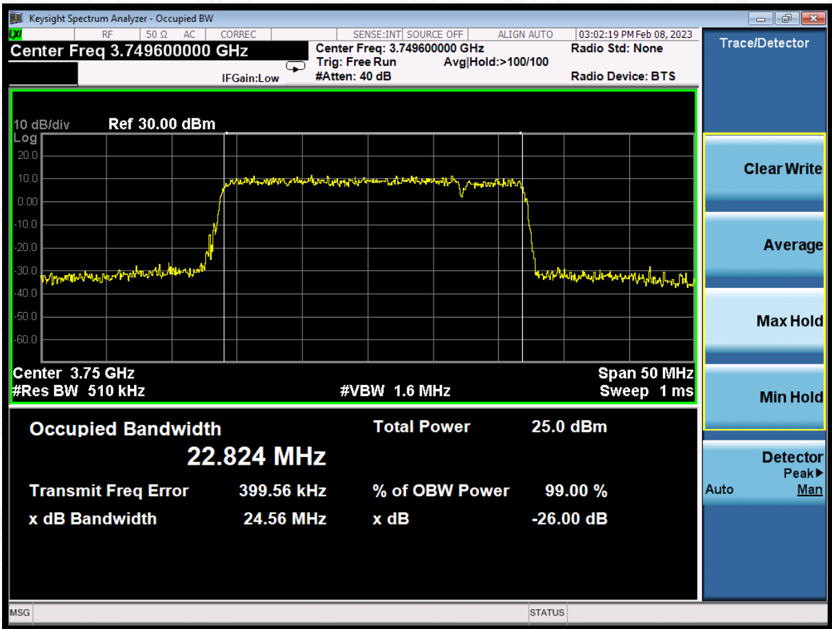
LTE CA band 43Part27 , 20MHz+5MHz Bandwidth,64QAM (99% BW)
