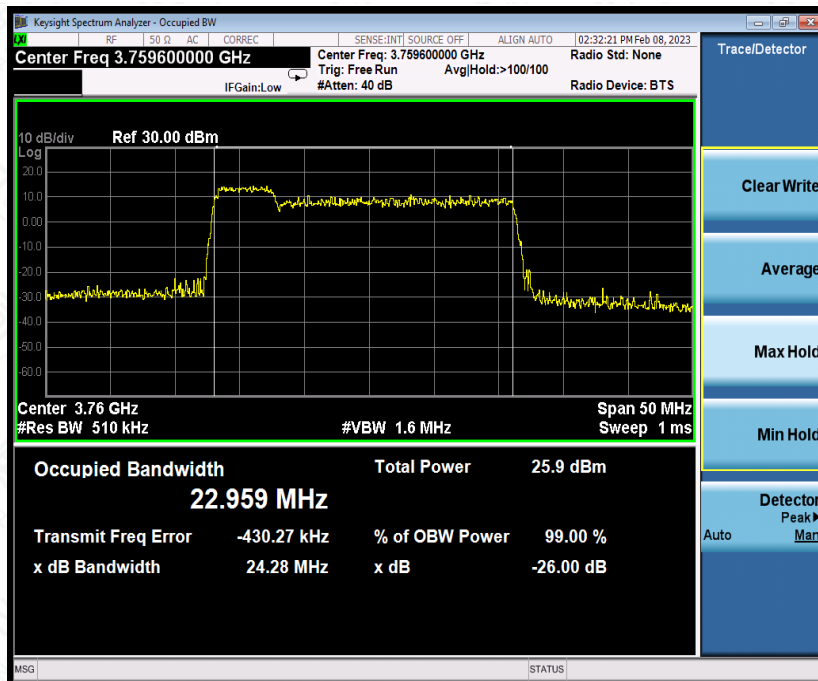
LTE CA band 43Part27 , 5MHz+20MHz Bandwidth,QPSK (99% BW)
