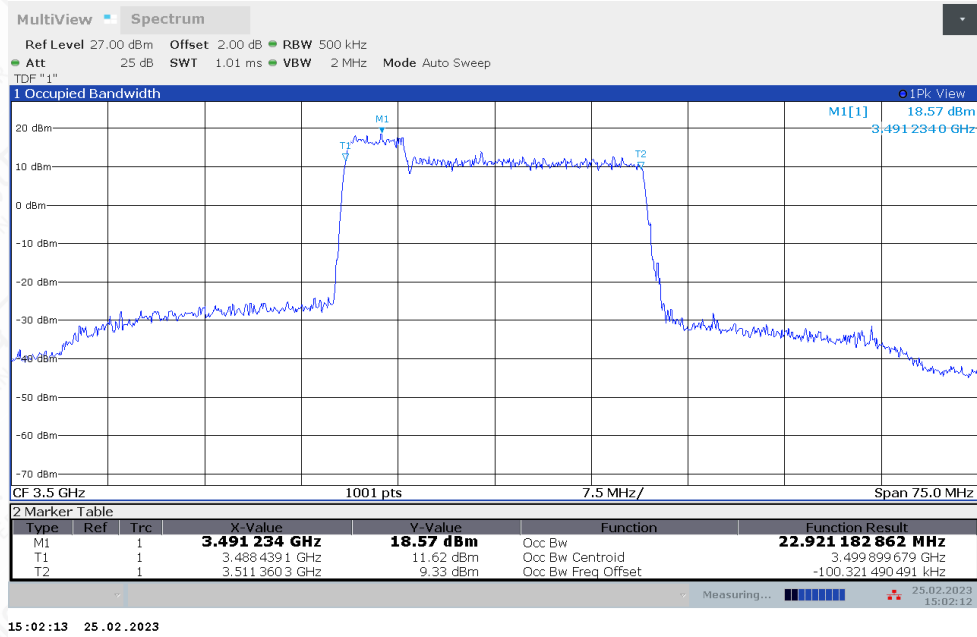
LTE CA band 42Part27 , 5MHz+20MHz Bandwidth,64QAM (99% BW)
