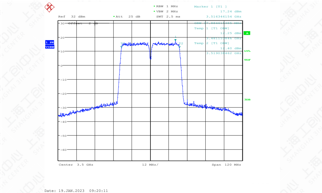
LTE CA band 43Part27,5MHz+20MHz(99%)*
