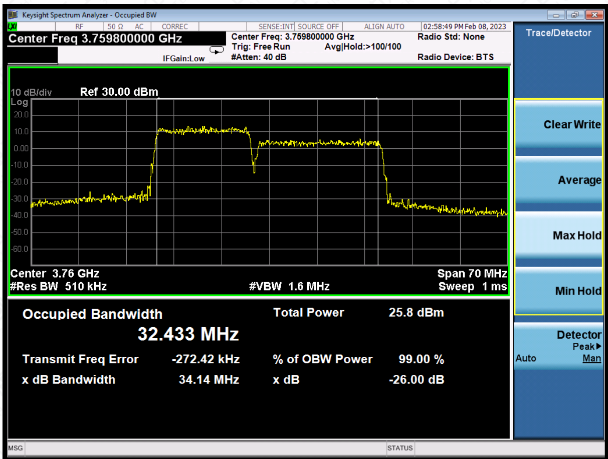
LTE CA band 43Part27 , 15MHz+20MHz Bandwidth,16QAM (99% BW)
