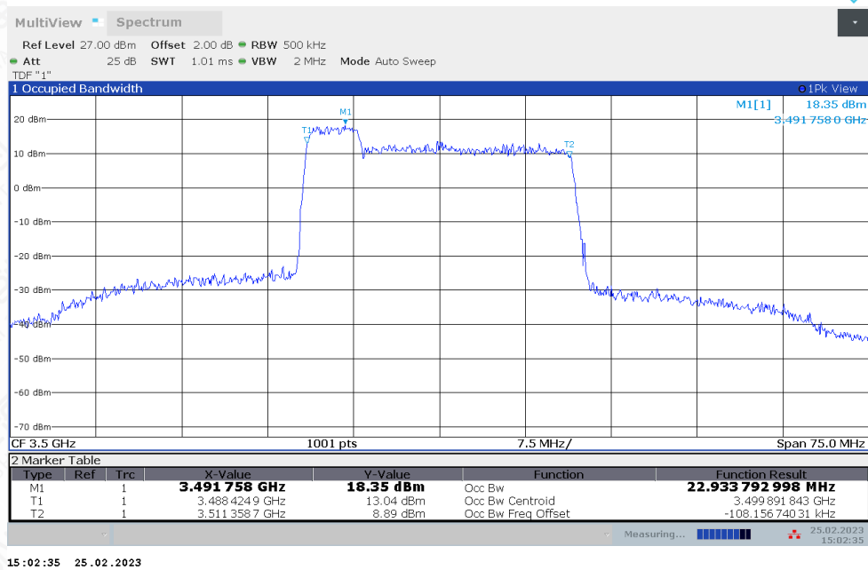
LTE CA band 42Part27 , 5MHz+20MHz Bandwidth,64QAM (99% BW)
