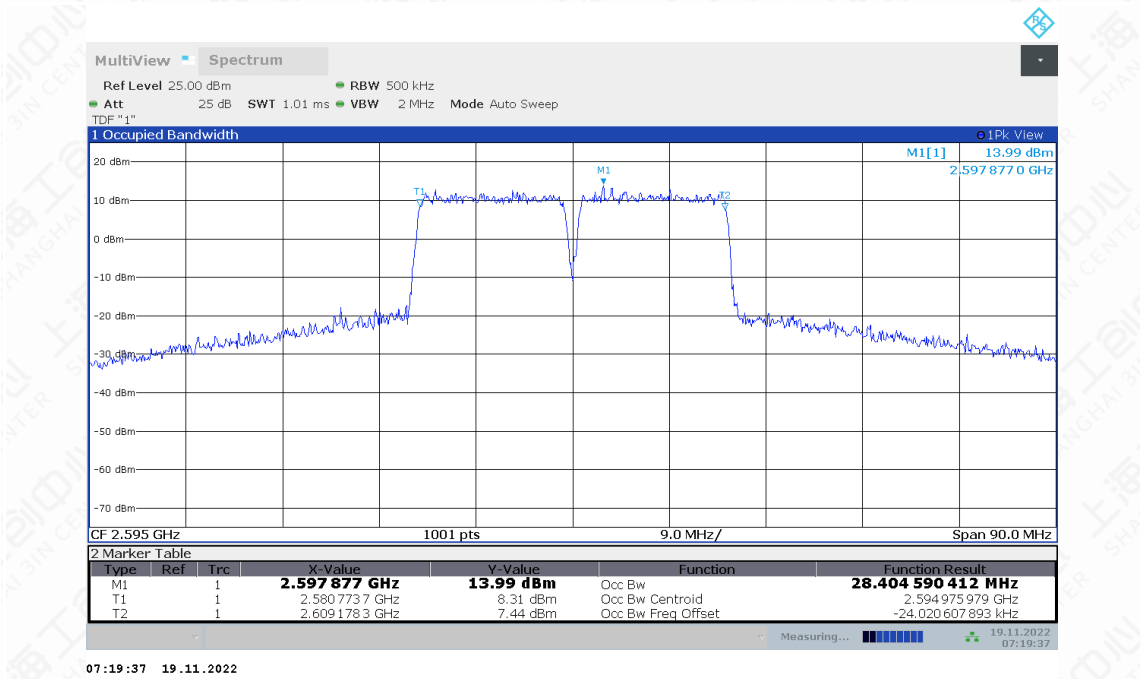
LTE CA band 38 , 15MHz+15MHz Bandwidth,QPSK (99% BW)
