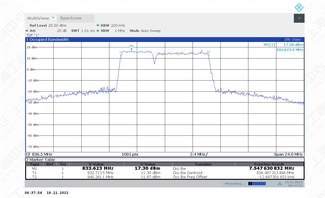
LTE CA band 5 , 3MHz+5MHz Bandwidth,QPSK (99% BW)
