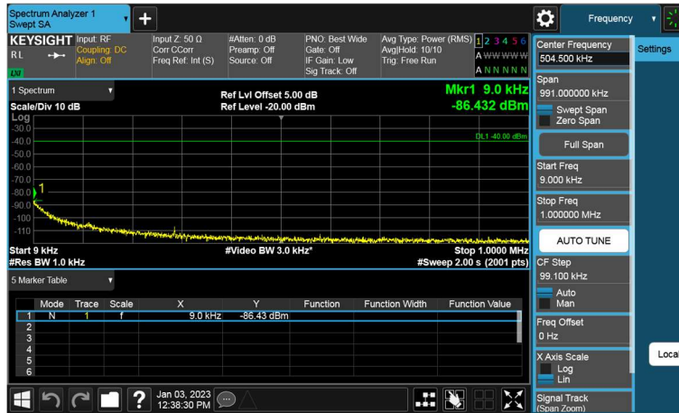
20M_5M_QPSK_1RB_CSE1
