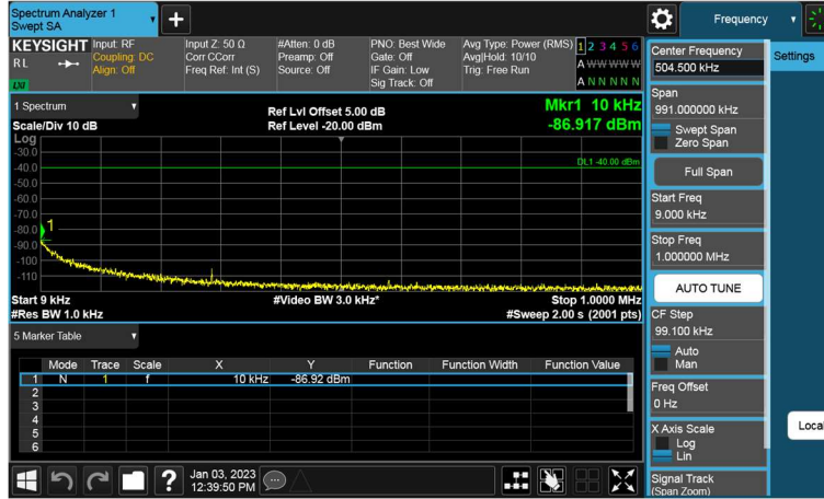
20M_5M_Q64_FULLLRB_CSE0b
