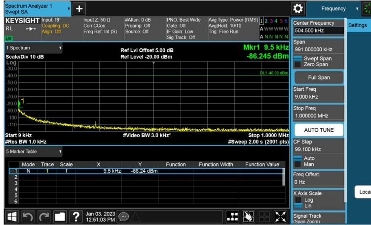
15M_20M_Q64_FULLRB_CSE0b
