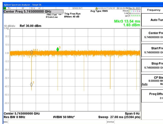
UNII-3-11n-HT20-Duty cycle
