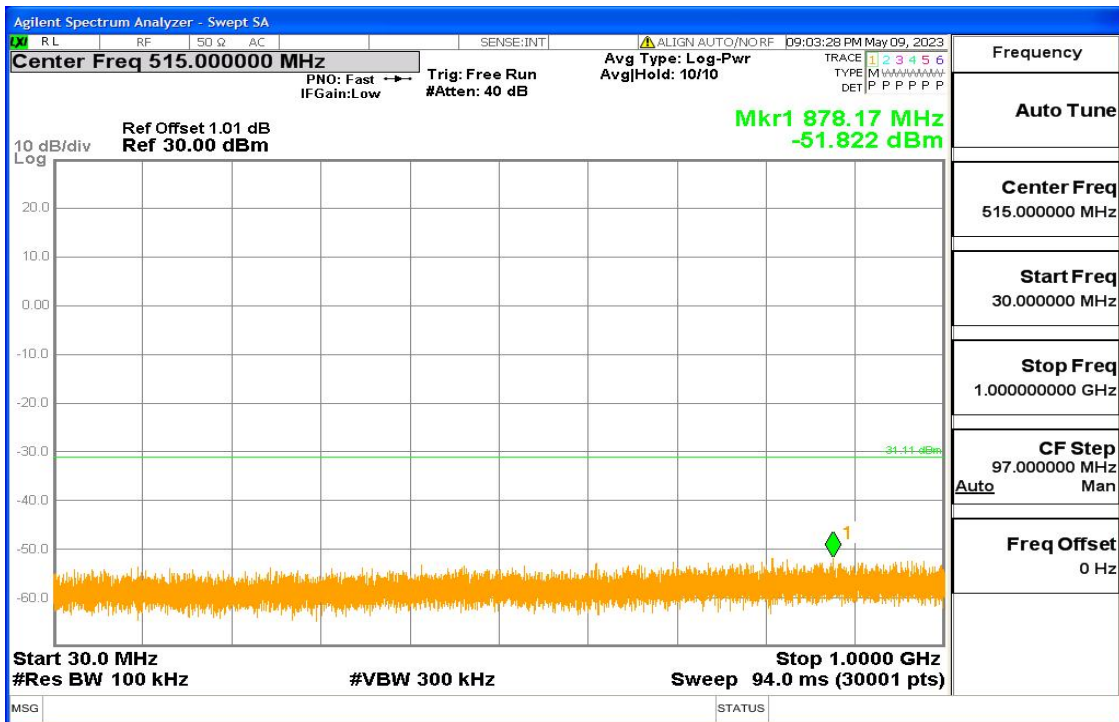
11g Fig2
