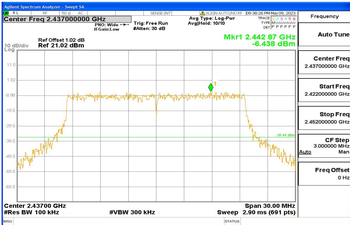
11ax-HE20 Fig4
