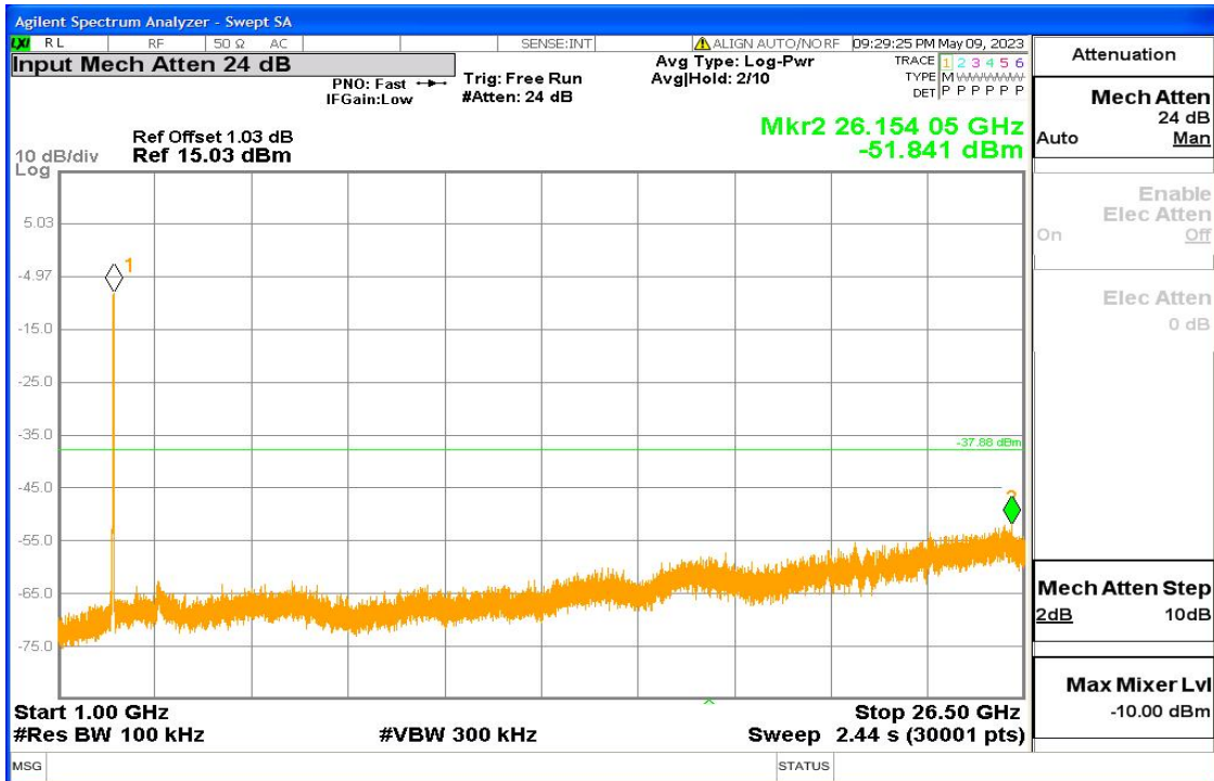
11n-HT40 Fig9
