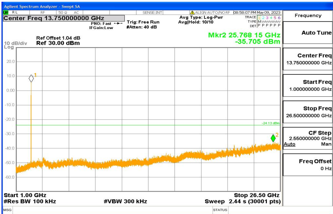
11b Fig9
