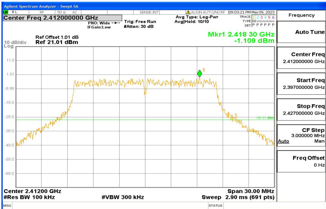
11g Fig1
