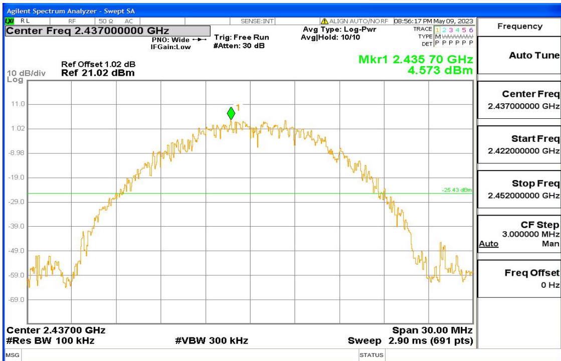
11b Fig4
