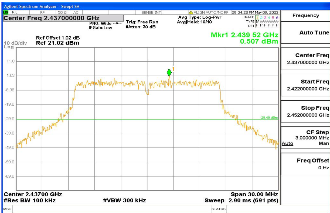
11g Fig4
