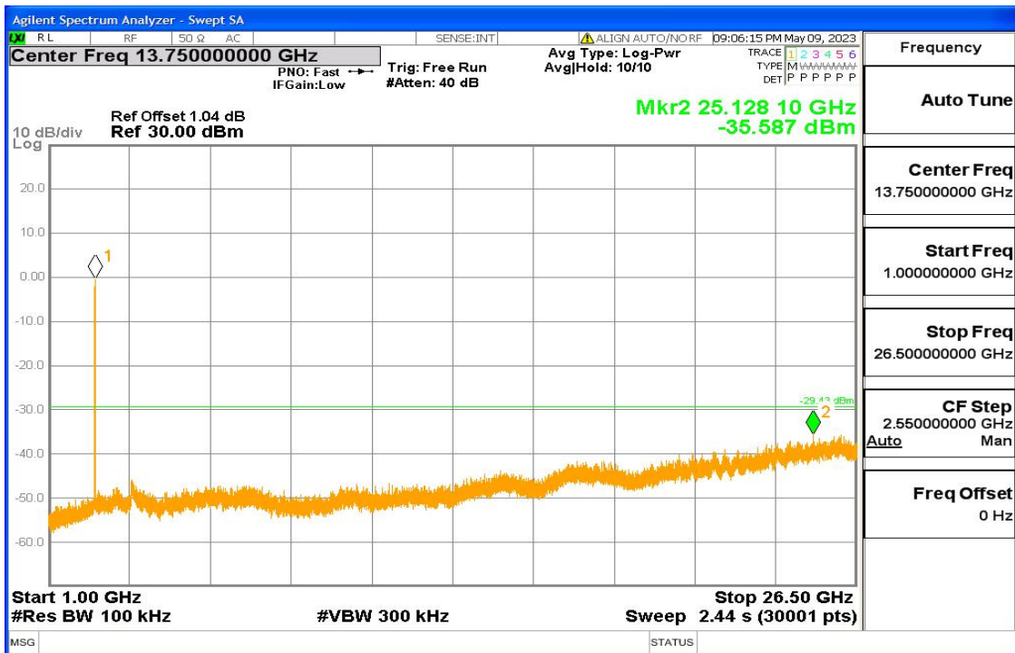
11g Fig9
