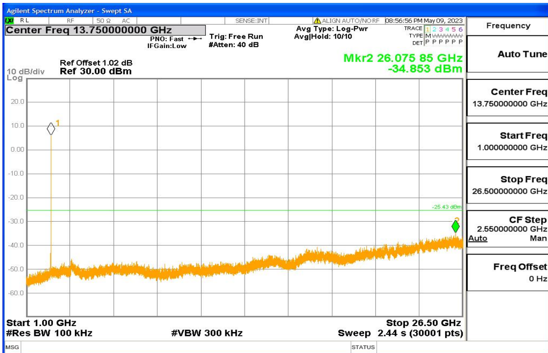
11b Fig6
