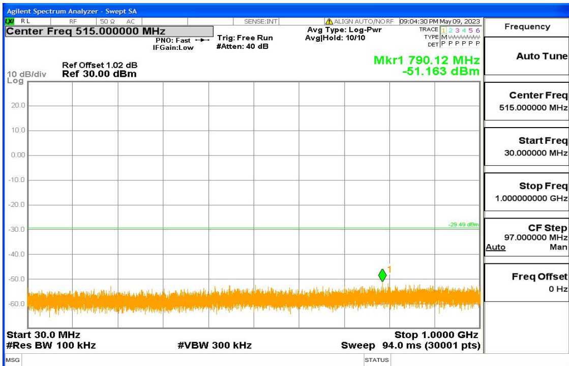
11g Fig5
