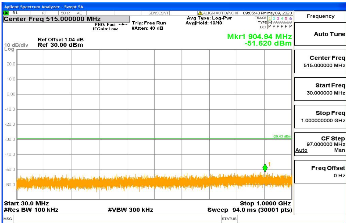
11g Fig8
