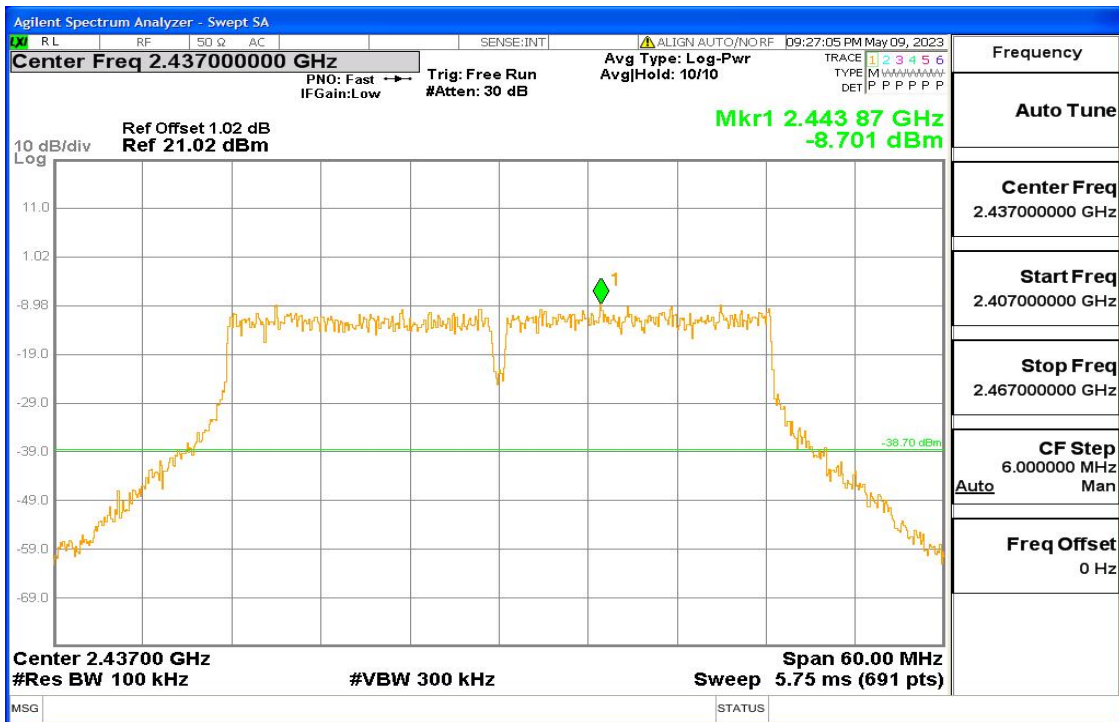
11n-HT40 Fig4
