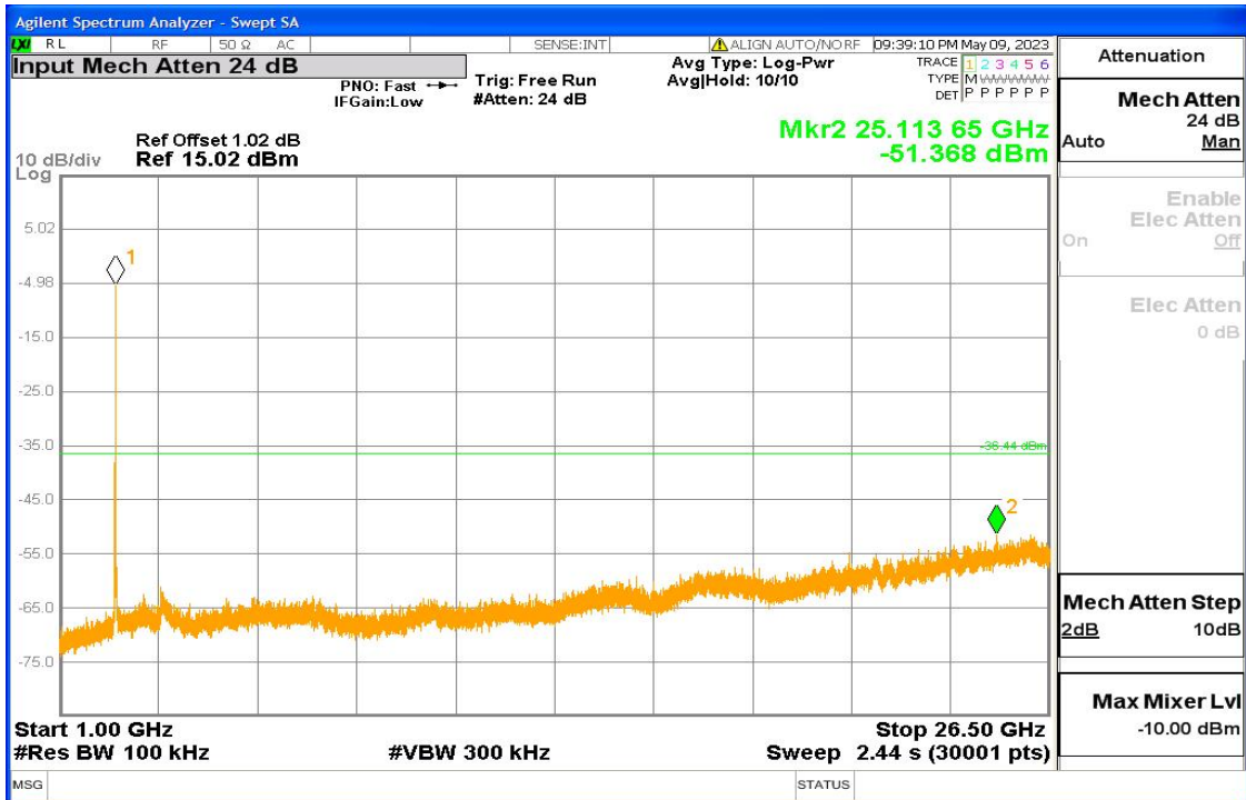
11ax-HE20 Fig6
