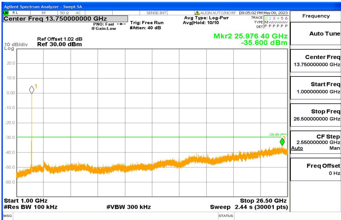
11g Fig6
