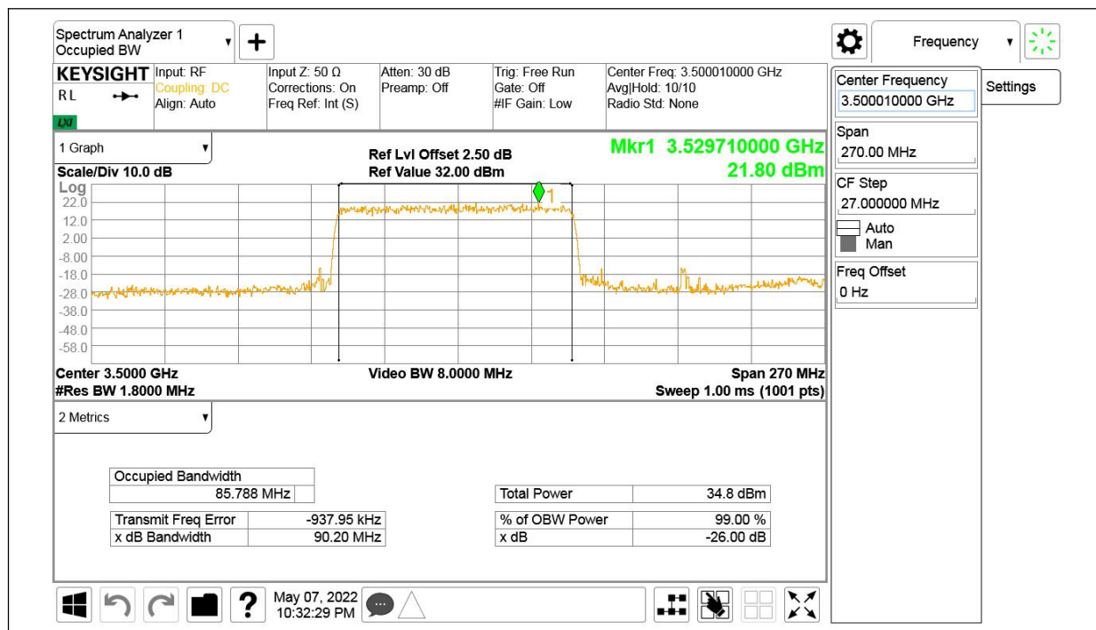
n77L,100MHz(99%)
