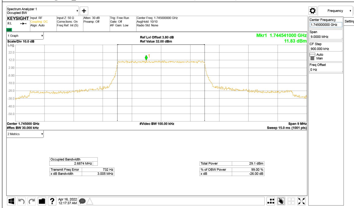
LTE band 66@CA_12+66, 3MHz Bandwidth, QPSK (-26dBc BW)
