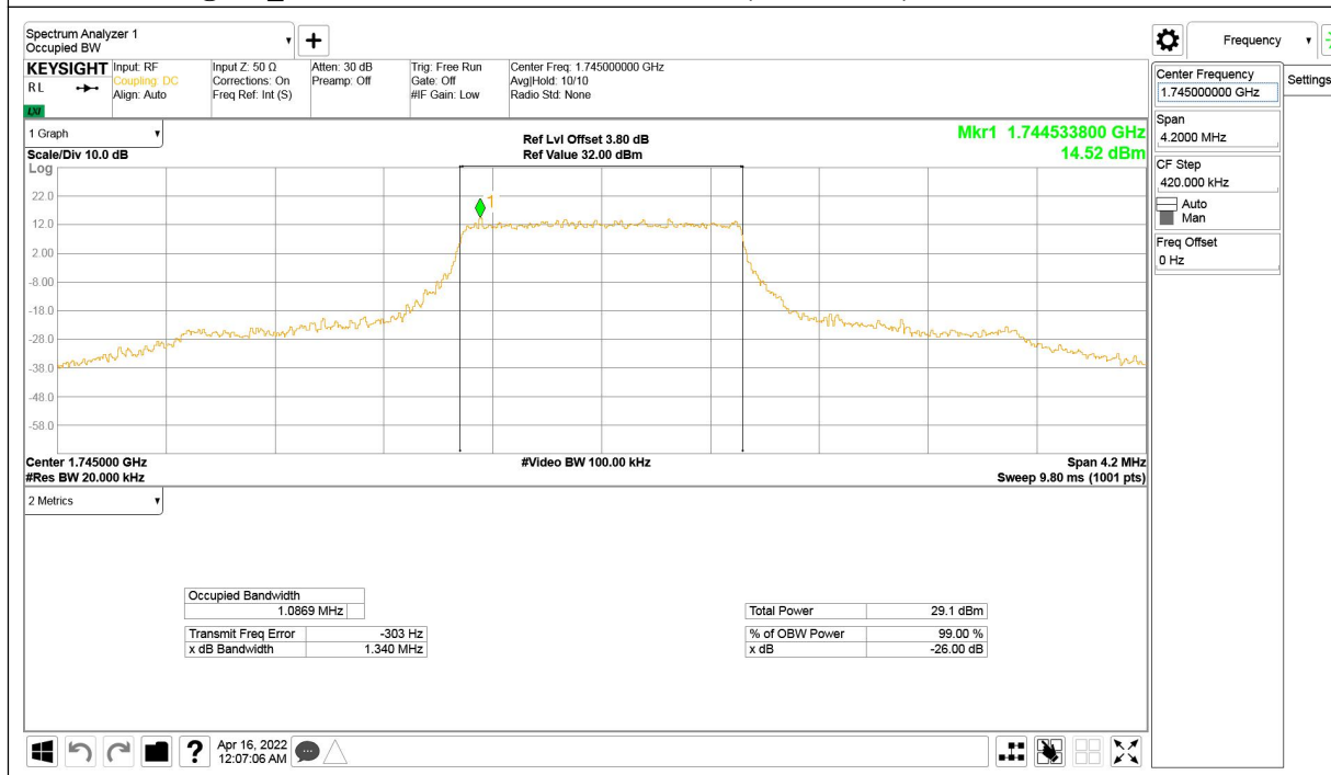
LTE band 66@CA_12+66, 1.4MHz Bandwidth, QPSK (-26dBc BW)
