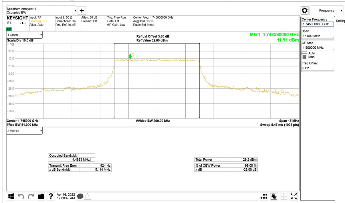
LTE band 66@CA_2+66, 5MHz Bandwidth, QPSK (-26dBc BW)
