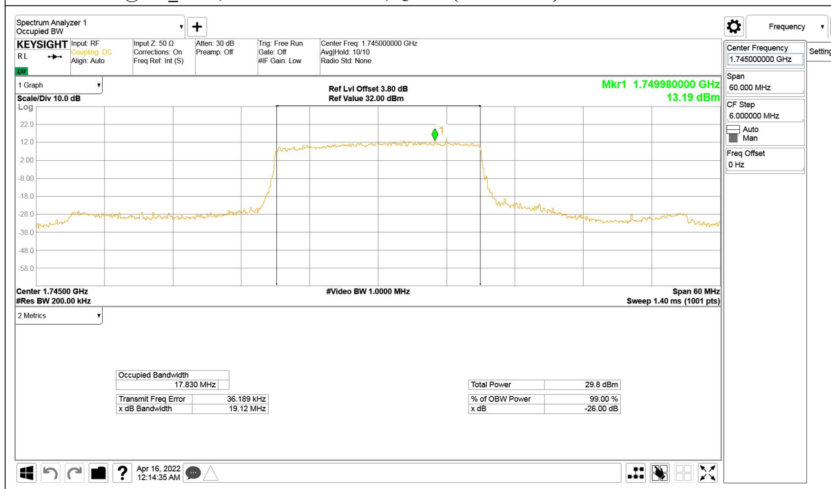
LTE band 66@CA_2+66, 20MHz Bandwidth, QPSK (-26dBc BW)
