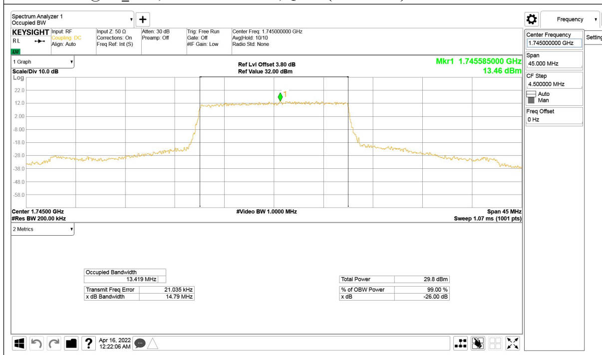
LTE band 66@CA_2+66, 15MHz Bandwidth, QPSK (-26dBc BW)
