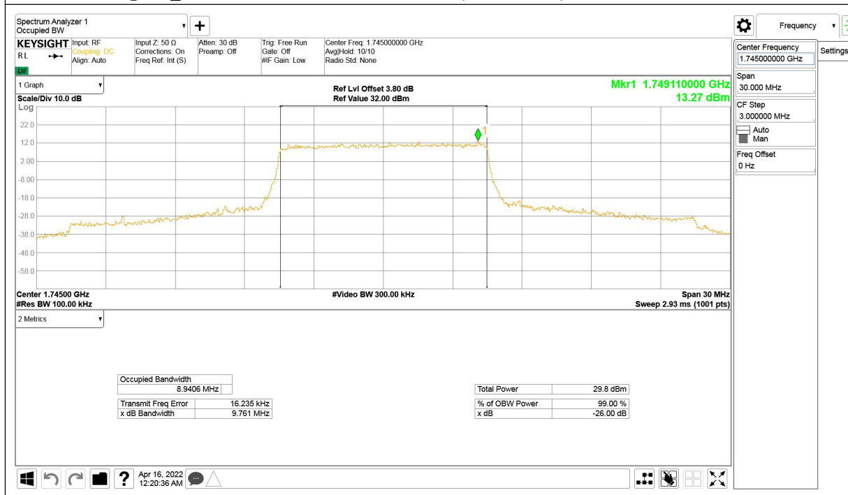
LTE band 66@CA_2+66, 10MHz Bandwidth, QPSK (-26dBc BW)
