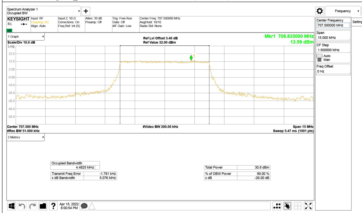
LTE band 12@CA_2+12, 5MHz Bandwidth, QPSK (99% BW)
