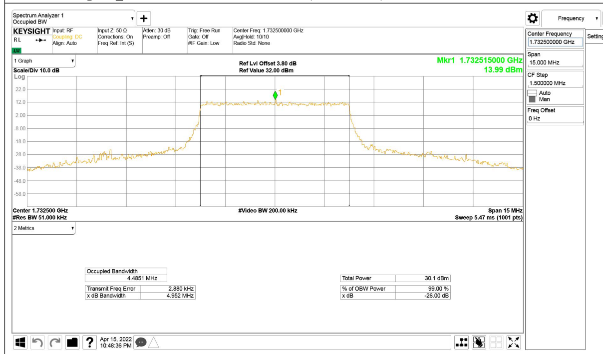
LTE band 4@CA_2+4, 5MHz Bandwidth, QPSK (-26dBc BW)
