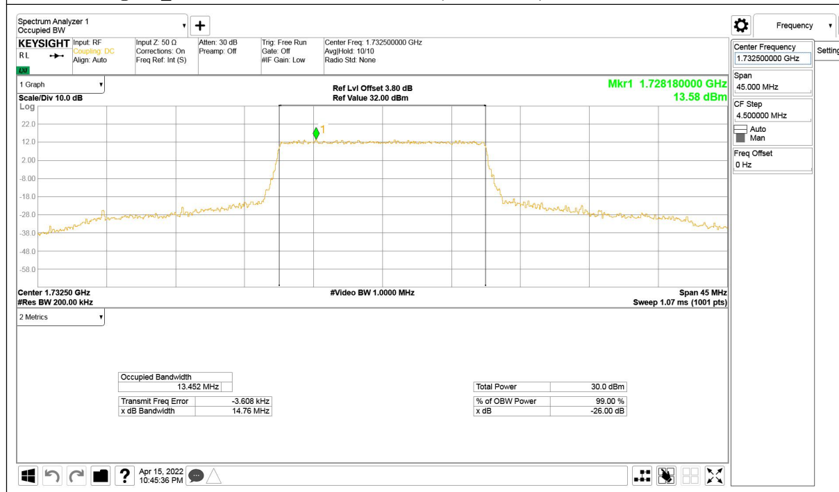
LTE band 4@CA_2+4, 15MHz Bandwidth, QPSK (-26dBc BW)
