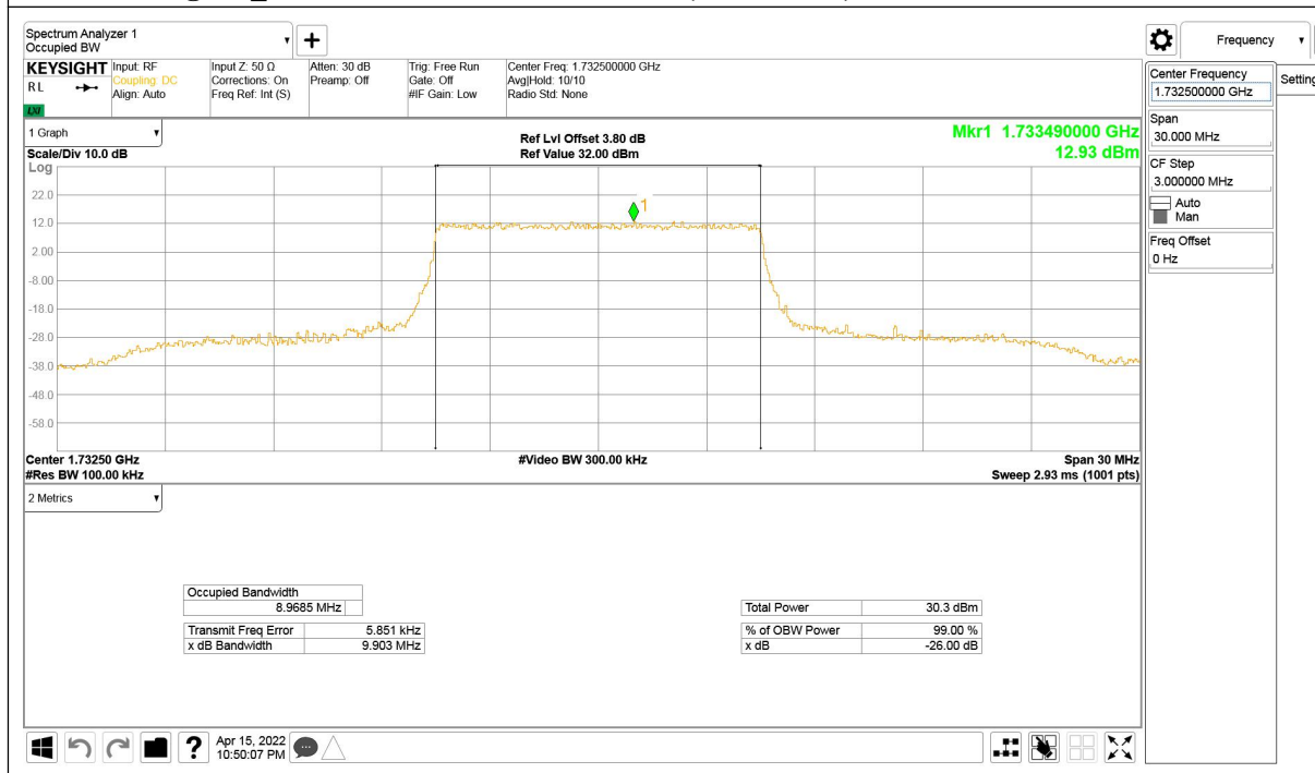
LTE band 4@CA_2+4, 10MHz Bandwidth, QPSK (-26dBc BW)
