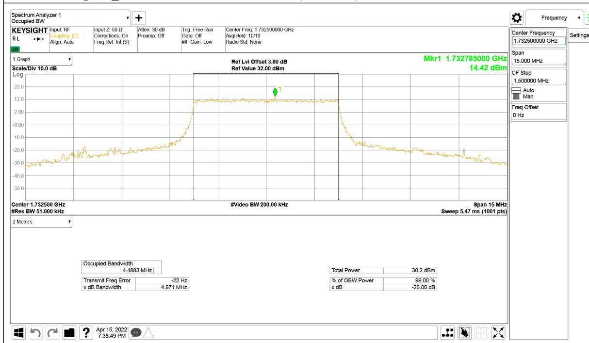
LTE band 4@CA_2+4, 5MHz Bandwidth, QPSK (99% BW)
