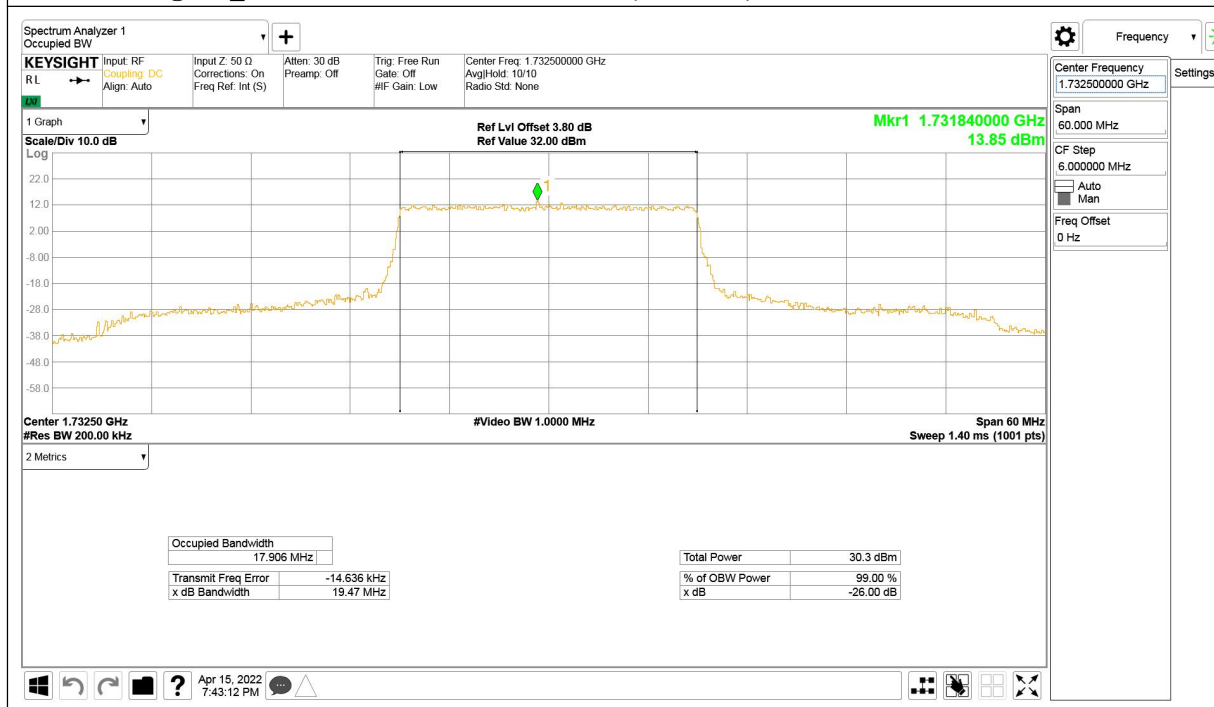
LTE band 4@CA_2+4, 20MHz Bandwidth, QPSK (99% BW)
