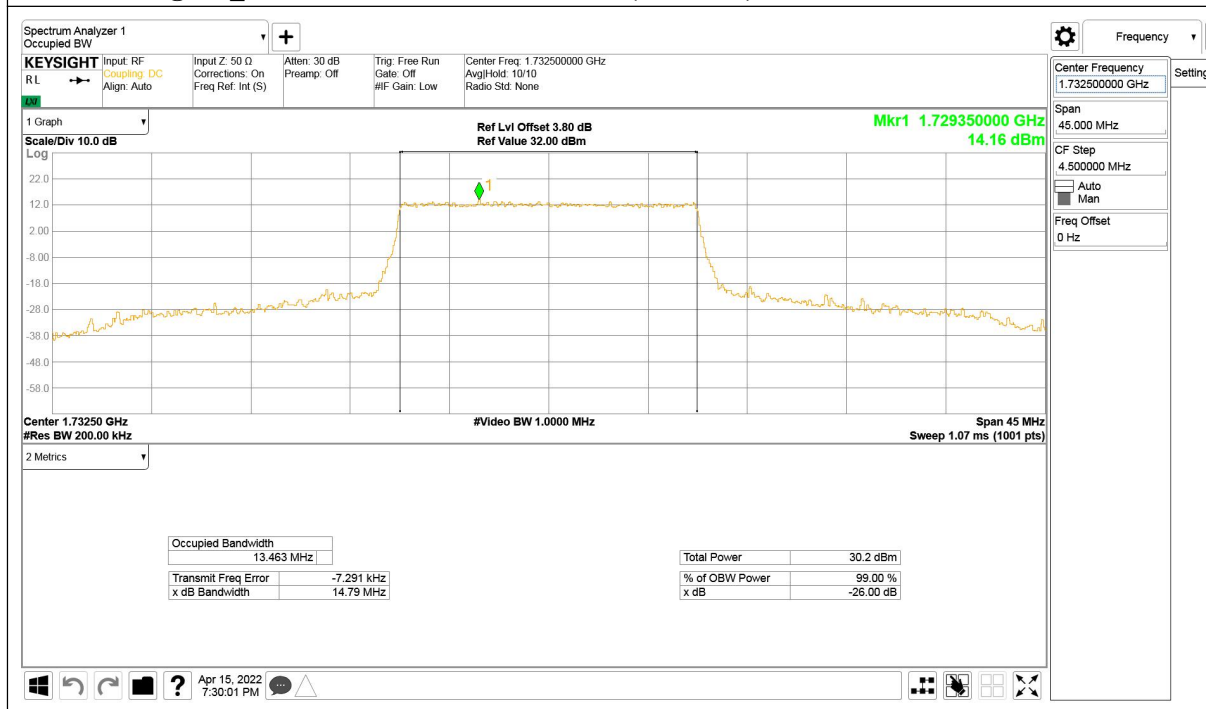
LTE band 4@CA_2+4, 15MHz Bandwidth, QPSK (99% BW)
