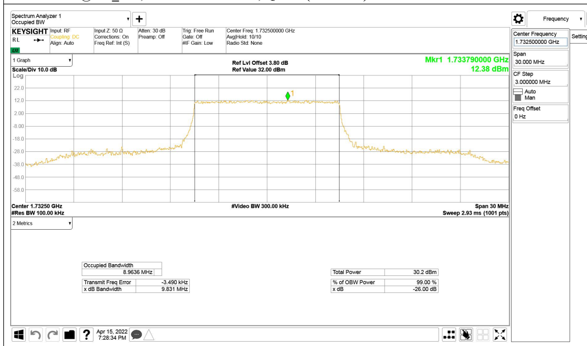
LTE band 4@CA_2+4, 10MHz Bandwidth, QPSK (99% BW)
