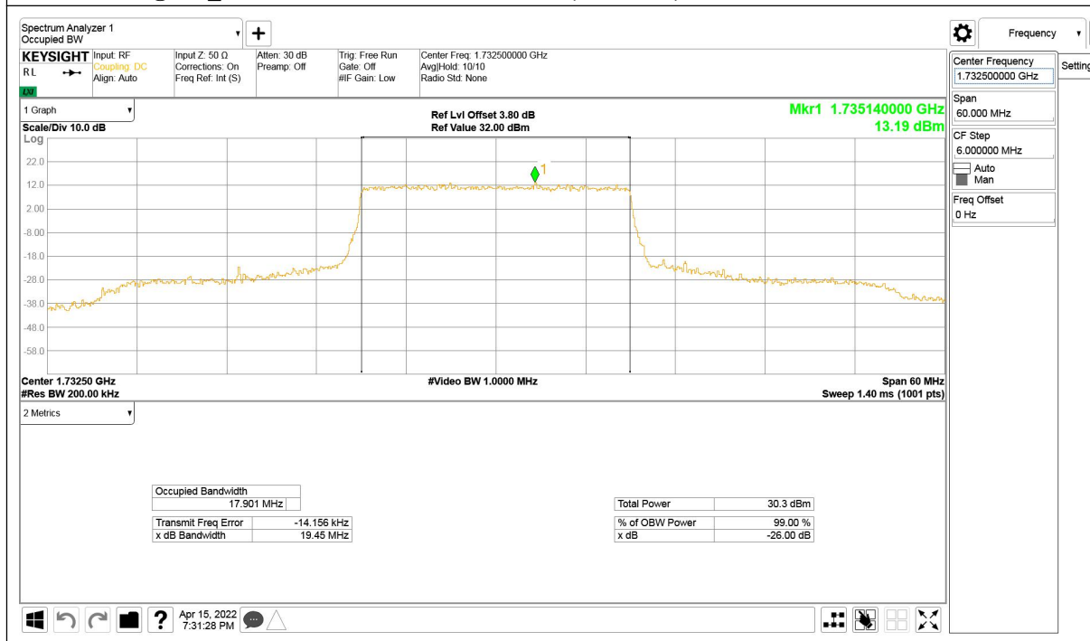
LTE band 4@CA_2+4, 20MHz Bandwidth, QPSK (99% BW)
