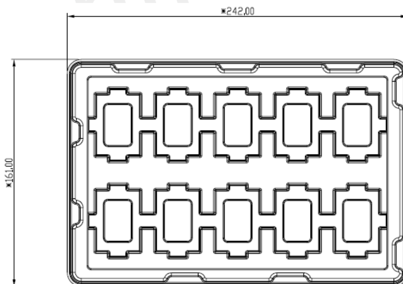
Figure 36: Tray drawing
