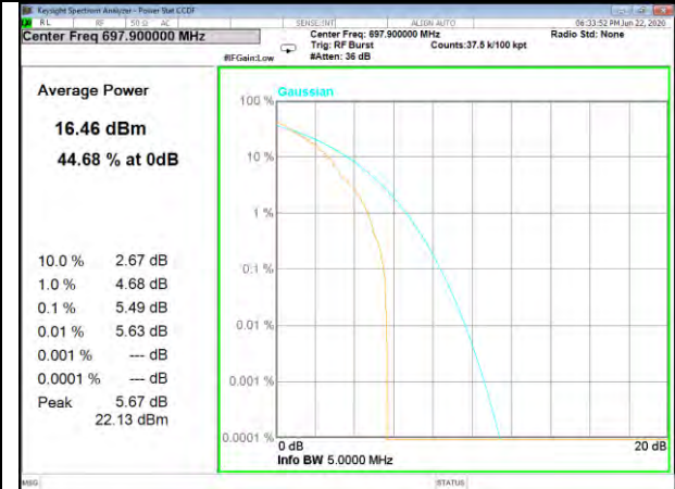
Band71_15kHz_QPSK_12#0_High
