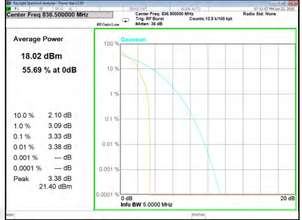
Band5_15kHz_QPSK_12#0_Middle
