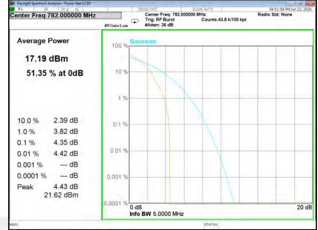
Band13_15kHz_QPSK_12#0_Middle
