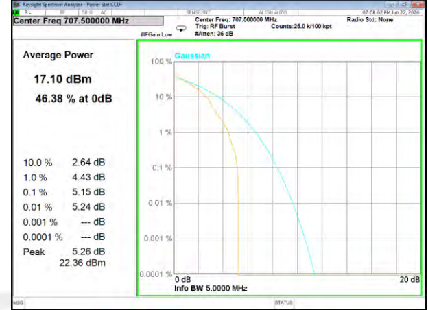
Band12_15kHz_QPSK_12#0_Middle
