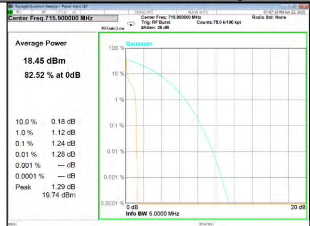
Band12_15kHz_QPSK_High
