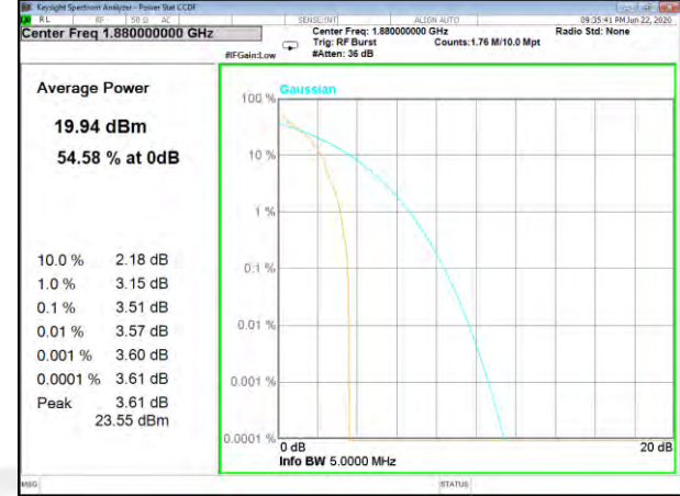
Band2_15kHz_QPSK_12#0_Middle
