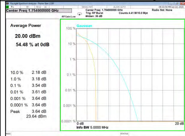
Band4_15kHz_QPSK_12#0_High
