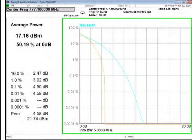
Band13_15kHz_QPSK_12#0_High
