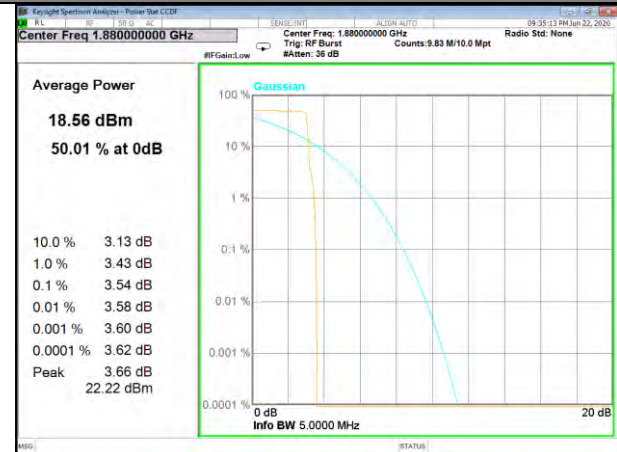
Band2_15kHz_BPSK_High
