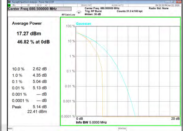
Band71_15kHz_QPSK_12#0_Middle
