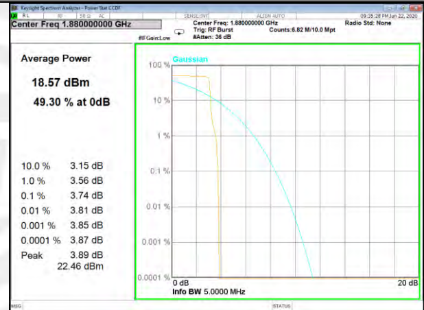
Band2_15kHz_QPSK_High
