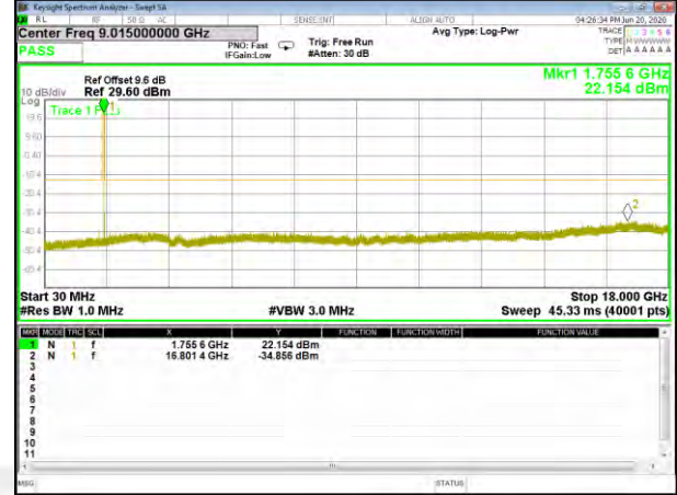
Band4_15kHz_QPSK_High_12#0
