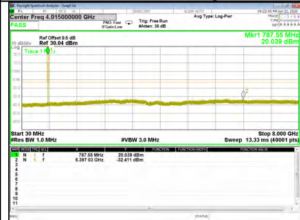
Band13_15kHz_QPSK_High_12#0
