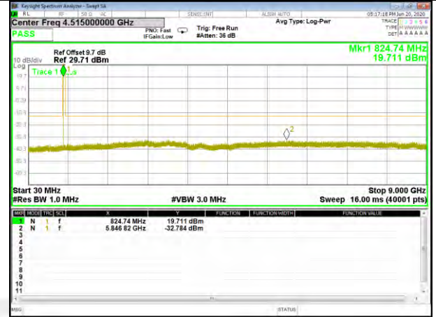
Band5_15kHz_BPSK_Middle_1#0
