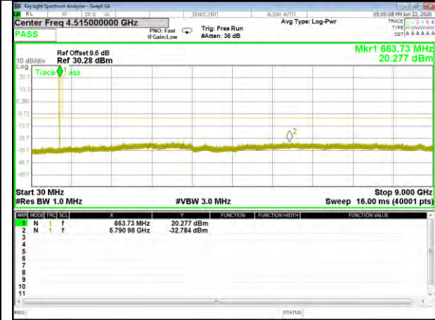
Band71_15kHz_QPSK_High_12#0
