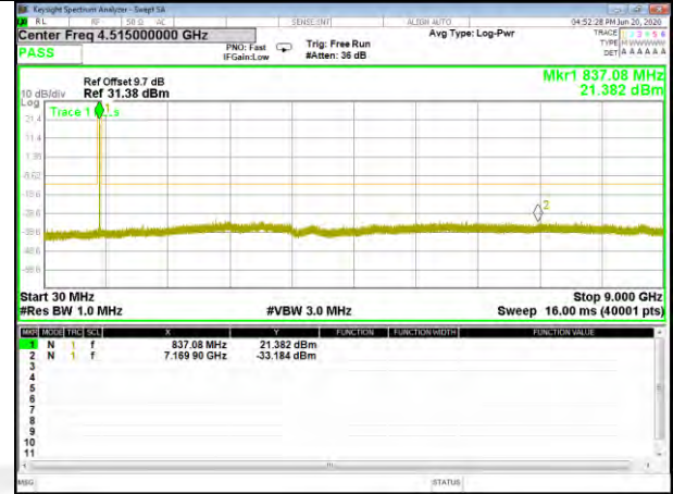
Band5_15kHz_QPSK_Middle_12#0
