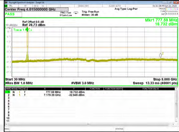
Band13_3.55kHz_BPSK_Middle_1#0
