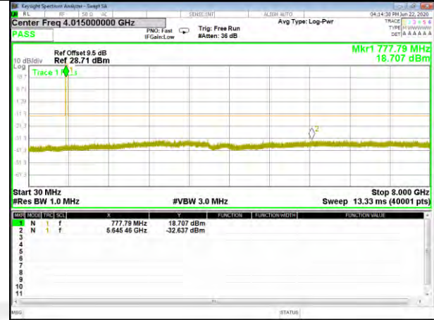
Band13_15kHz_BPSK_Middle_1#0
