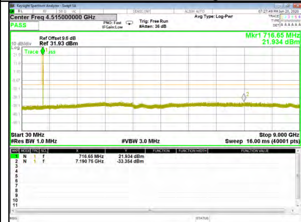
Band12_15kHz_QPSK_High_12#0
