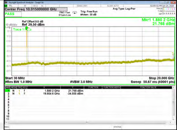
Band2_15kHz_QPSK_Middle_12#0
