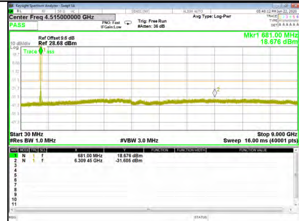
Band71_3.75kHz_QPSK_High_1#0
