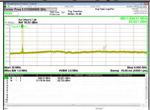
Band5_3.75kHz_BPSK_High_1#0
