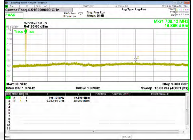
Band12_15kHz_QPSK_Middle_12#0
