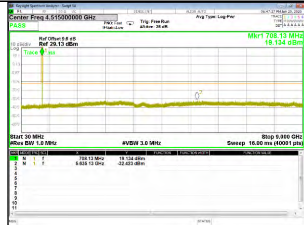
Band12_15kHz_QPSK_High_1#0
