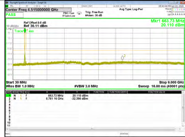
Band71_3.75kHz_QPSK_Middle_1#0
