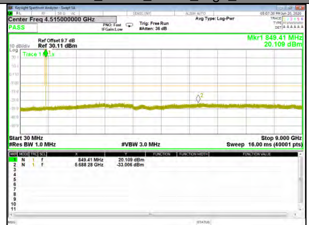
Band5_15kHz_BPSK_High_1#0
