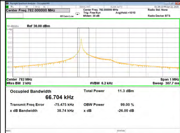
Band13_3.55kHz_QPSK_High_1#0
