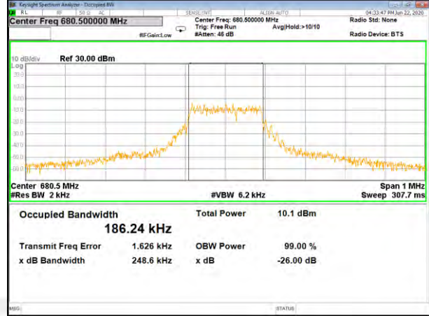
Band71_15kHz_QPSK_Middle_12#0
