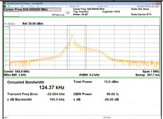
Band5_15kHz_BPSK_High_1#0
