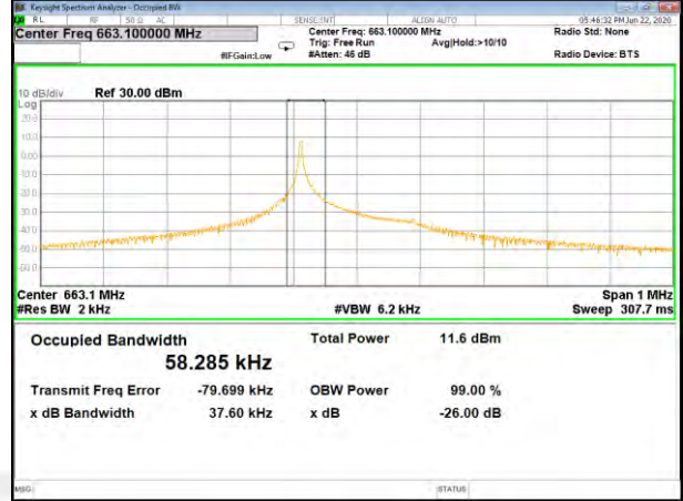
Band71_3.75kHz_BPSK_Middle_1#0
