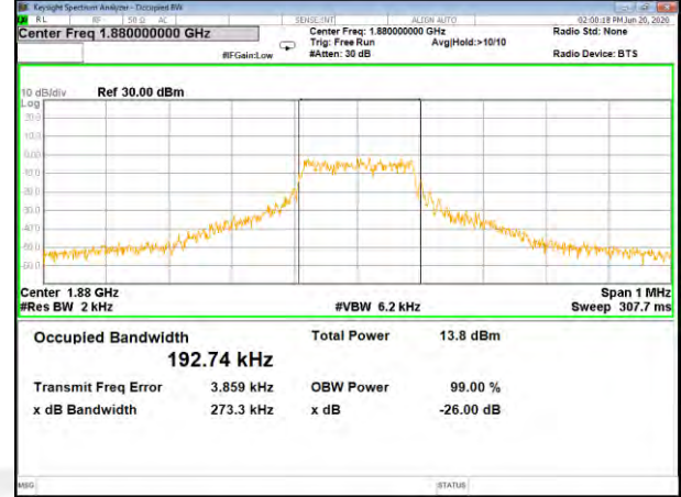
Band2_15kHz_QPSK_Middle_12#0
