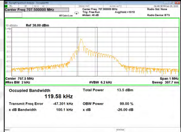
Band12_15kHz_16QAM_High_1#0
