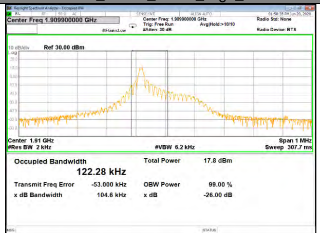
Band2_15kHz_BPSK_High_1#0
