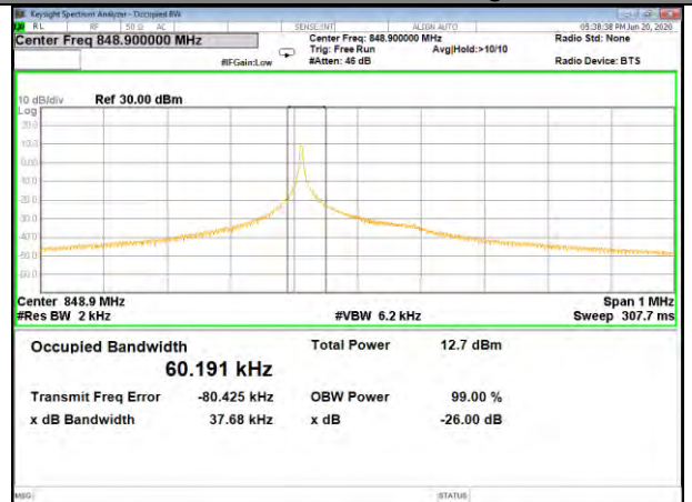
Band5_3.75kHz_BPSK_High_1#0
