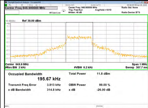
Band5_15kHz_QPSK_High_12#0
