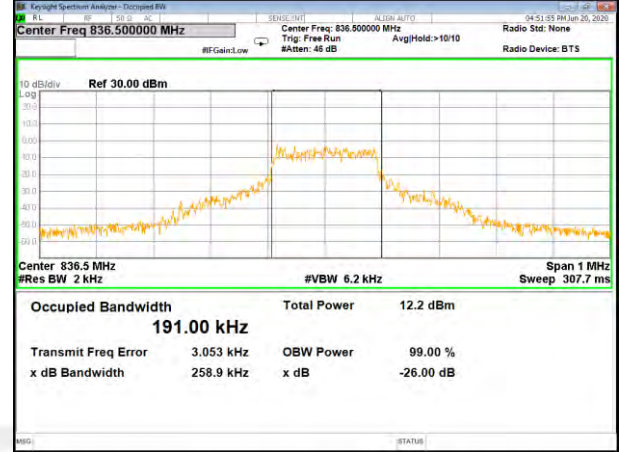
Band5_15kHz_QPSK_Middle_12#0
