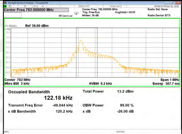
Band13_15kHz_BPSK_High_1#0
