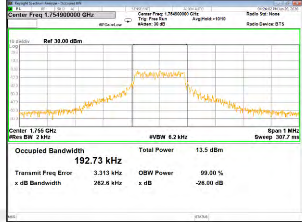
Band4_15kHz_QPSK_High_12#0
