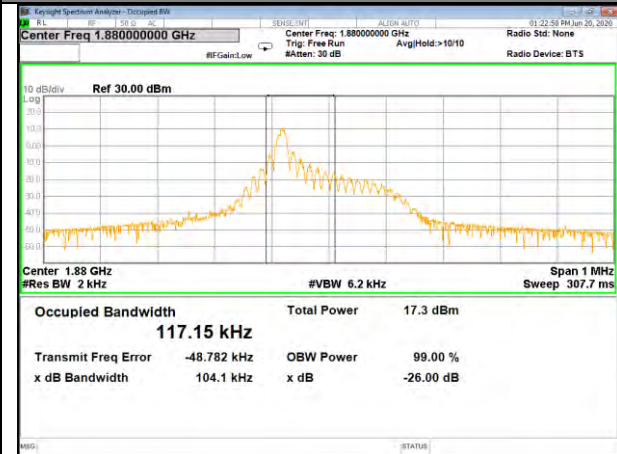
Band2_15kHz_QPSK_High_1#0
