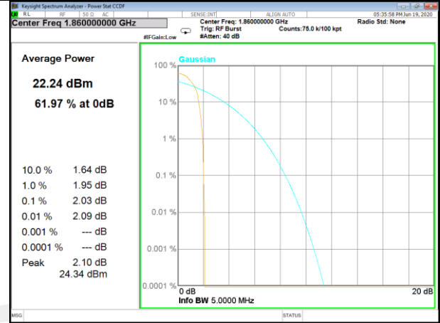
Band25-20M-16QAM-FULL RB-M
