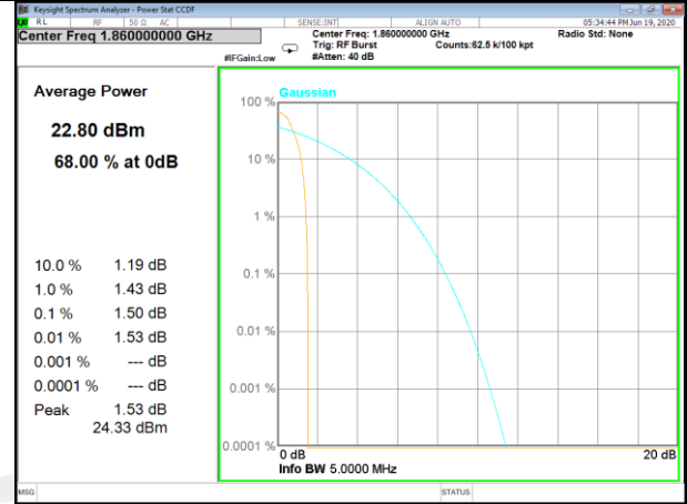
Band25-20M-QPSK-FULL RB-M
