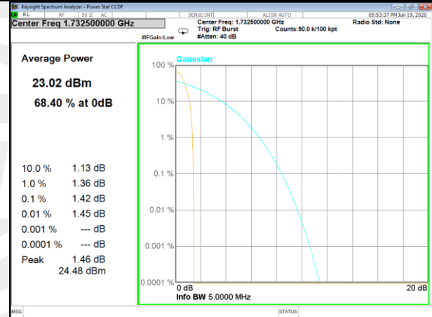
Band4-20M-QPSK-FULL RB-H
