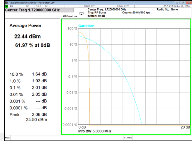
Band4-20M-16QAM-FULL RB-M
