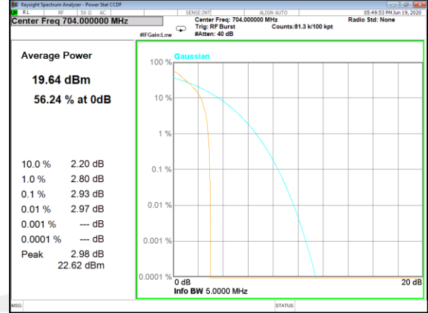
Band12-10M-QPSK-FULL RB-M
