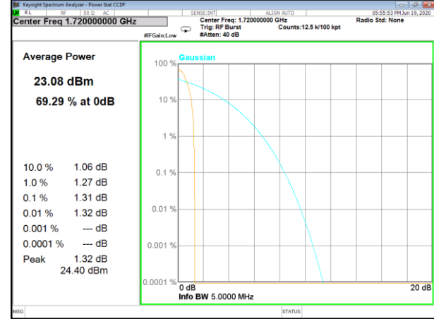
Band4-20M-QPSK-1 RB-M
