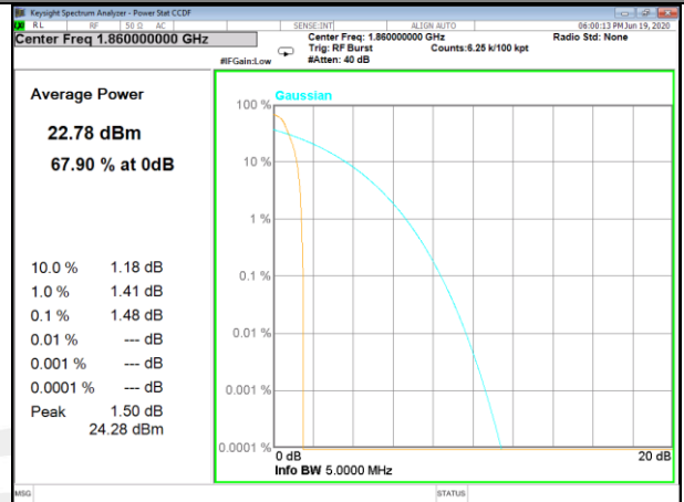
Band2-20M-QPSK-FULL RB-M
