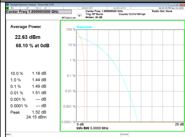
Band2-20M-QPSK-1 RB-H
