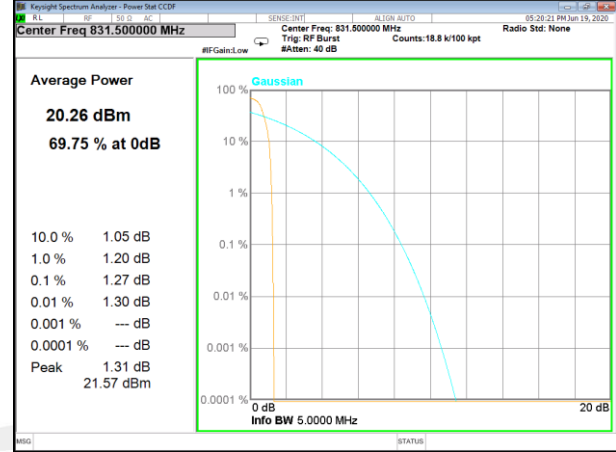
Band26-15M-QPSK-FULL RB-M
