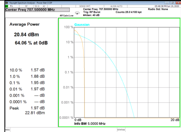
Band12-10M-QPSK-1 RB-H
