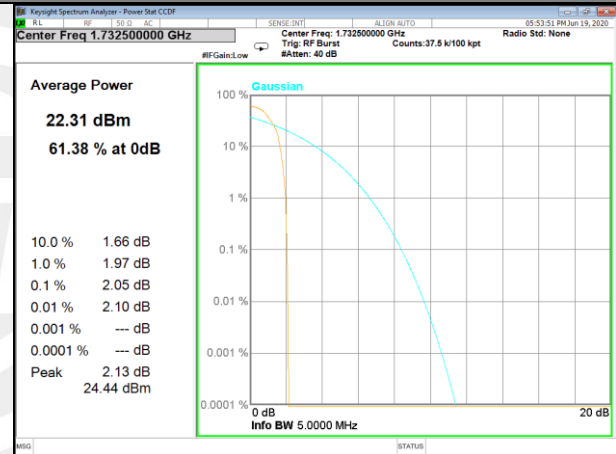
Band4-20M-16QAM-FULL RB-H
