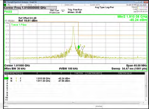
Band2 QPSK_20M_Higher_Full-RB
