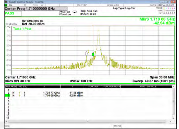
Band4 16QAM_15M_Lower_Full-RB
