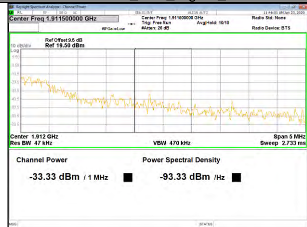
Band2 16QAM_20M_Lower_1-RB
