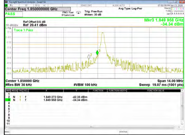
Band2 16QAM_3M_Lower_Full-RB
