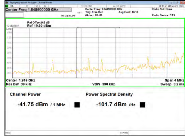
Band2 16QAM_15M_Lower_Full-RB
