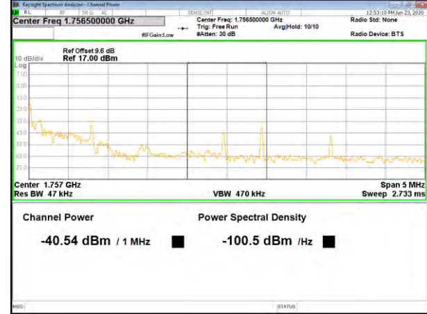
Band4 QPSK_20M_Higher_Full-RB
