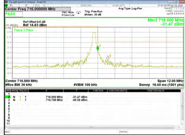
Band12_QAM16_1.4M_High_Full-RB
