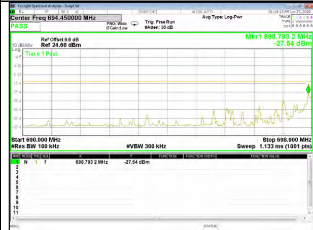
Band12_QAM16_1.4M_Low_Full-RB
