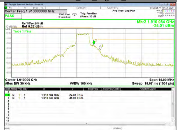
Band2 QPSK_3M_Higher_Full-RB
