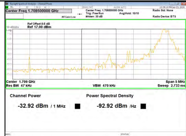
Band4 QPSK_3M_Lower_1-RB
