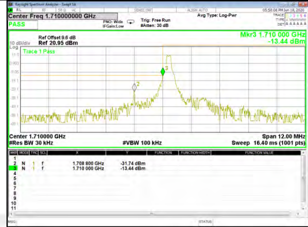
Band4 QPSK_1.4M_Lower_Full-RB
