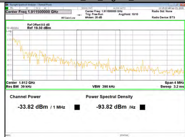
Band2 QPSK_3M_Higher_Full-RB
