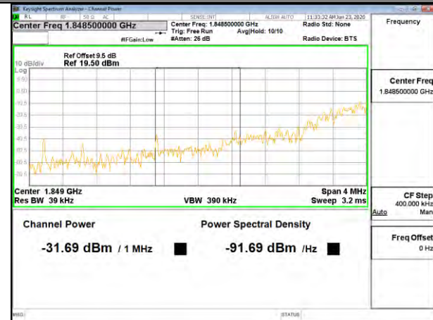
Band2 16QAM_10M_Lower_Full-RB
