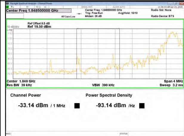
Band2_QPSK_1.4M_Low_Full-RB
