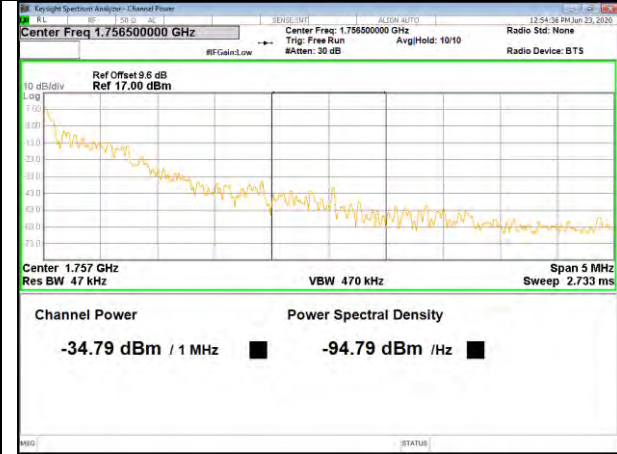
Band4 QPSK_20M_Lower_1-RB
