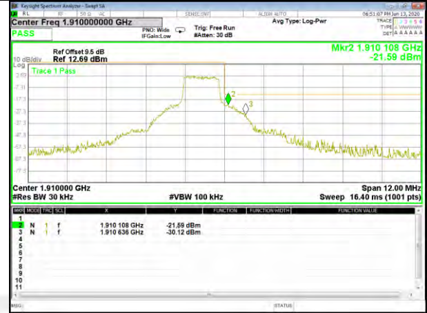
Band2_16QAM_1.4M_Low_1-RB
