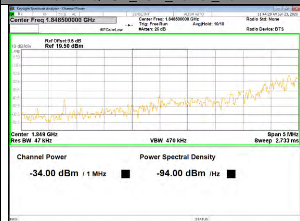
Band2 QPSK_20M_Lower_Full-RB
