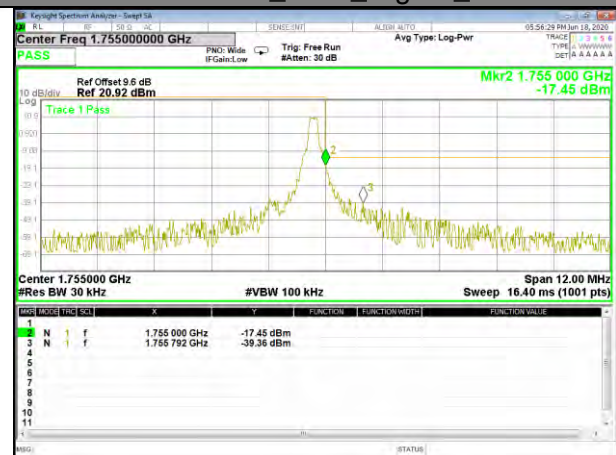
Band4 QPSK_1.4M_Higher_1-RB
