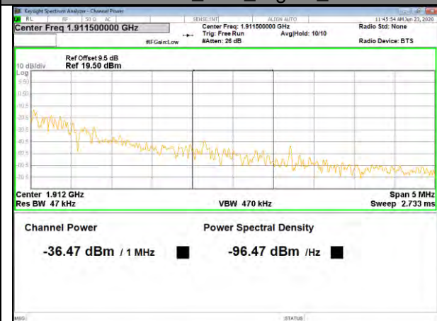
Band2 16QAM_20M_Higher_Full-RB
