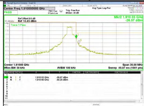
Band2 QPSK_15M_Higher_Full-RB
