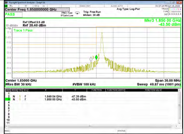
Band2 16QAM_15M_Lower_Full-RB
