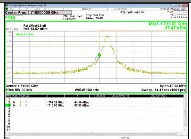
Band4 QPSK_20M_Lower_Full-RB
