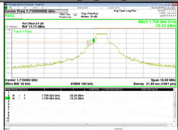
Band4 QPSK_5M_Lower_Full-RB
