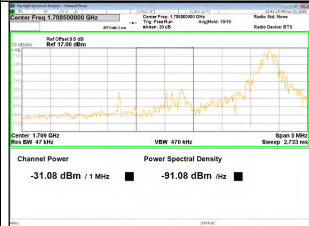
Band4 QPSK_5M_Lower_Full-RB
