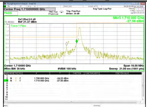
Band4 16QAM_5M_Lower_1-RB
