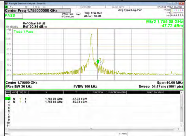
Band4 16QAM_20M_Higher_Full-RB
