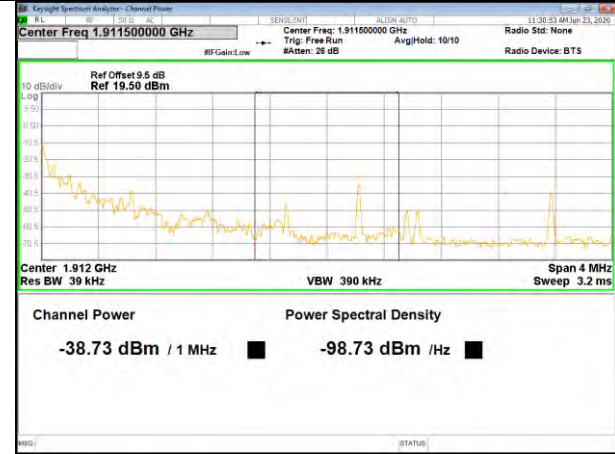
Band2_16QAM_10M_High_Full-RB
