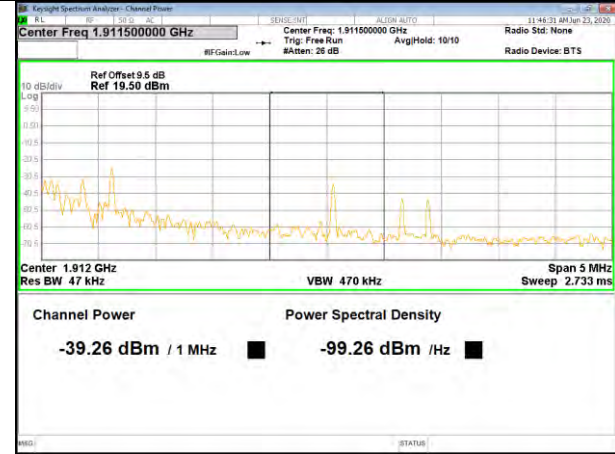
Band2 QPSK_20M_Higher_Full-RB
