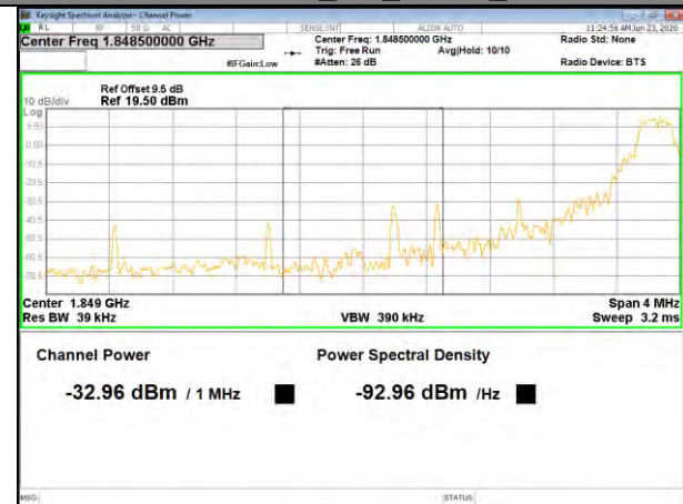
Band2 QPSK_5M_Lower_Full-RB
