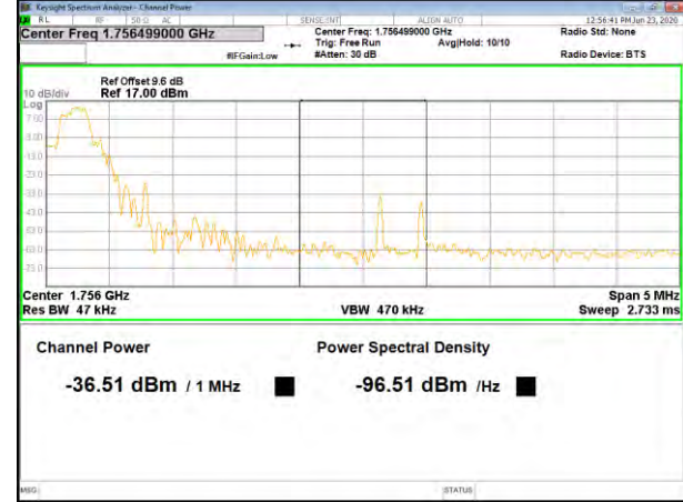
Band4 16QAM_10M_Higher_Full-RB
