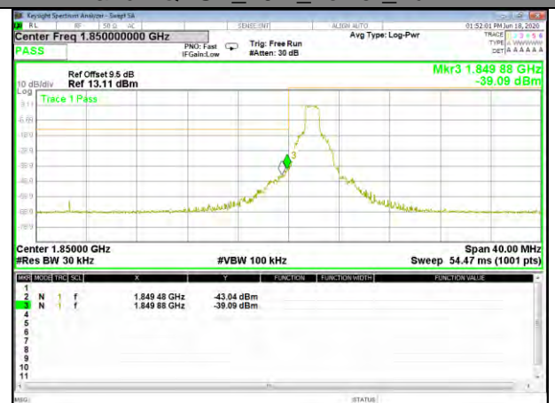
Band2 QPSK_20M_Lower_Full-RB
