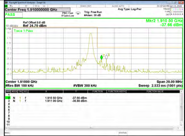
Band2_16QAM_10M_High_Full-RB
