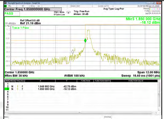
Band2_QPSK_1.4M_Low_Full-RB
