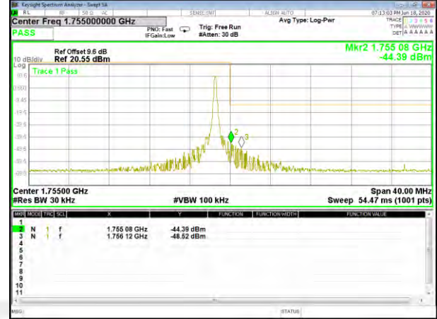
Band4 QPSK_20M_Higher_Full-RB
