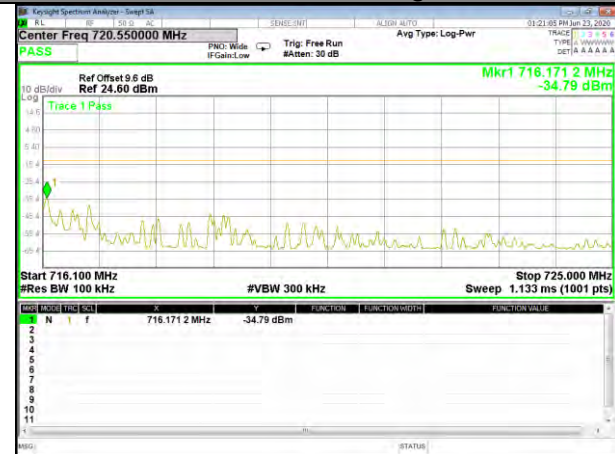
Band12_QPSK_3M_High_Full-RB
