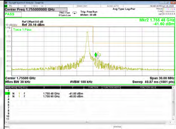
Band4 QPSK_15M_Higher_Full-RB
