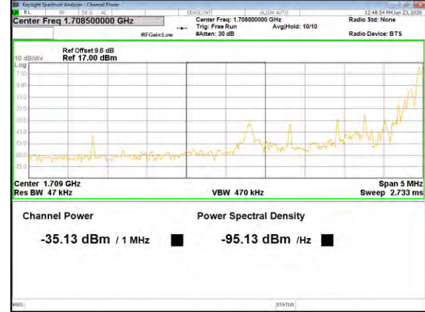
Band4 16QAM_15M_Lower_Full-RB
