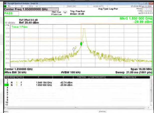
Band2 QPSK_5M_Lower_Full-RB
