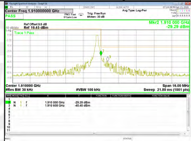
Band2 16QAM_5M_Higher_Full-RB
