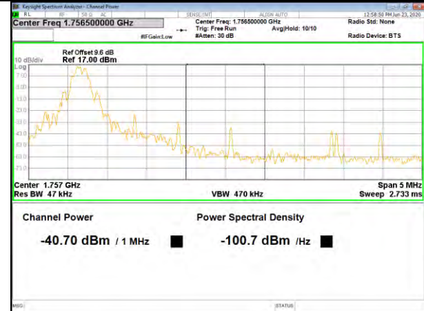
Band4 16QAM_5M_Higher_Full-RB
