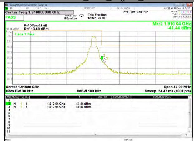
Band2 16QAM_20M_Higher_Full-RB
