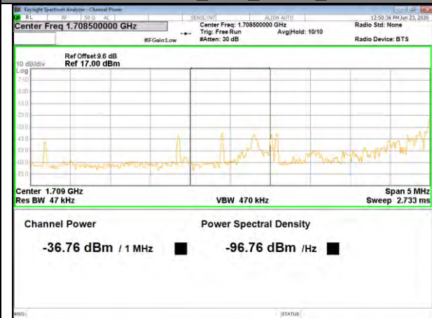
Band4 QPSK_20M_Lower_Full-RB
