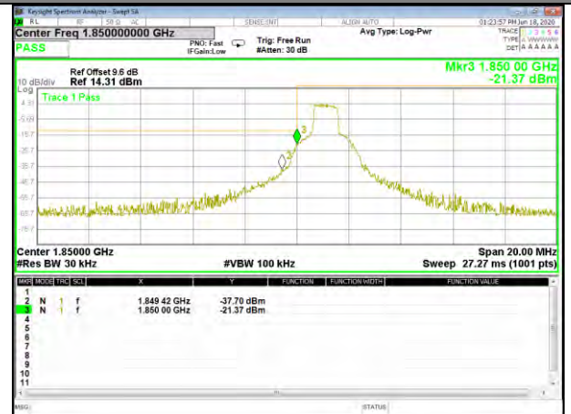
Band2 16QAM_10M_Lower_Full-RB
