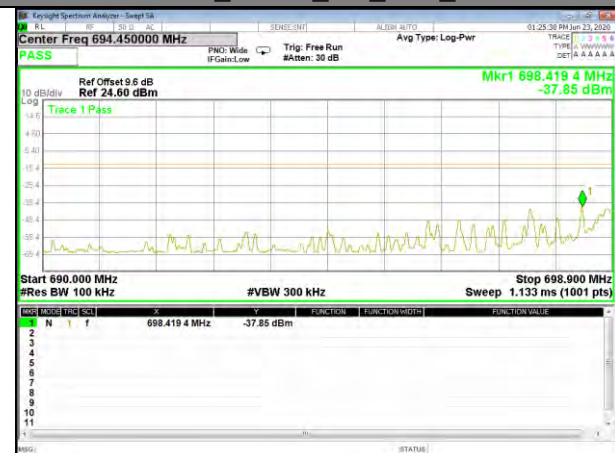
Band12_QPSK_3M_Low_1-RB
