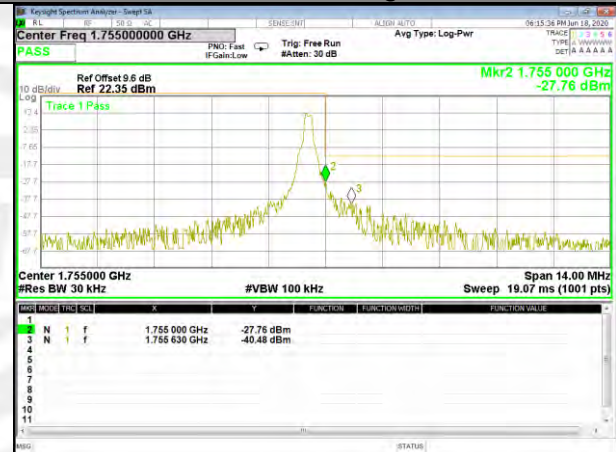
Band4 QPSK_3M_Higher_Full-RB
