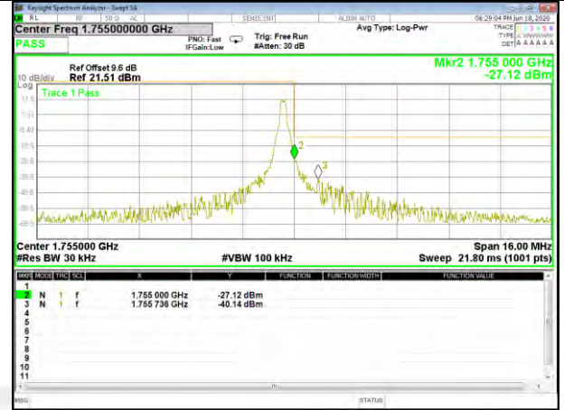
Band4 QPSK_5M_Higher_Full-RB
