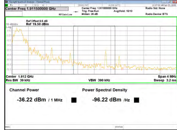
Band2 QPSK_5M_Higher_Full-RB
