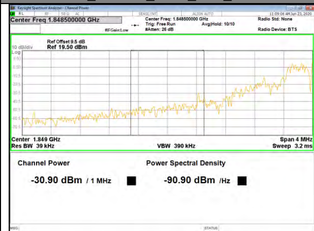
Band2_16QAM_1.4M_Low_Full-RB
