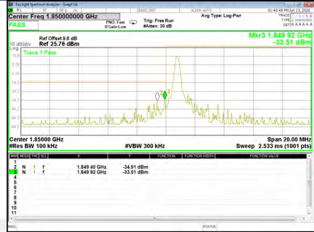
Band2_QPSK_10M_Low_Full-RB
