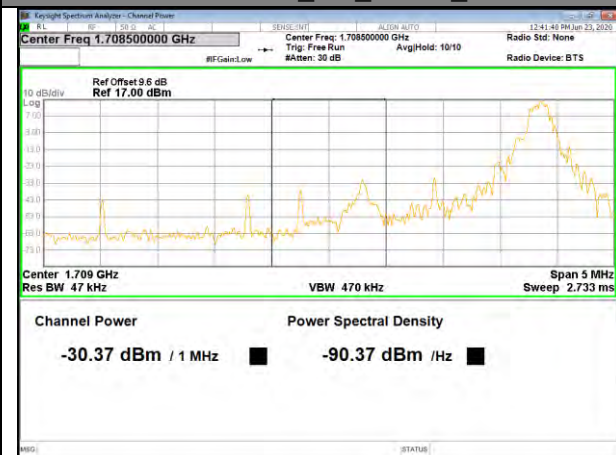
Band4 16QAM_5M_Lower_1-RB
