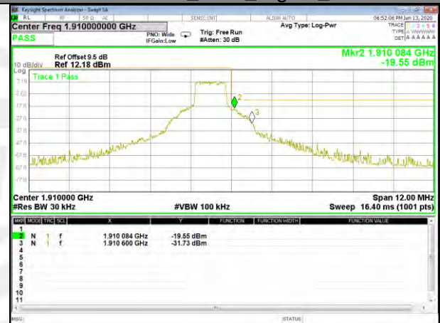
Band2 QPSK_3M_Lower_1-RB
