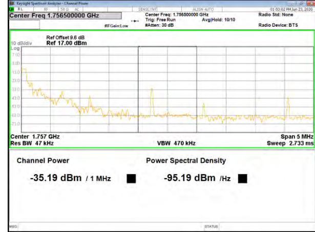
Band4 16QAM_1.4M_Higher_Full-RB
