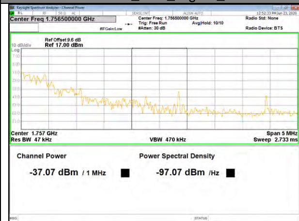
Band4 16QAM_20M_Higher_Full-RB
