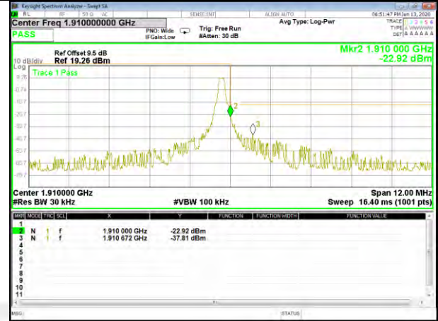
Band2 16QAM_1.4M_Higher_Full-RB
