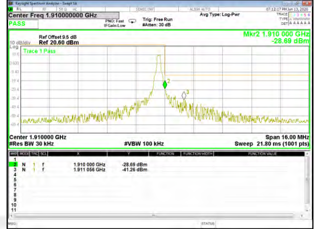
Band2 QPSK_5M_Higher_Full-RB
