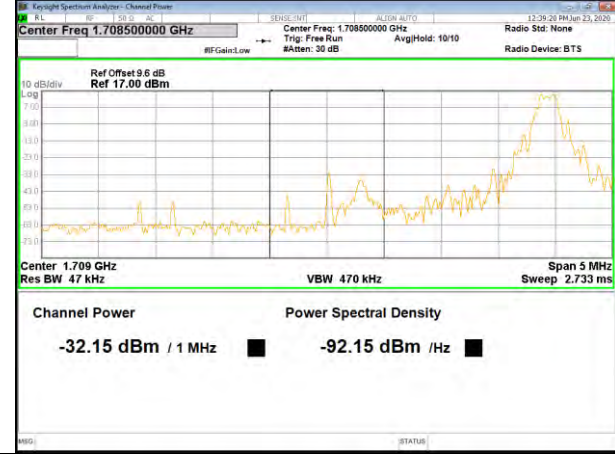
Band4 16QAM_3M_Lower_Full-RB
