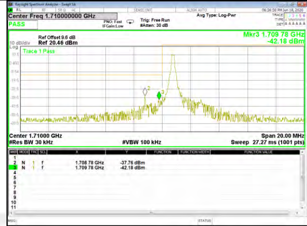
Band4 QPSK_10M_Lower_Full-RB
