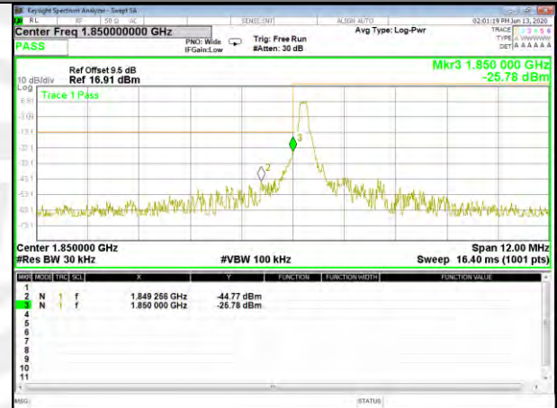
Band2_16QAM_1.4M_Low_Full-RB
