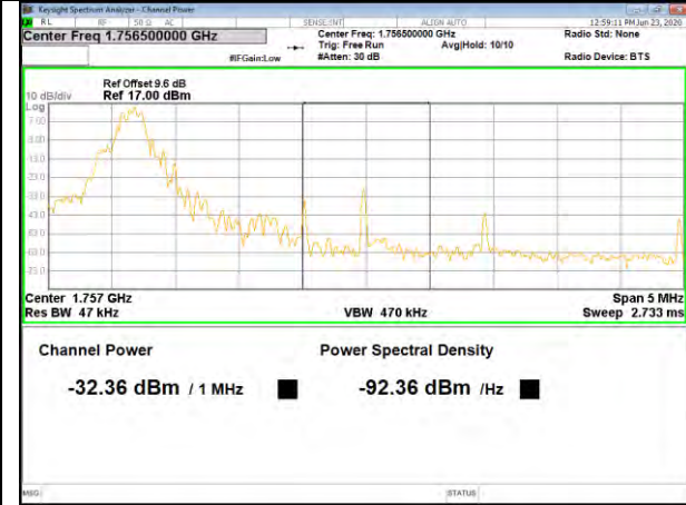
Band4 QPSK_5M_Higher_Full-RB
