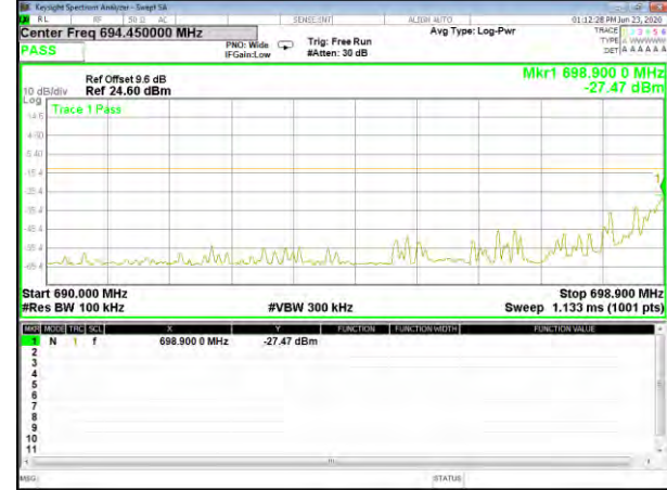
Band12_QPSK_1.4M_Low_Full-RB
