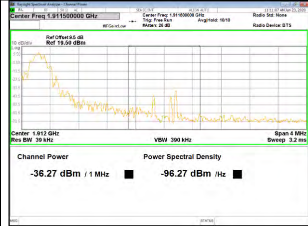
Band2 16QAM_1.4M_Higher_Full-RB
