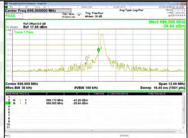
Band12_QAM16_1.4M_Low_Full-RB
