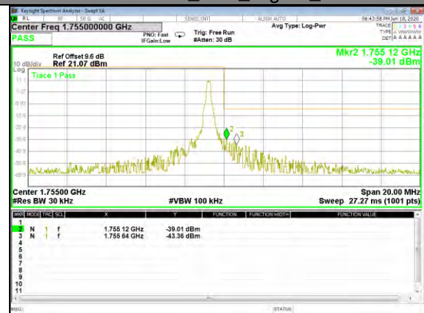
Band4 QPSK_10M_Higher_1-RB
