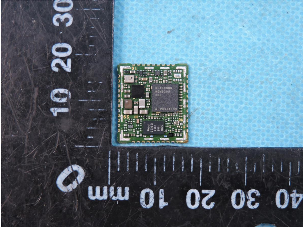
Photo 1(SIM7080G module)
