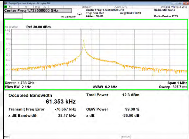
B4_3.75K_1#0_QPSK_Higher_(26BW and 99%)
