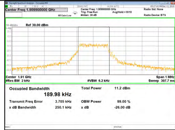
B2_15k_12#0_QPSK_Higher_(26BW and 99%)
