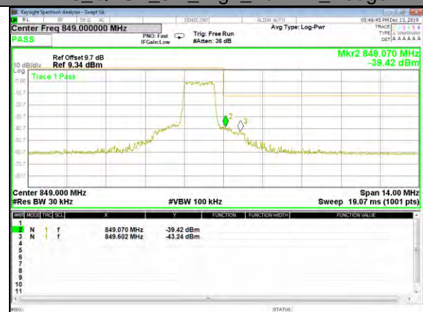
B26_QPSK_3M_High_Full-RB_Bedge
