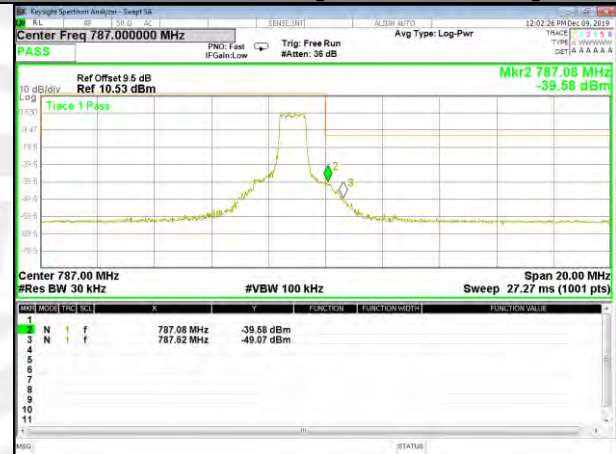
B13_Q16_10M_High_Full-RB_Bedge
