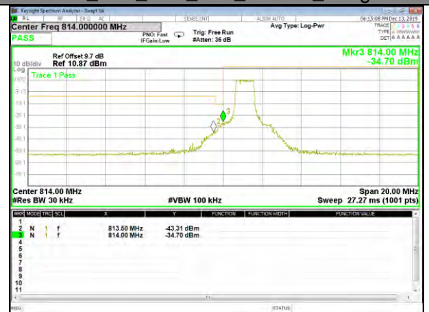
B26_Q16_10M_Low_Full-RB_Bedge
