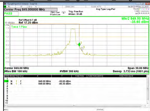
B26_Q16_15M_High_Full-RB_Bedge
