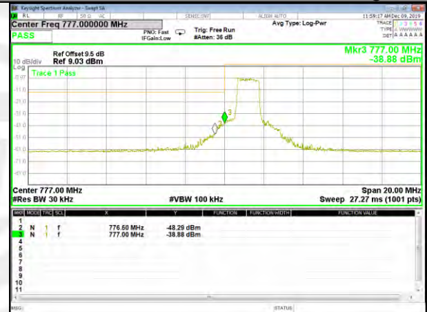
B13_QPSK_10M_High_Full-RB_Bedge
