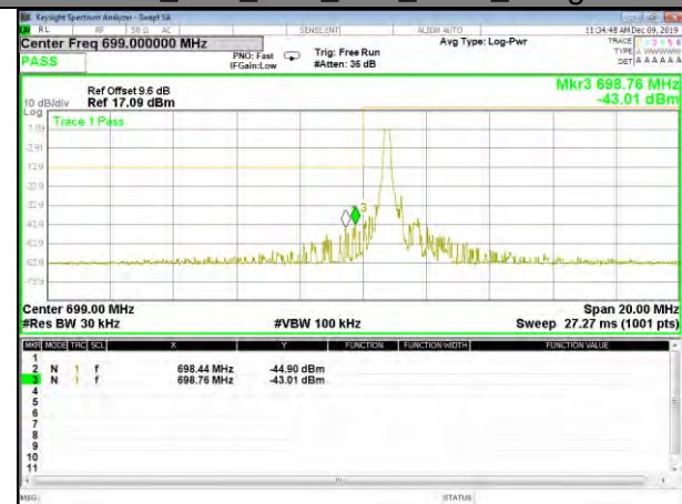
B12_Q16_10M_Low_1-RB_Bedge
