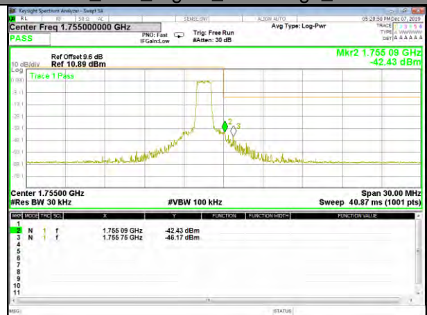
QPSK_15M_Higher_Band edge_Full-RB
