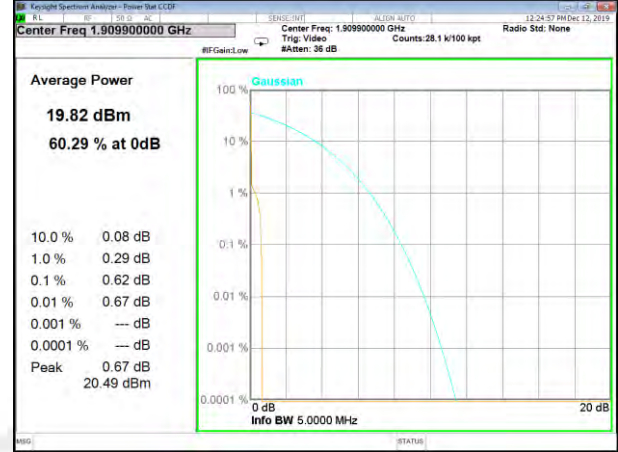
Band2_3.75k_1#0_BPSk_Higher
