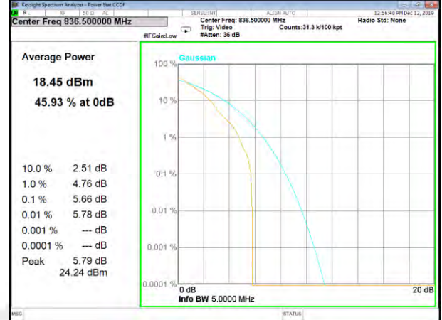
Band5_3.75k_1#0_QPSk_Middle
