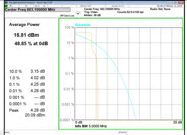
Band71_3.75k_1#0_BPSk_Lower
