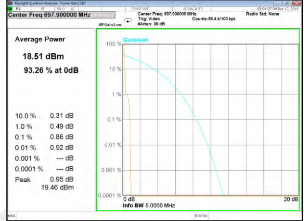
Band71_3.75k_1#0_BPSk_Higher
