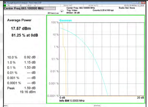
Band71_15k_1#0_BPSk_Middle
