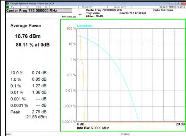
Band13_15k_1#0_BPSk_Higher
