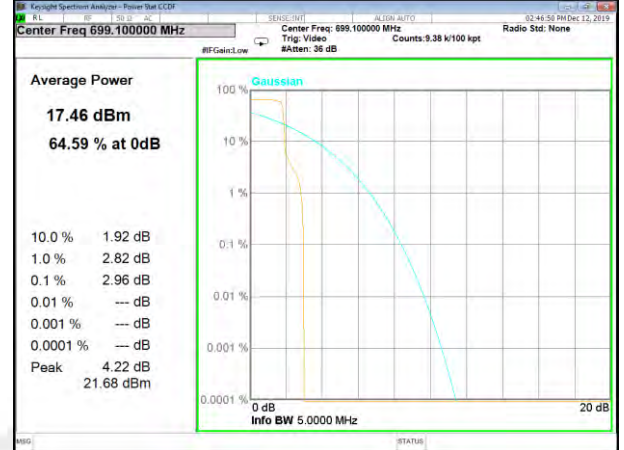
Band12_3.75k_1#0_BPSk_Lower
