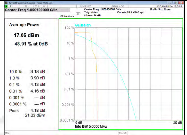
Band2_3.75k_1#0_BPSk_Lower
