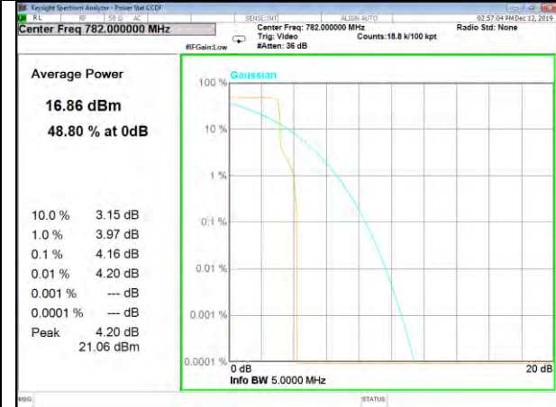
Band13_3.75k_1#0_BPSk_Middle
