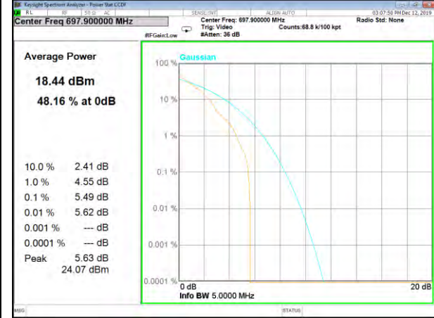
Band71_3.75k_1#0_QPSk_Higher
