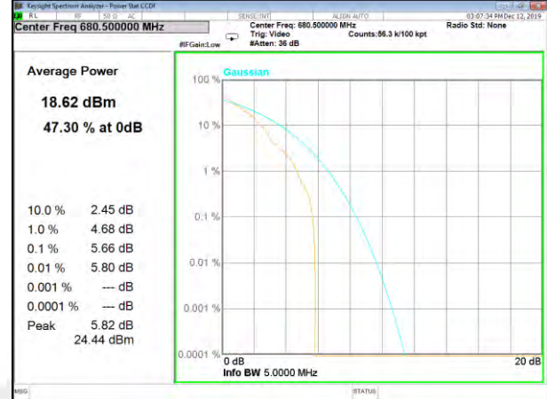
Band71_3.75k_1#0_QPSk_Middle
