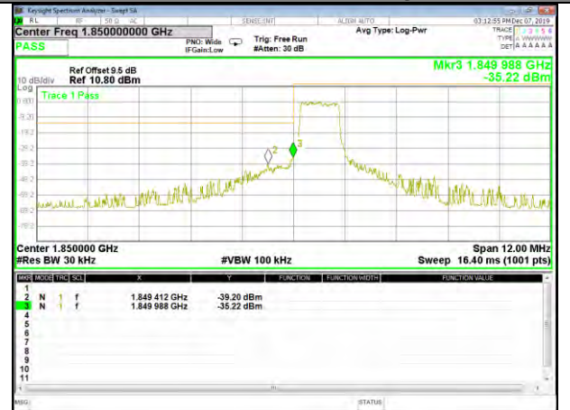
16QAM_1.4M_Lower_Band edge_Full-RB
