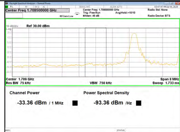
Band66_5M_QPSK_Low_Full-RB
