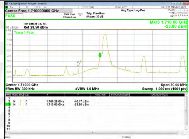
Band66_15M_QPSK_Low_Full-RB
