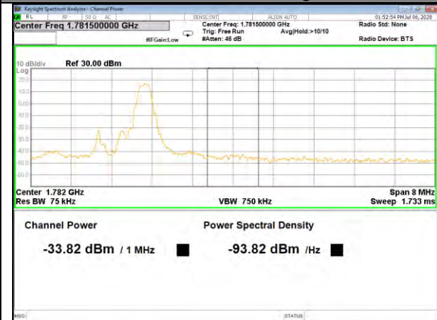
Band66_1.4M_QPSK_High_1-RB
