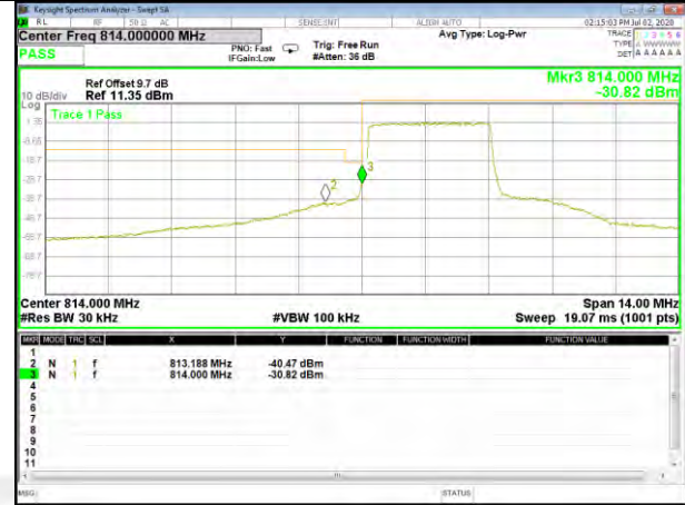
Band26_3M_16QAM_High_Full-RB
