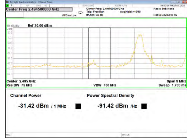
Band41_5M_QPSK_Low_Full-RB
