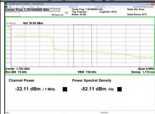
Band66_5M_16QAM_High_Full-RB
