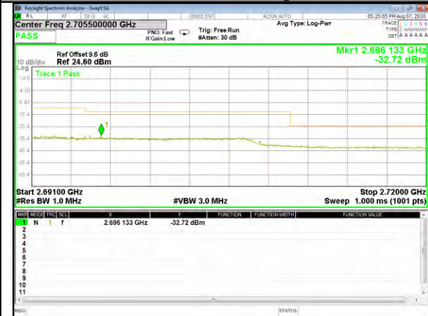
Band41_20M_QPSK_High_Full-RB
