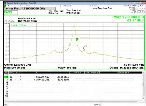
Band66_1.4M_QPSK_High_1-RB
