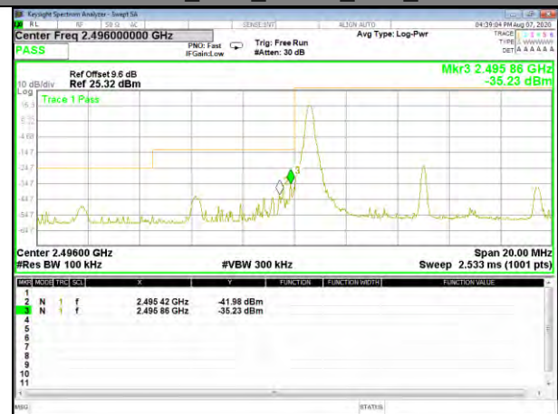
Band41_10M_QPSK_Low_1-RB
