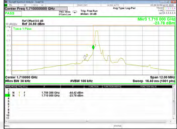
Band66_1.4M_QPSK_Low_Full-RB
