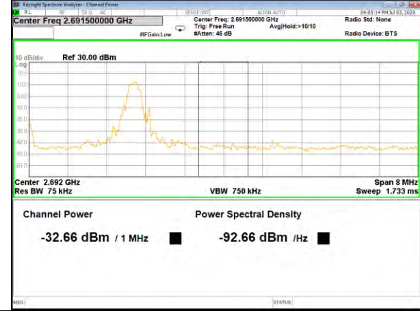
Band41_5M_16QAM_High_Full-RB
