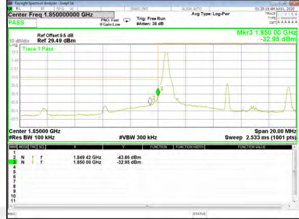
Band25_10M_QPSK_Low_Full-RB
