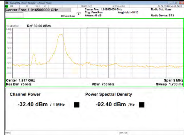
Band25_3M_QPSK_High_Full-RB
