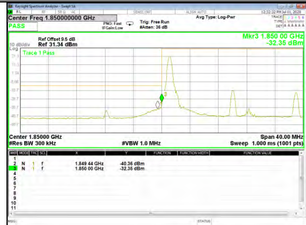
Band25_20M_QPSK_Low_1-RB
