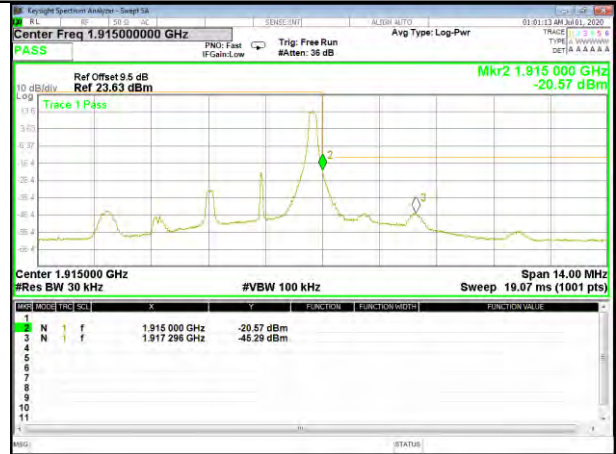
Band25_3M_16QAM_High_1-RB
