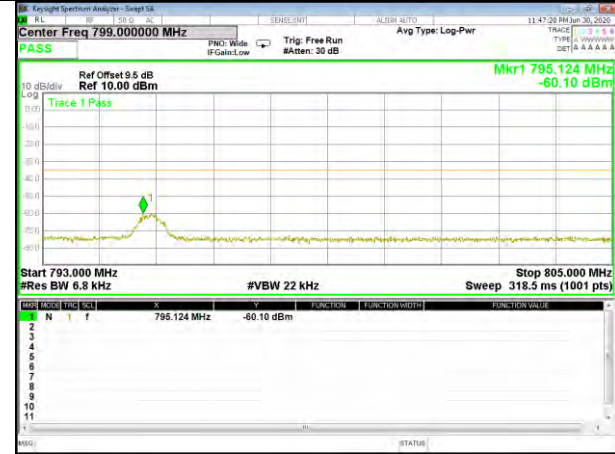
Band13_5M_16QAM_High_Full-RB
