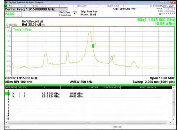
Band25_5M_QPSK_High_Full-RB
