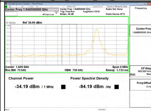
Band25_5M_16QAM_Low_1-RB
