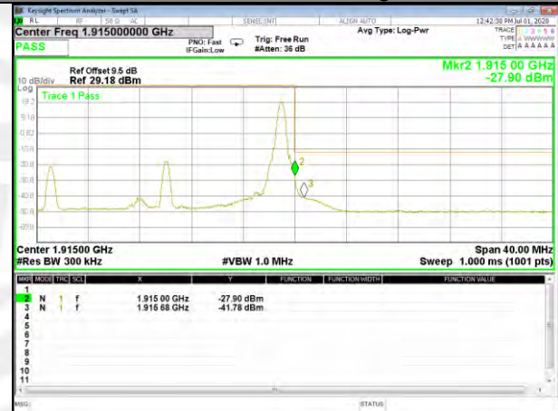
Band25_20M_QPSK_High_Full-RB
