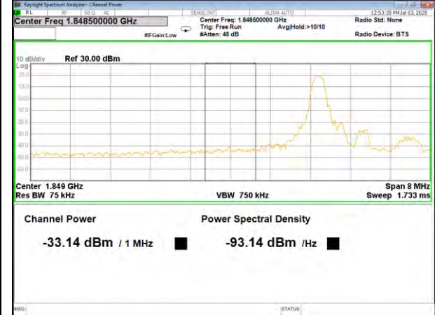
Band25_1.4M_QPSK_Low_Full-RB
