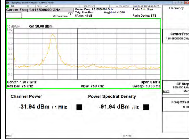
Band25_5M_QPSK_High_Full-RB
