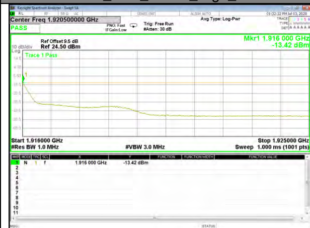
Band25_10M_QPSK_High_1-RB
