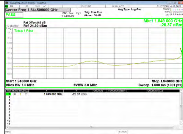
Band25_15M_QPSK_Low_Full-RB
