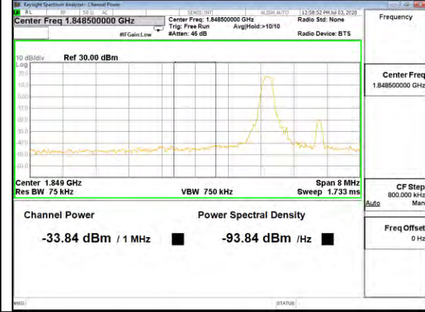
Band25_3M_16QAM_Low_Full-RB
