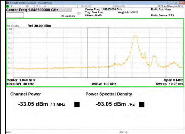
Band2_1.4M_16QAM_Low_Full-RB
