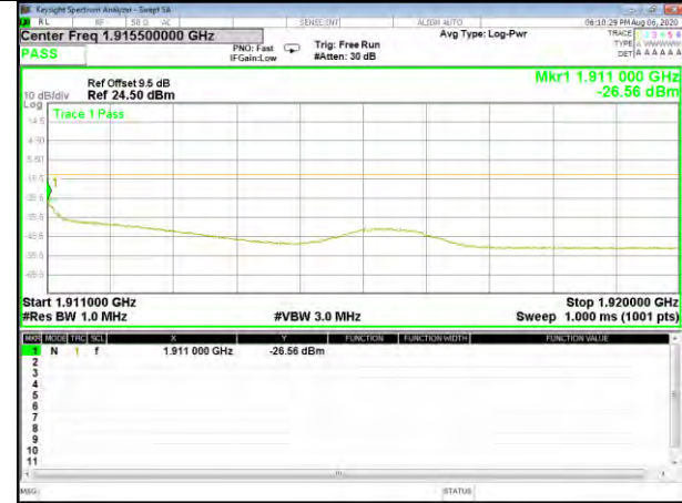
Band2_15M_QPSK_High_Full-RB
