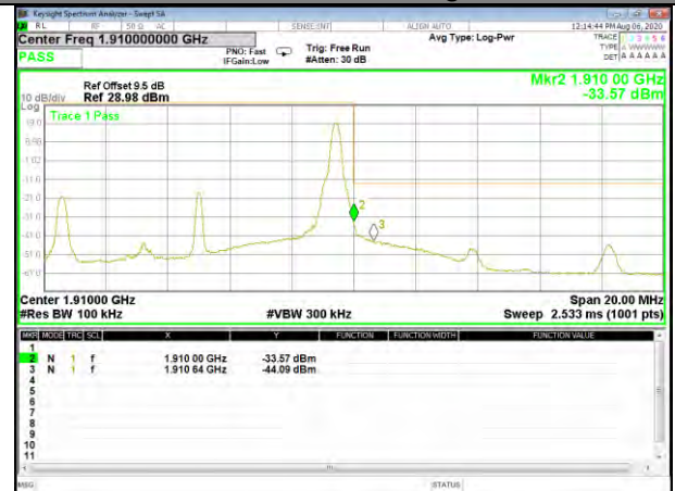
Band2_10M_QPSK_High_1-RB
