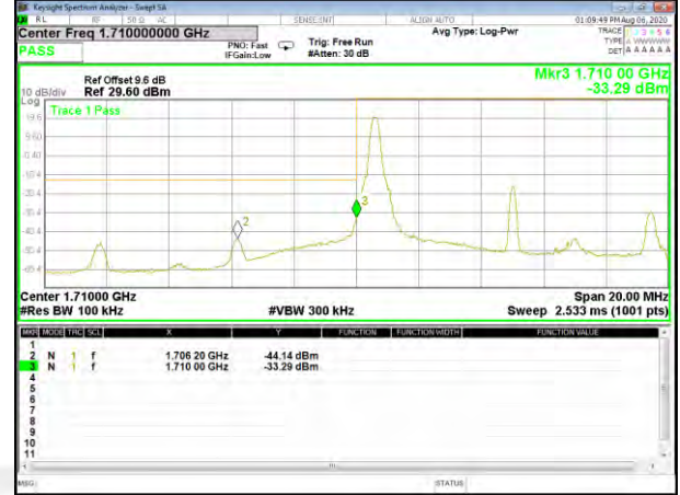
Band4_10M_QPSK_Low_Full-RB
