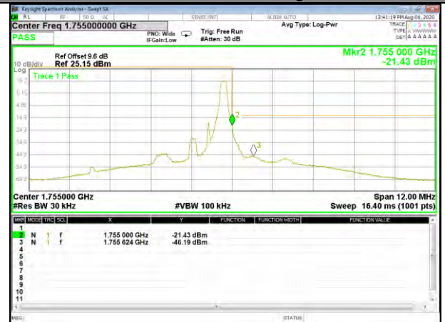
Band4_1.4M_QPSK_High_1-RB
