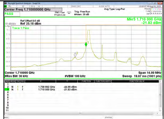
Band4_3M_QPSK_Low_1-RB
