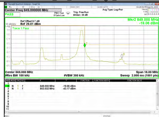
Band5_5M_QPSK_High_1-RB
