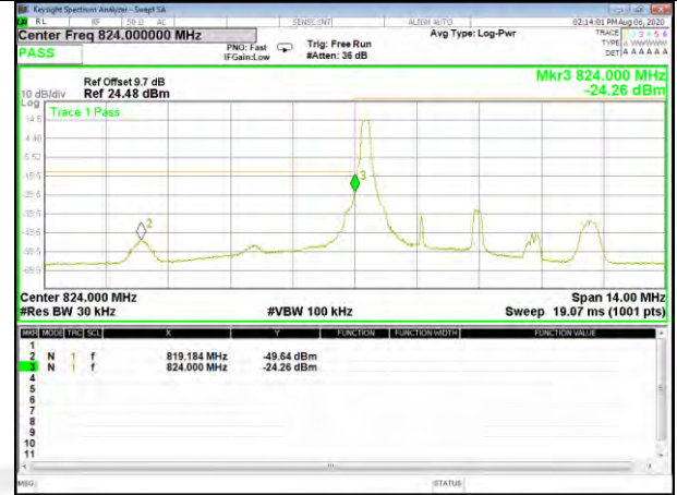
Band5_3M_16QAM_Low_Full-RB
