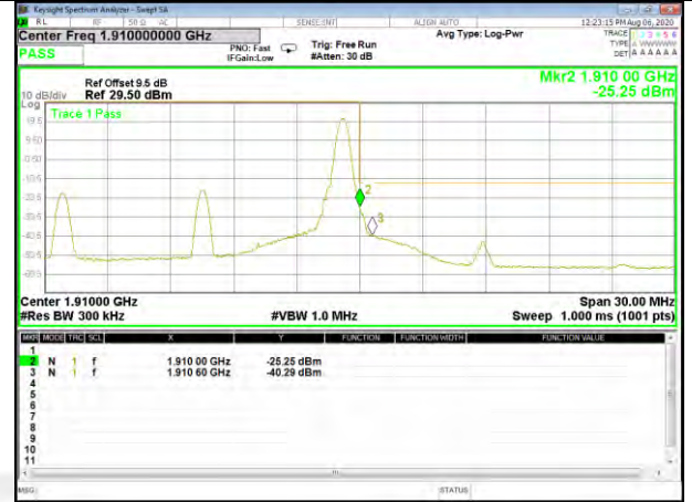
Band2_15M_QPSK_High_Full-RB
