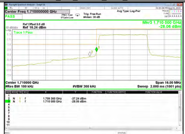
Band4_5M_QPSK_Low_Full-RB
