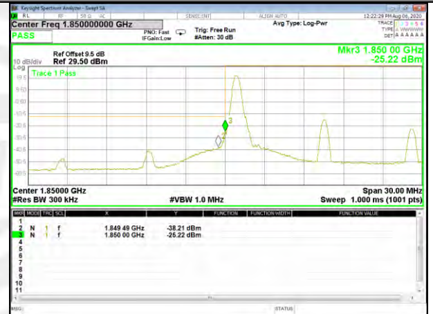
Band2_15M_QPSK_Low_Full-RB
