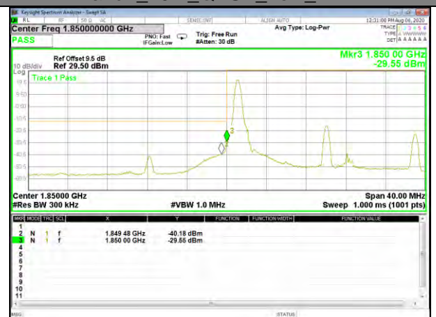
Band2_20M_QPSK_Low_1-RB
