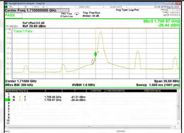
Band4_15M_QPSK_Low_Full-RB
