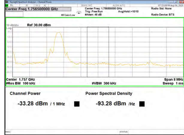
Band4_5M_QPSK_High_Full-RB
