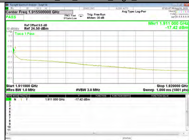
Band2_5M_16QAM_High_Full-RB
