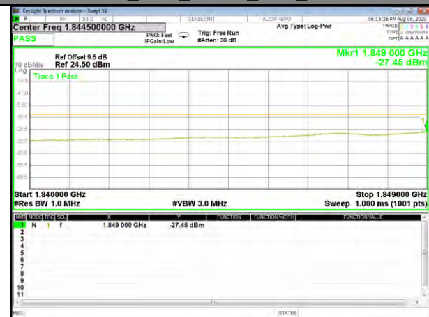
Band2_15M_QPSK_Low_Full-RB
