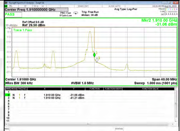
Band2_20M_QPSK_High_Full-RB
