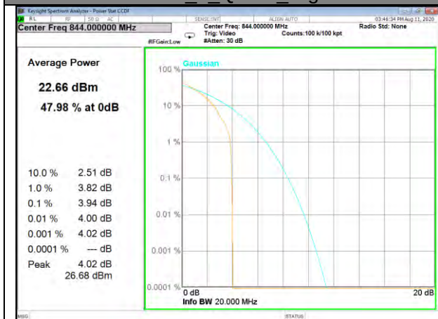
Band5_1_Q16_High
