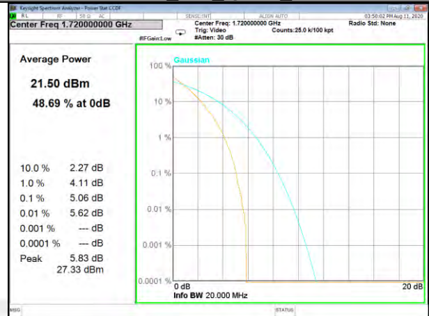
Band4_100_Q16_Low
