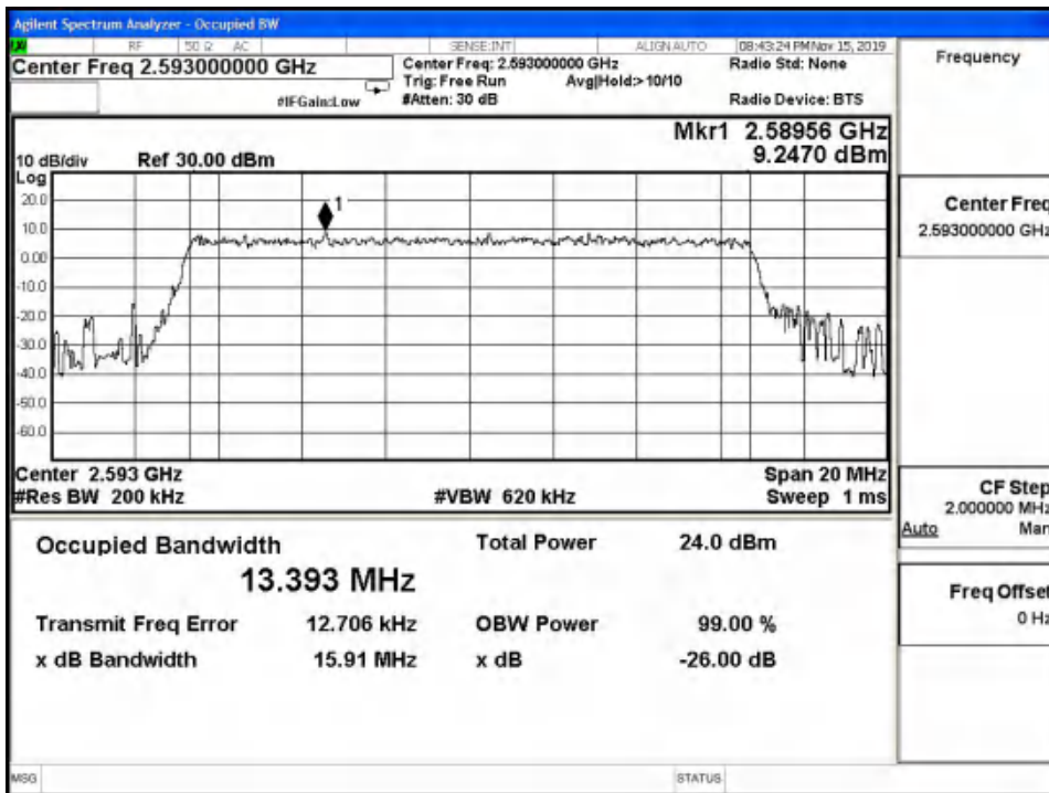
LTE Band41 16QAM -26dBc Channel 40620 BW=15MHz RB=75 RB Offset=0
