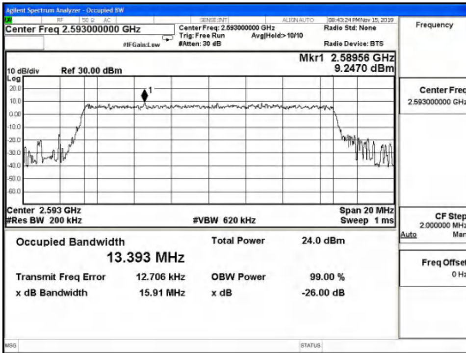
LTE Band41 16QAM 99% Channel 40620 BW=15MHz RB=75 RB Offset=0
