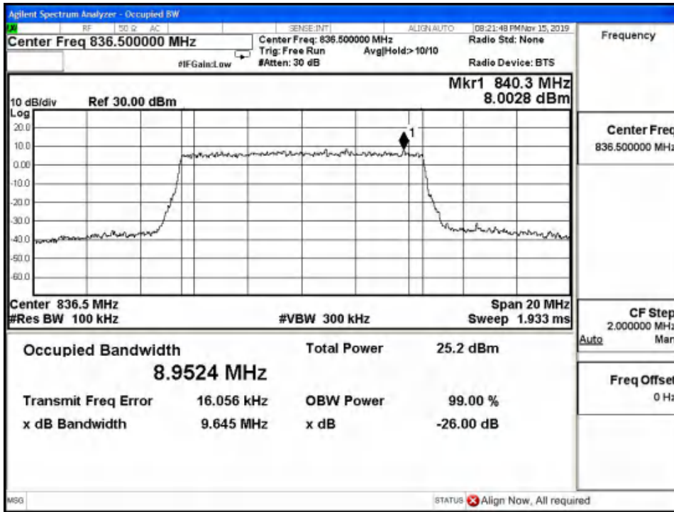
LTE Band26 16QAM 99% Channel 26915 BW=10MHz RB=50 RB Offset=0
