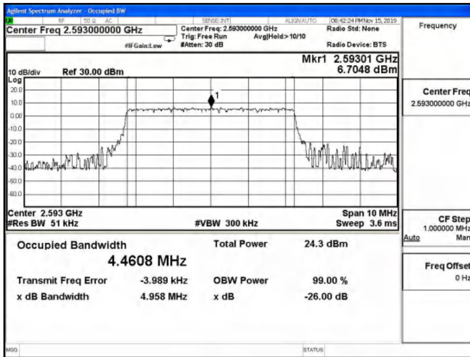
LTE Band41 QPSK -26dBc Channel 40620 BW=5MHz RB=25 RB Offset=0
