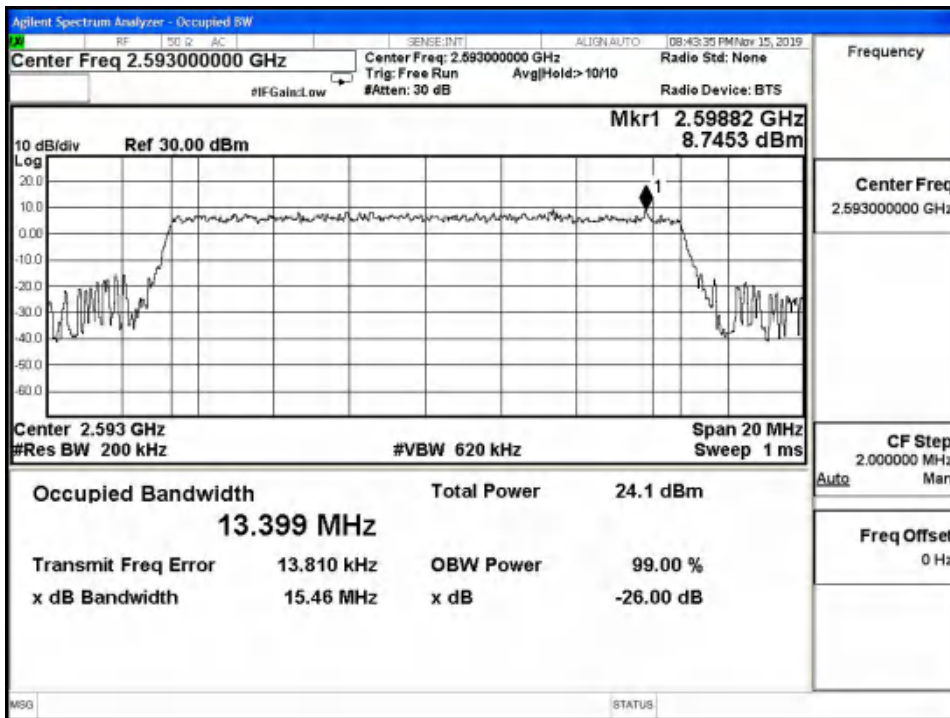
LTE Band41 QPSK -26dBc Channel 40620 BW=15MHz RB=75 RB Offset=0
