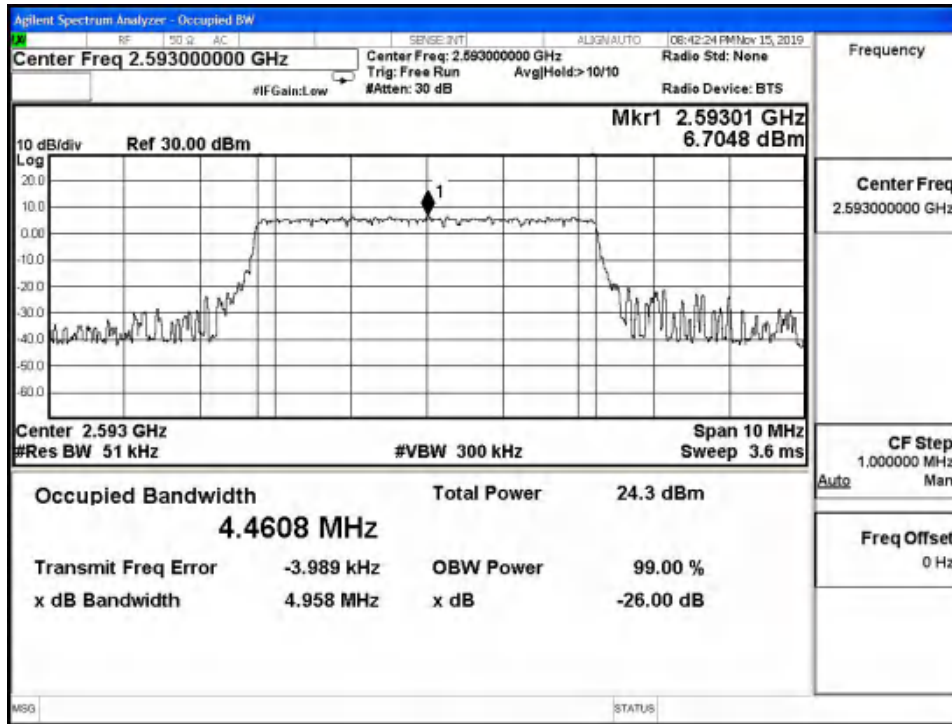
LTE Band41 QPSK 99% Channel 40620 BW=5MHz RB=25 RB Offset=0
