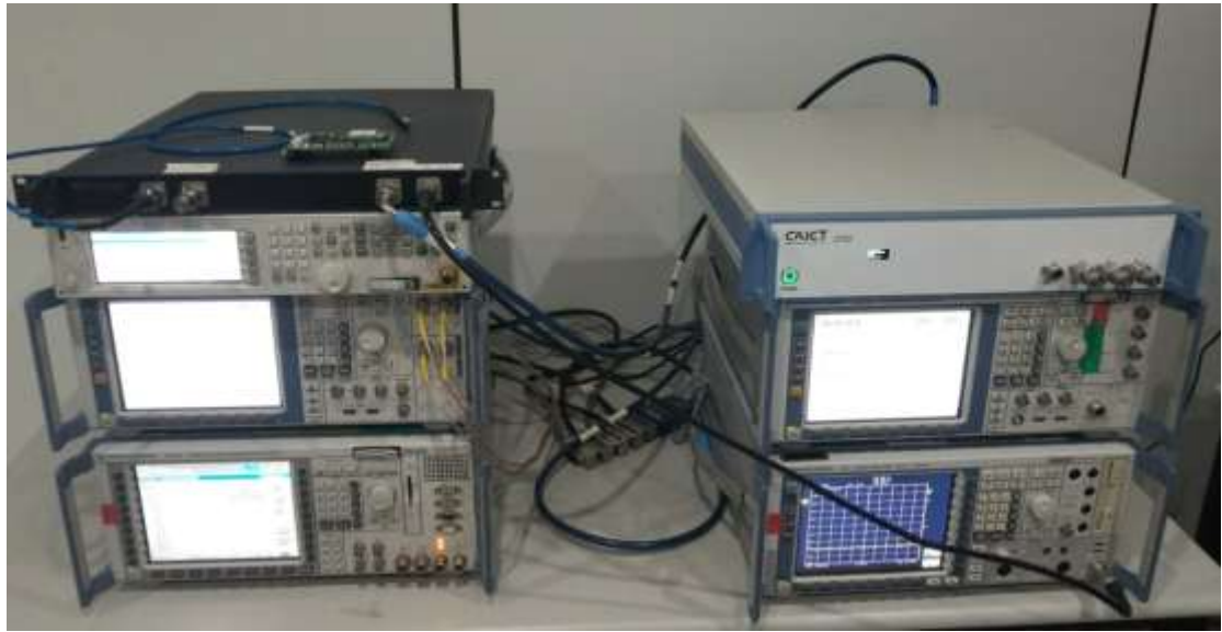
Test Setup Photo for RF test
