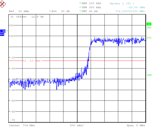
LOW BAND EDGE BLOCK-20MHz-100%RB
