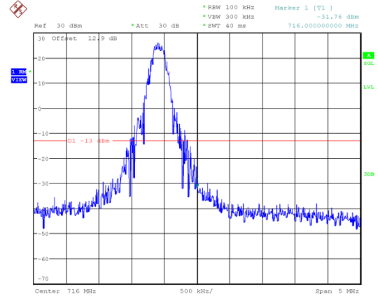
HIGH BAND EDGE BLOCK-1RB-high_offset
