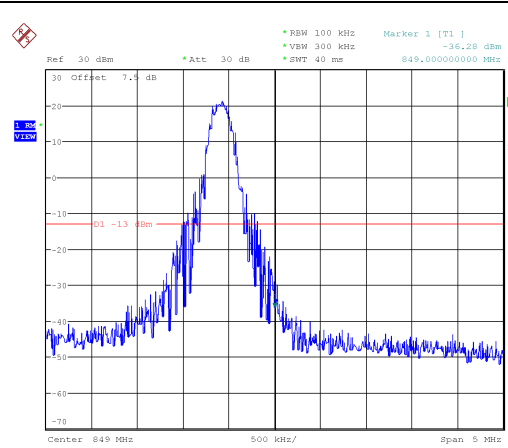
HIGH BAND EDGE BLOCK-1RB-high_offset
