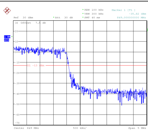
HIGH BAND EDGE BLOCK-20MHz-100%RB
