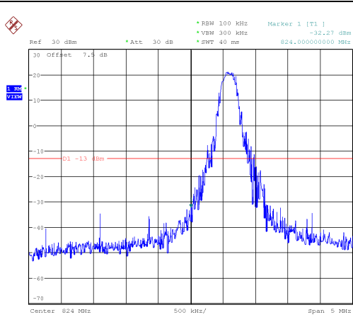
LOW BAND EDGE BLOCK-1RB-low_offset
