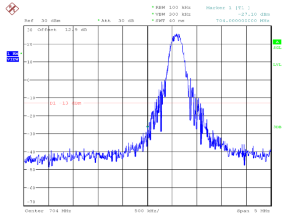
LOW BAND EDGE BLOCK-1RB-low_offset
