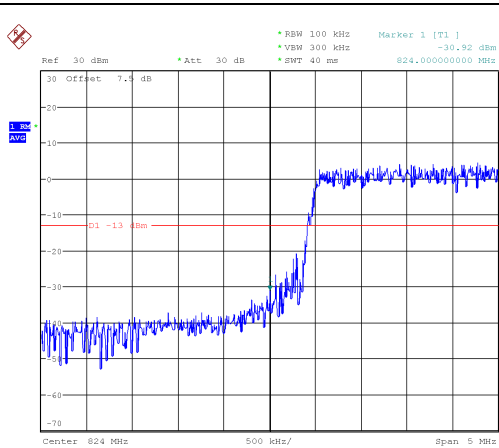
LOW BAND EDGE BLOCK-20MHz-100%RB
