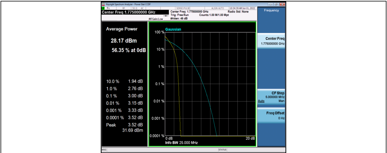
Band66-10MHz-16QAM-132022-50RB#0
