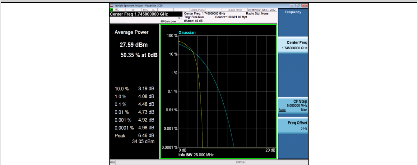
Band66-15MHz-16QAM-132597-75RB#0
