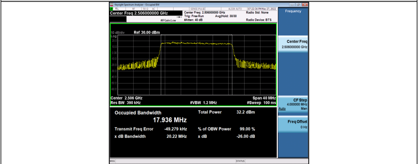
Band41-20MHz-16QAM-40620-100RB#0
