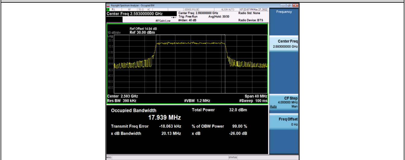
Band41-20MHz-16QAM-41490-100RB#0
