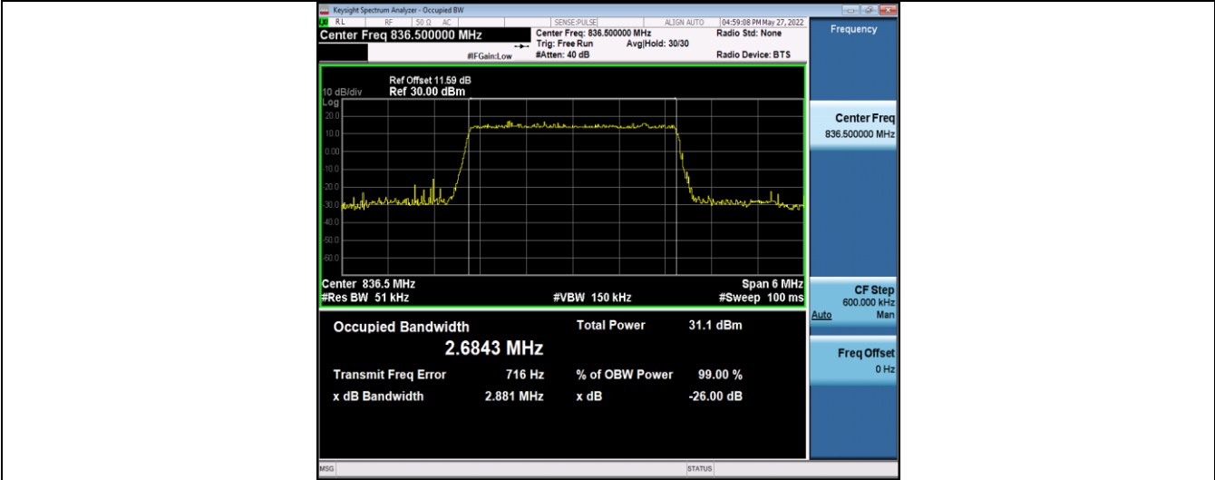
Band26-3MHz-16QAM-27025-15RB#0
