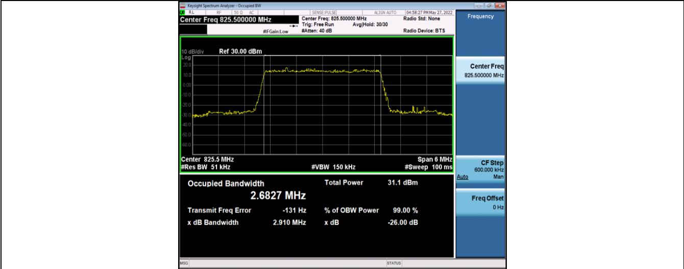
Band26-3MHz-16QAM-26915-15RB#0
