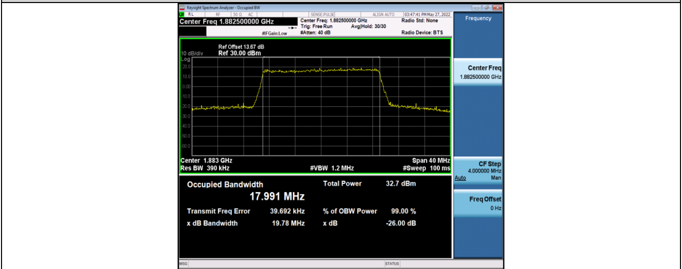
Band25-20MHz-16QAM-26590-100RB#0
