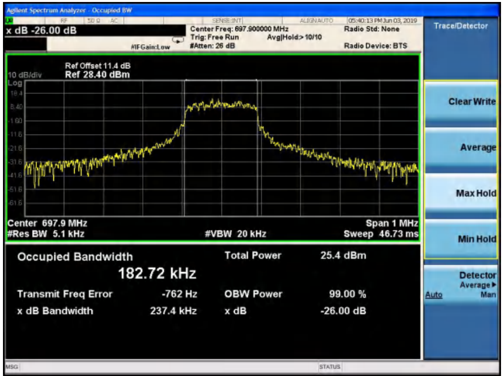
NB-IoT Guard-band band 71 133471 QPSK(26dB)
