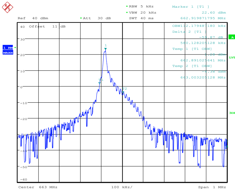
NB-IoT Guard-band band 71 133122 QPSK(99%)
