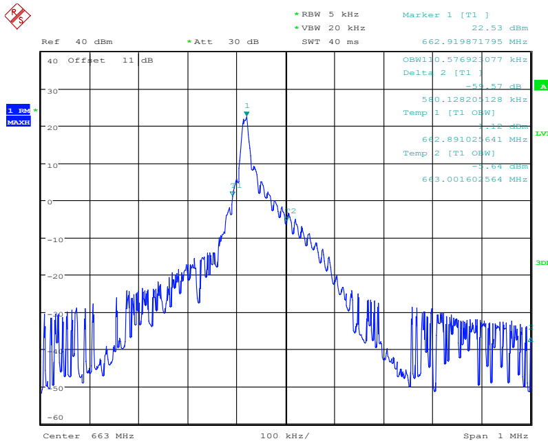
NB-IoT In-band band 71 133122 QPSK(99%)
