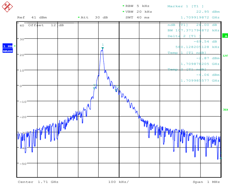
NB-IoT standalone band 66 131972 QPSK(26dB)
