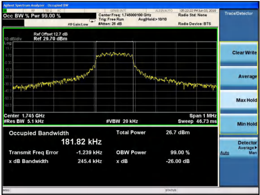
NB-IoT standalone band 66 132322QPSK(26dB)
