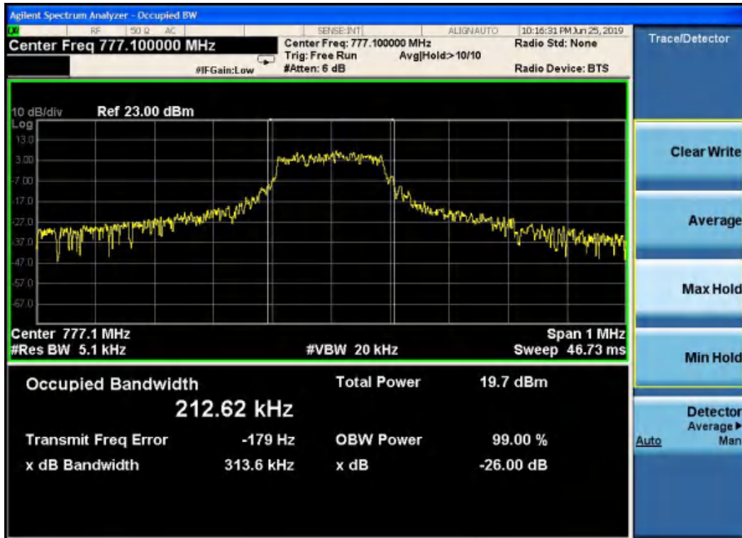
NB-IoT Guard-band band 13 23181 QPSK(99%)
