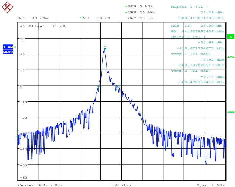
NB-IoT Guard-band band 71 133297 QPSK(26dB)
