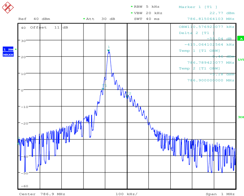
NB-IoT Guard-band band 13 23279 QPSK(99%)
