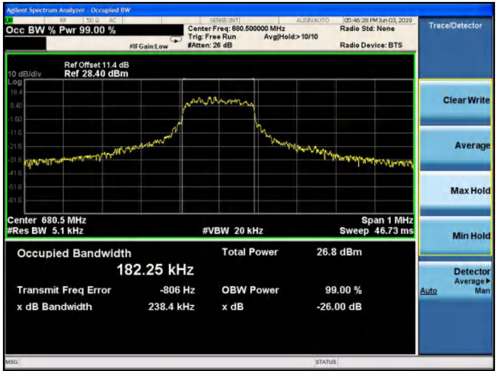
NB-IoT standalone band 71 133297 QPSK(99%)
