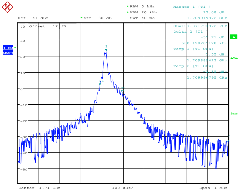
NB-IoT standalone band 66 131972 QPSK(99%)
