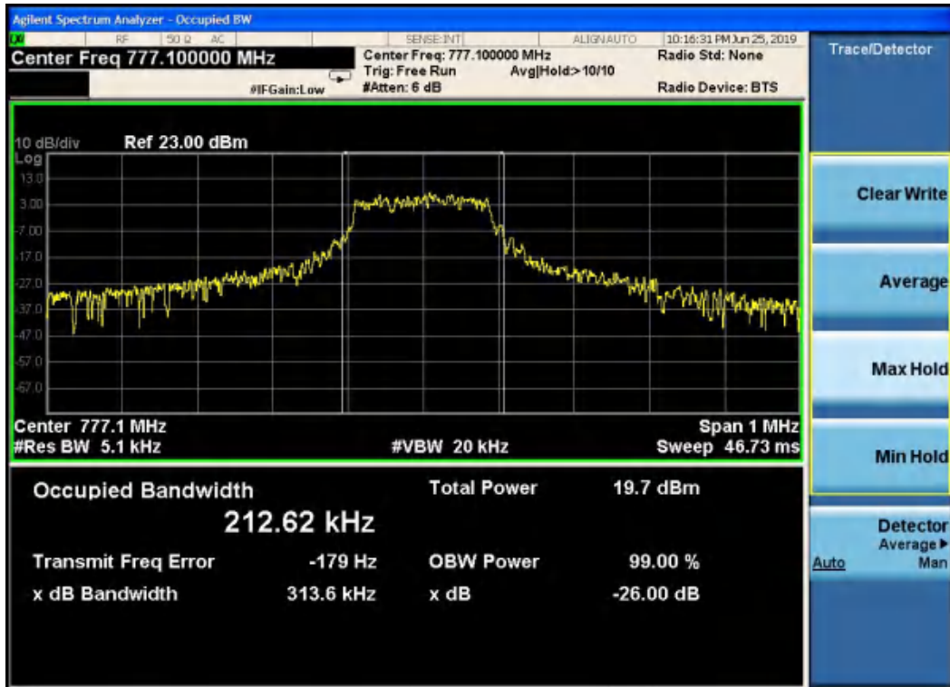
NB-IoT Guard-band band 13 23181 QPSK(26dB)
