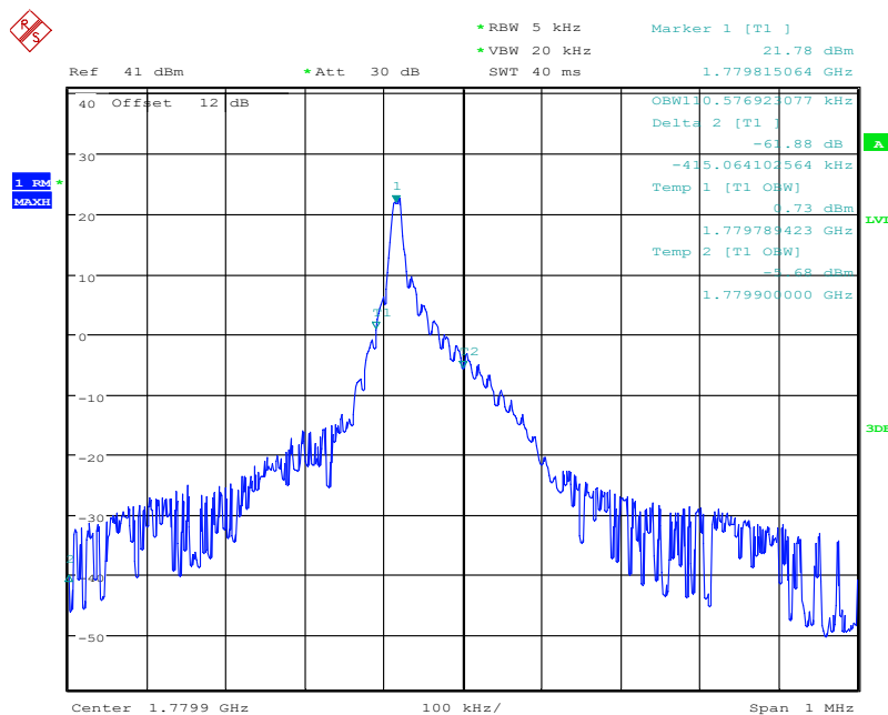
NB-IoT standalone band 66 132671 QPSK(99%)
