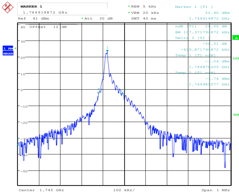
NB-IoT Guard-band band 66 132322 QPSK(26dB)
