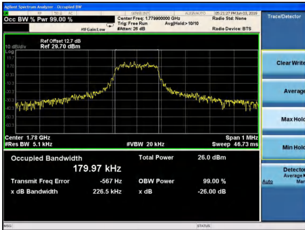
NB-IoT standalone band 66 132671 QPSK(99%)
