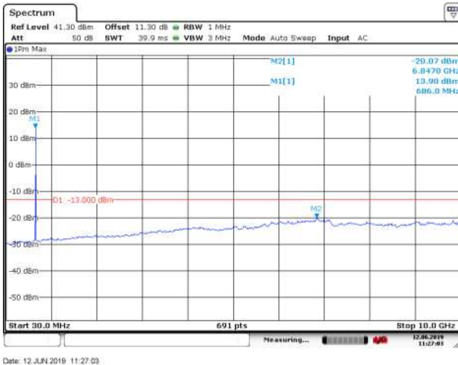
30MHz to 10GHz, Mid Channel, Subcarrier (15kHz), BPSK, 12@0 Note: The strong emission shown in each case is the carrier signal.
