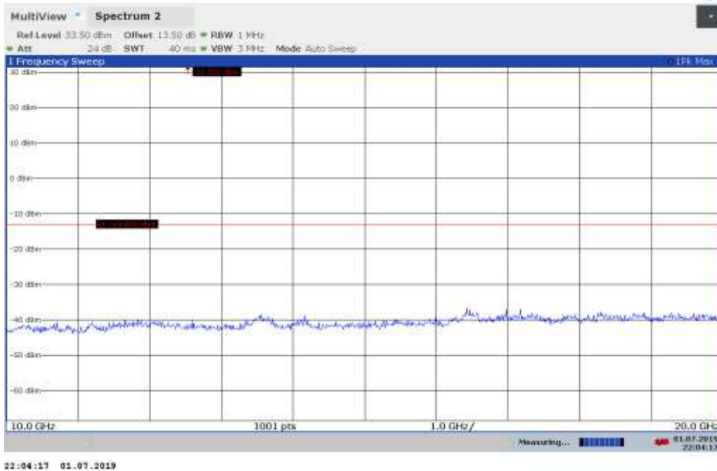
10GHz to 20GHz, High Channel, Subcarrier (3.75kHz), BPSK, 1@0
