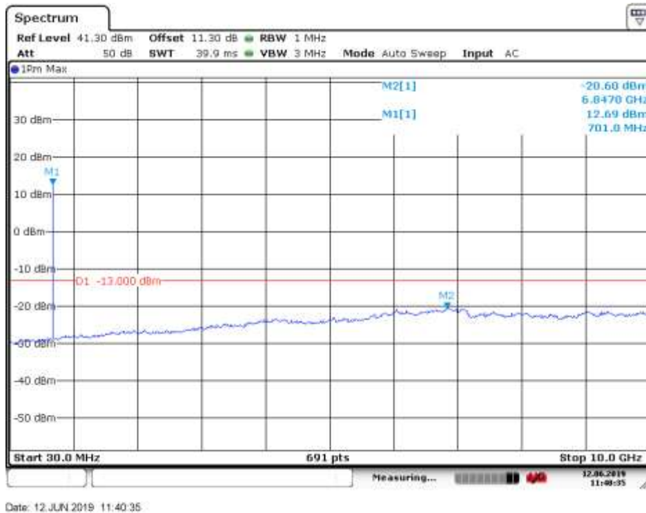
30MHz to 10GHz, High Channel, Subcarrier (15kHz), BPSK, 12@0 Note: The strong emission shown in each case is the carrier signal.
