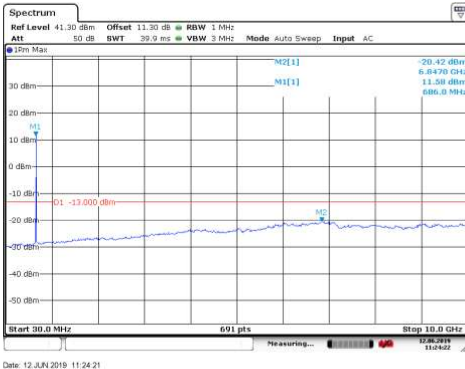
30MHz to 10GHz, Mid Channel, Subcarrier (15kHz), QPSK, 12@0 Note: The strong emission shown in each case is the carrier signal.
