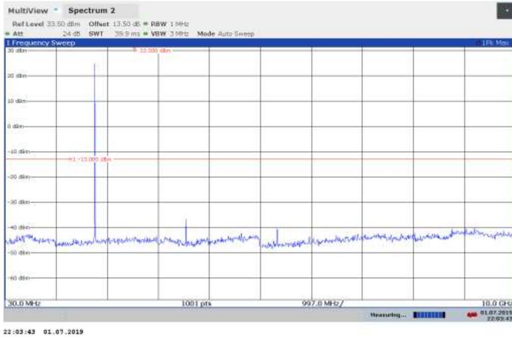
30MHz to 10GHz, High Channel, Subcarrier (3.75kHz), BPSK, 1@0 Note: The strong emission shown in each case is the carrier signal.
