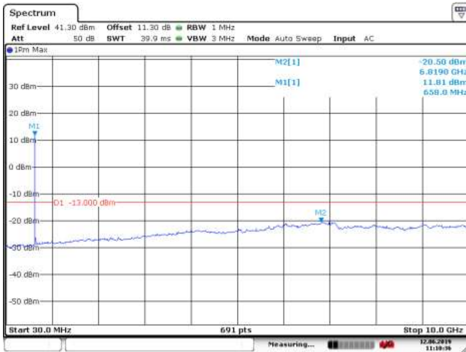
30MHz to 10GHz, Low Channel, Subcarrier (15kHz), BPSK, 1@0 Note: The strong emission shown in each case is the carrier signal.
