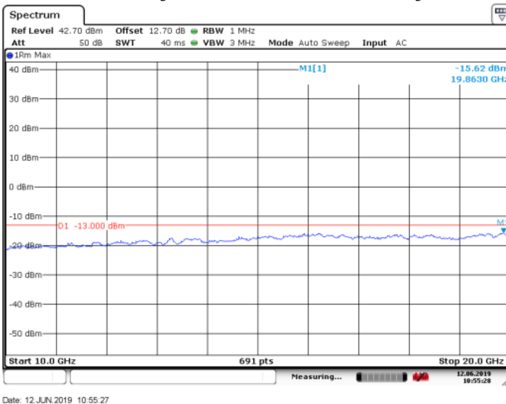
10GHz to 20GHz, High Channel, Subcarrier (15kHz), QPSK, 1@0
