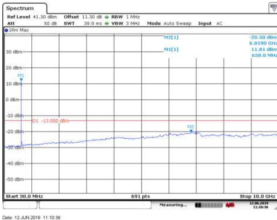
30MHz to 10GHz, Low Channel, Subcarrier (15kHz), BPSK, 12@0 Note: The strong emission shown in each case is the carrier signal.
