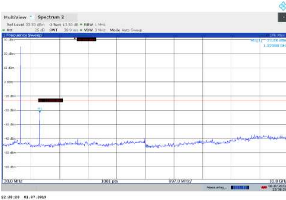
30MHz to 10GHz, Low Channel, Subcarrier (15kHz), BPSK, 1@0 Note: The strong emission shown in each case is the carrier signal.
