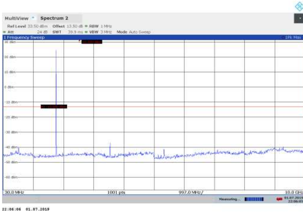
30MHz to 10GHz, High Channel, Subcarrier (15kHz), QPSK, 1@0 Note: The strong emission shown in each case is the carrier signal.
