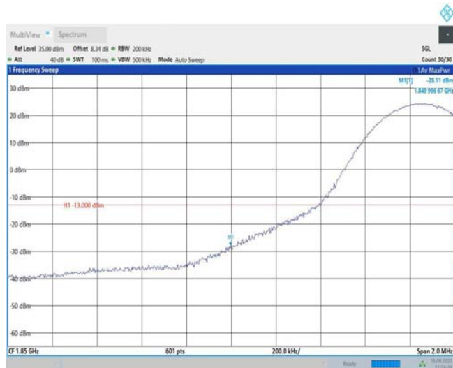
Band25-15MHz-16QAM-26115-1RB#74
