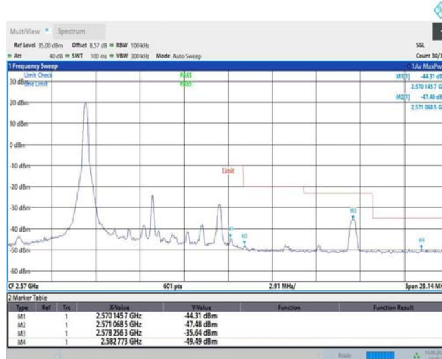
Band7-10MHz-QPSK-21400-1RB#49
