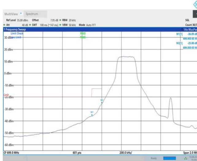
Band12-1.4MHz-QPSK-23017-1RB#5
