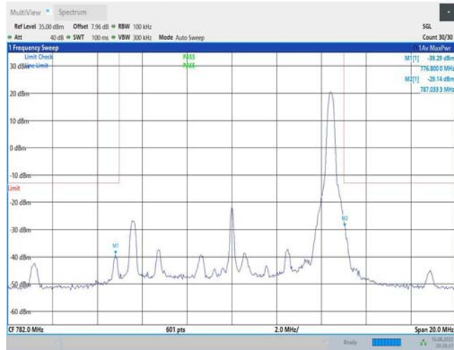
Band13-10MHz-QPSK-23230-50RB#0
