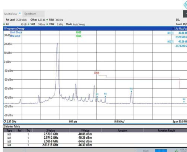
Band7-20MHz-16QAM-21350-1RB#99
