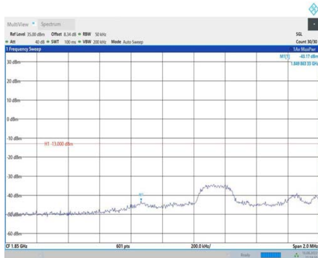
Band25-5MHz-QPSK-26065-25RB#0
