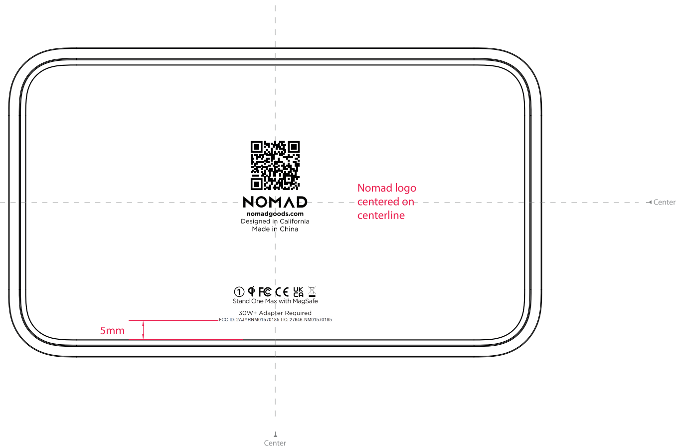
BOTTOM VIEW SCALE 1:1
