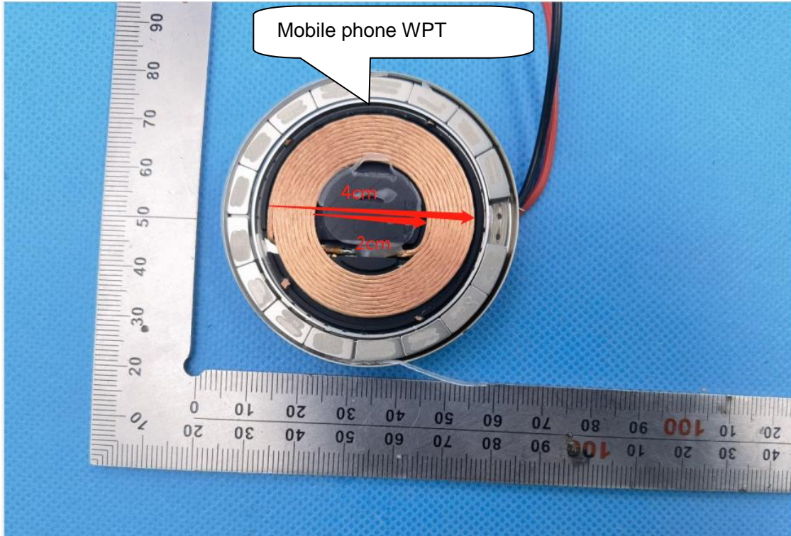
ANTENNA CLOSE-UP PHOTO-2
